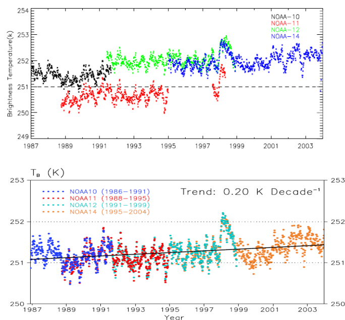
Figure 1. Global tropospheric temperature trends revealed by NOAA-10, -11, -12, and -14 Microwave Sounding Unit (MSU) data before (top) and after (bottom) intersatellite calibration bias correction.
