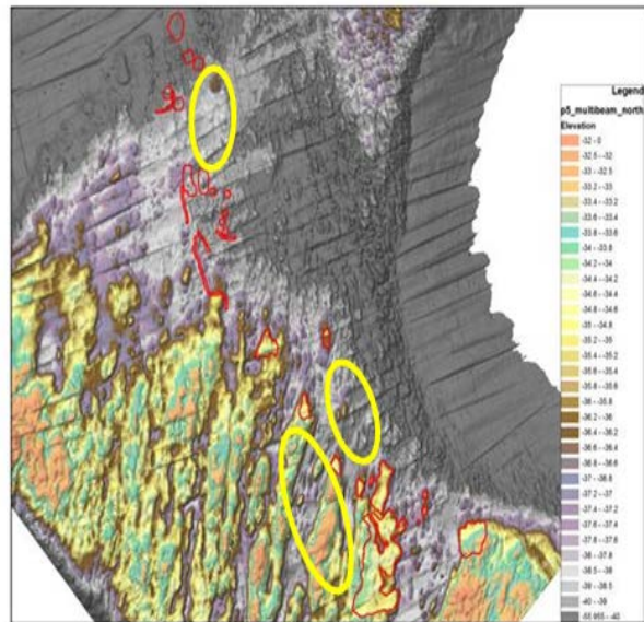
Figure 10: Location of reference transects (yellow polygons) adjacent to the T/V MARGARA site (impacted areas delineated in red).
