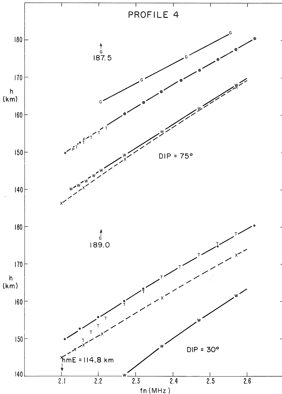
Fig. 13. Calculated and correct real heights for the base of the F layer for the profile 4 used for the valley tests.
