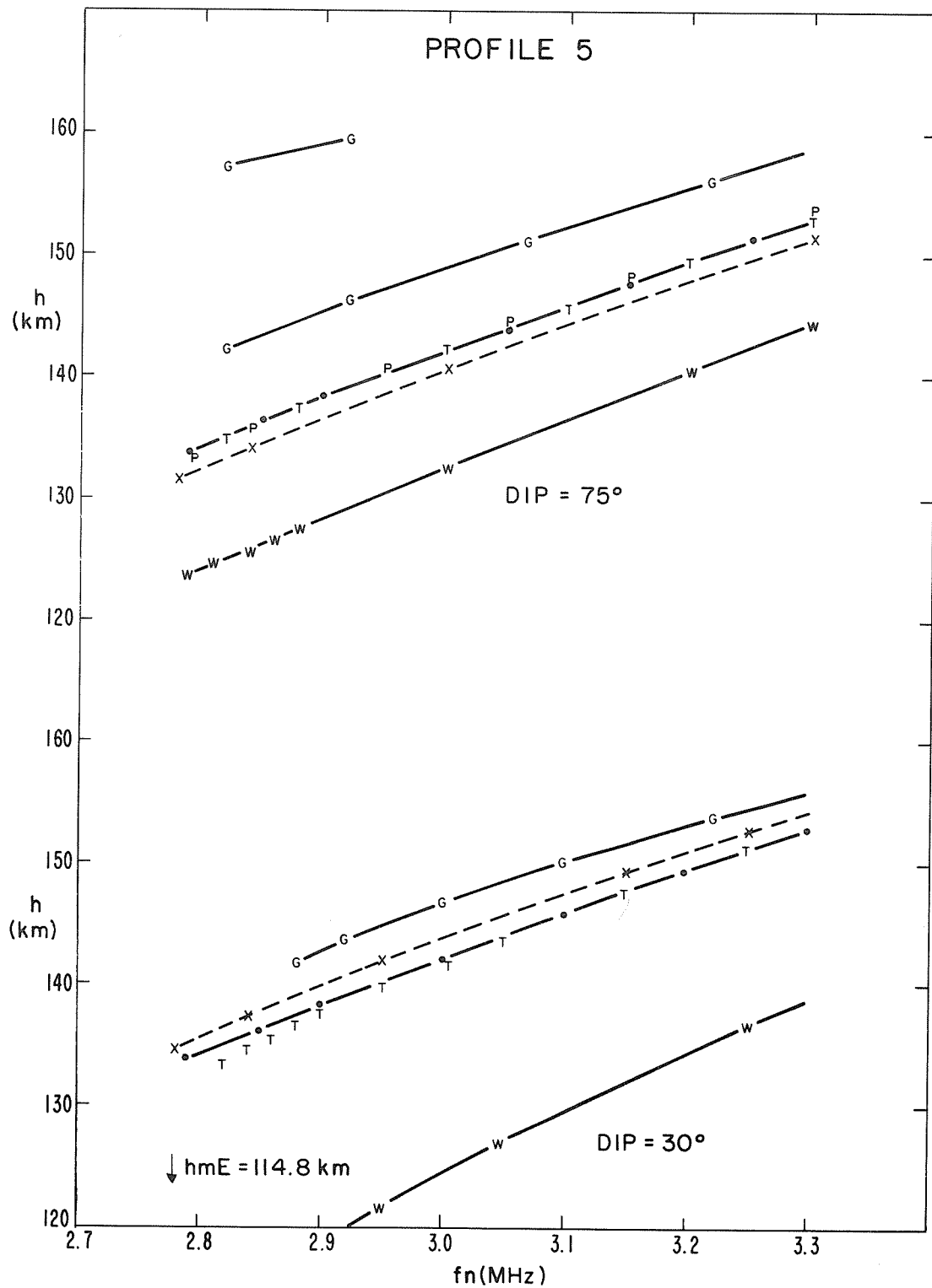
Fig. 14. Calculated and correct real heights for the base of the F layer for the profile 5 used for the valley tests.
