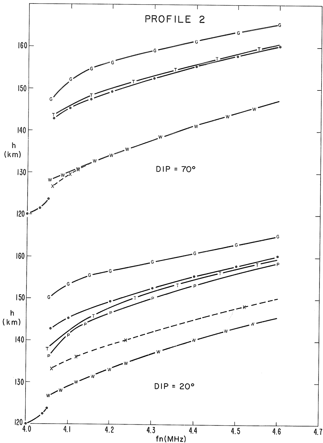
Fig. 11. Calculated and correct real heights for the base of the F layer for the profile 2 used for the valley tests
