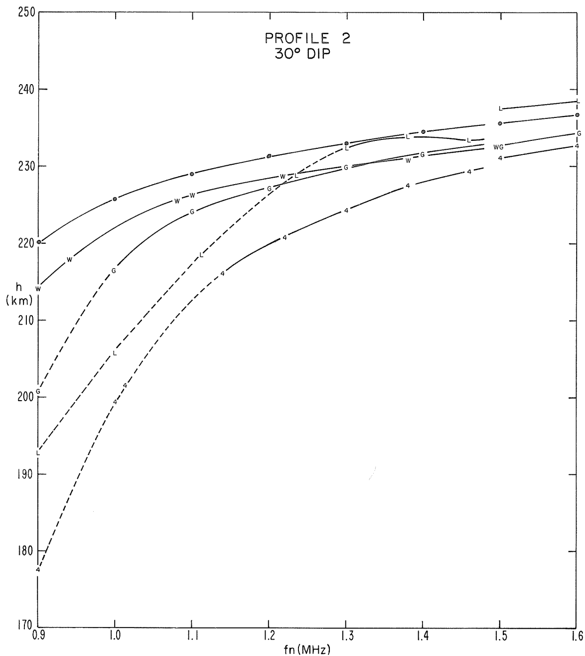
Fig. 4. Calculated and correct real heights for the lower parts of profile 2 used for the underlying ionization tests
