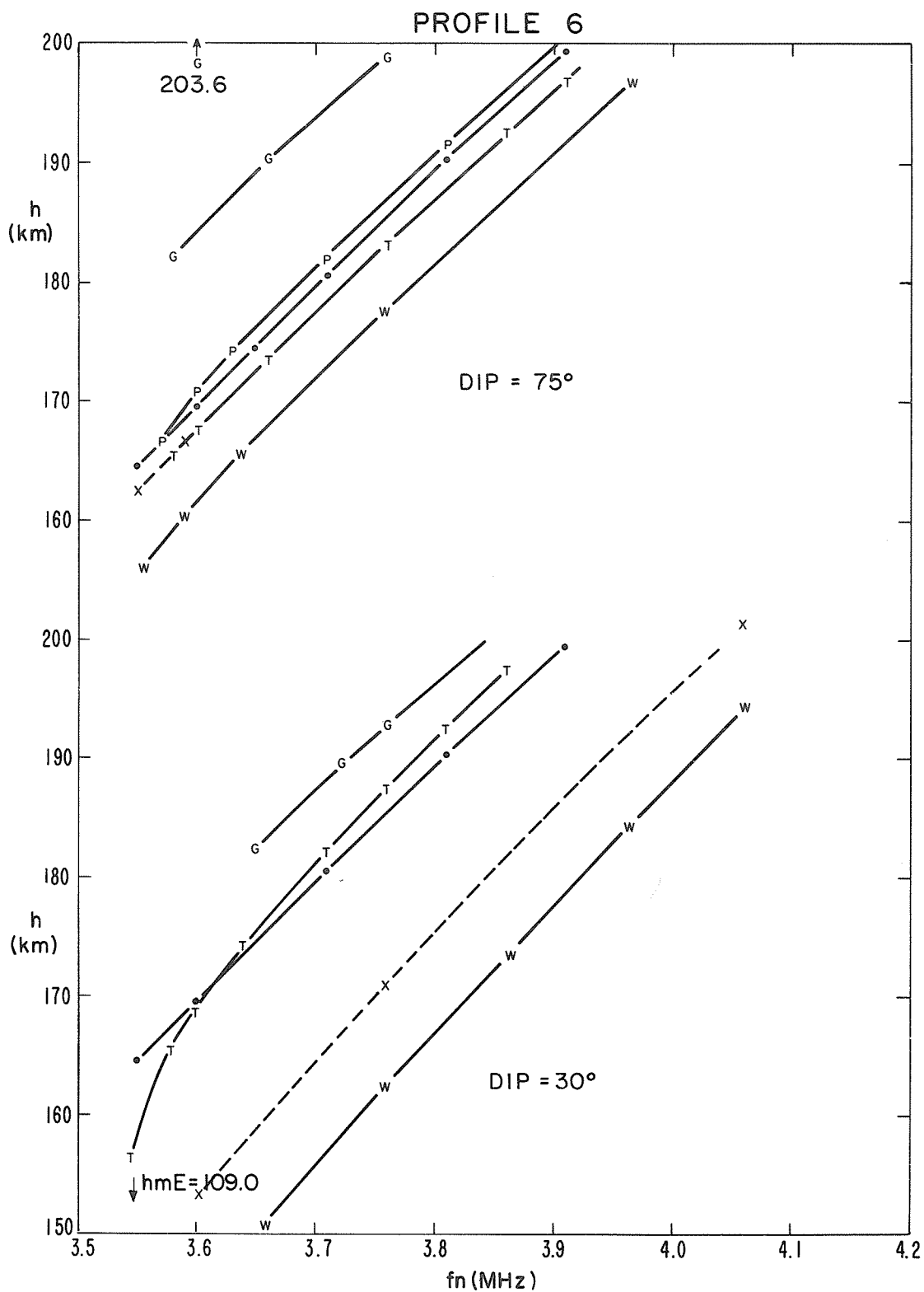
Fig. 15. Calculated and correct real heights for the base of the F layer for the profile 6 used for the valley tests.
