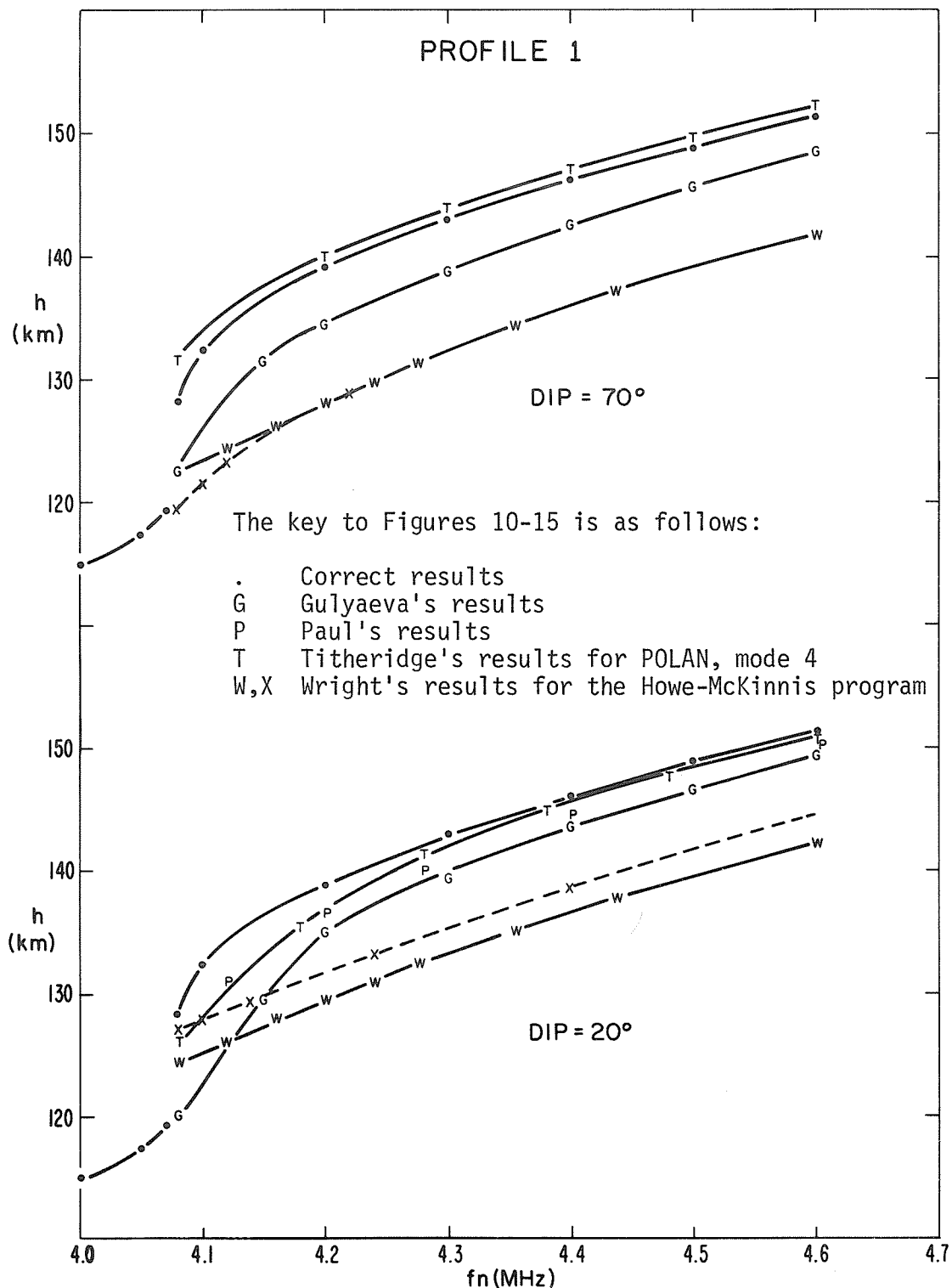
Fig. 10. Calculated and correct real heights for the base of the F layer for the profile 1 used for the valley tests
