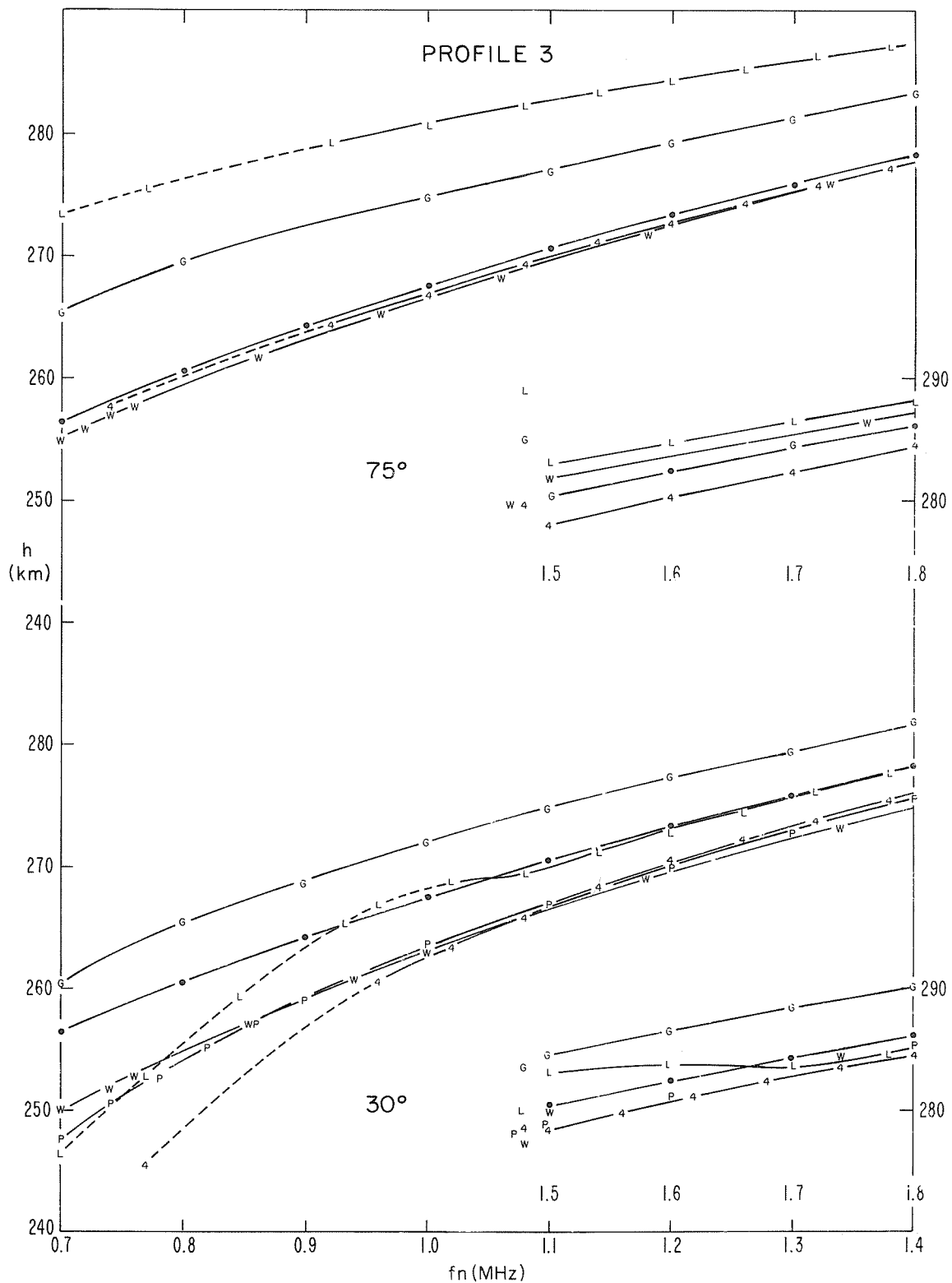
Fig. 6. Calculated and correct real heights for the lower parts of profile 3 used for the underlying ionization tests
