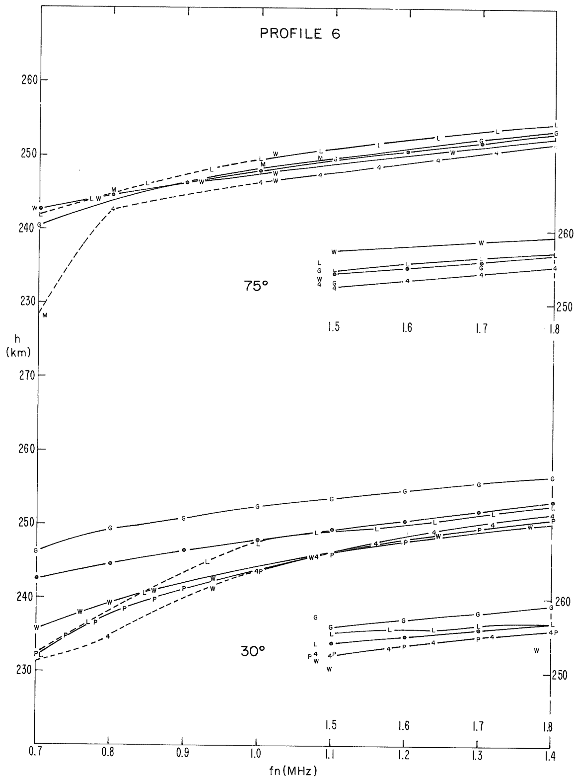
Fig. 9. Calculated and correct real heights for the lower parts of profile 6 used for the underlying ionization tests
