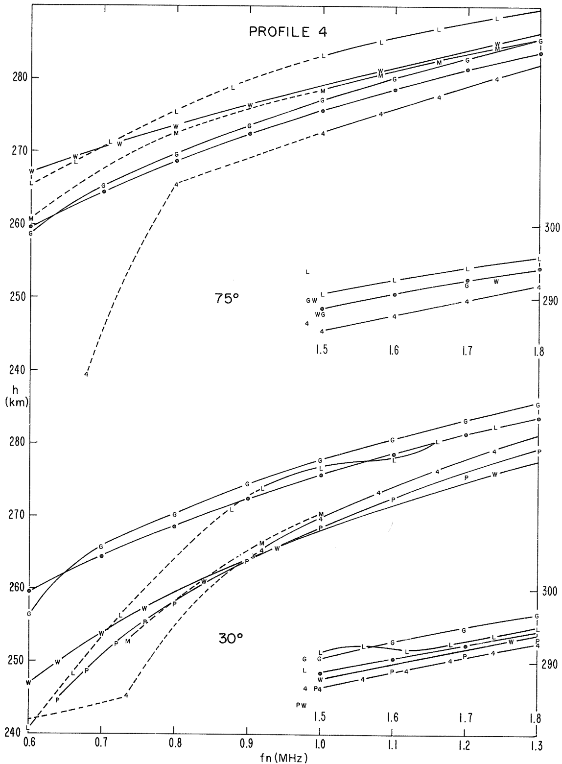
Fig. 7. Calculated and correct real heights for the lower parts of profile 4 used for the underlying ionization tests
