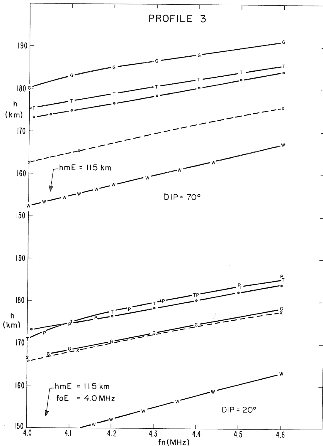
Fig. 12. Calculated and correct real heights for the base of the F layer for the profile 3 used for the valley tests.
