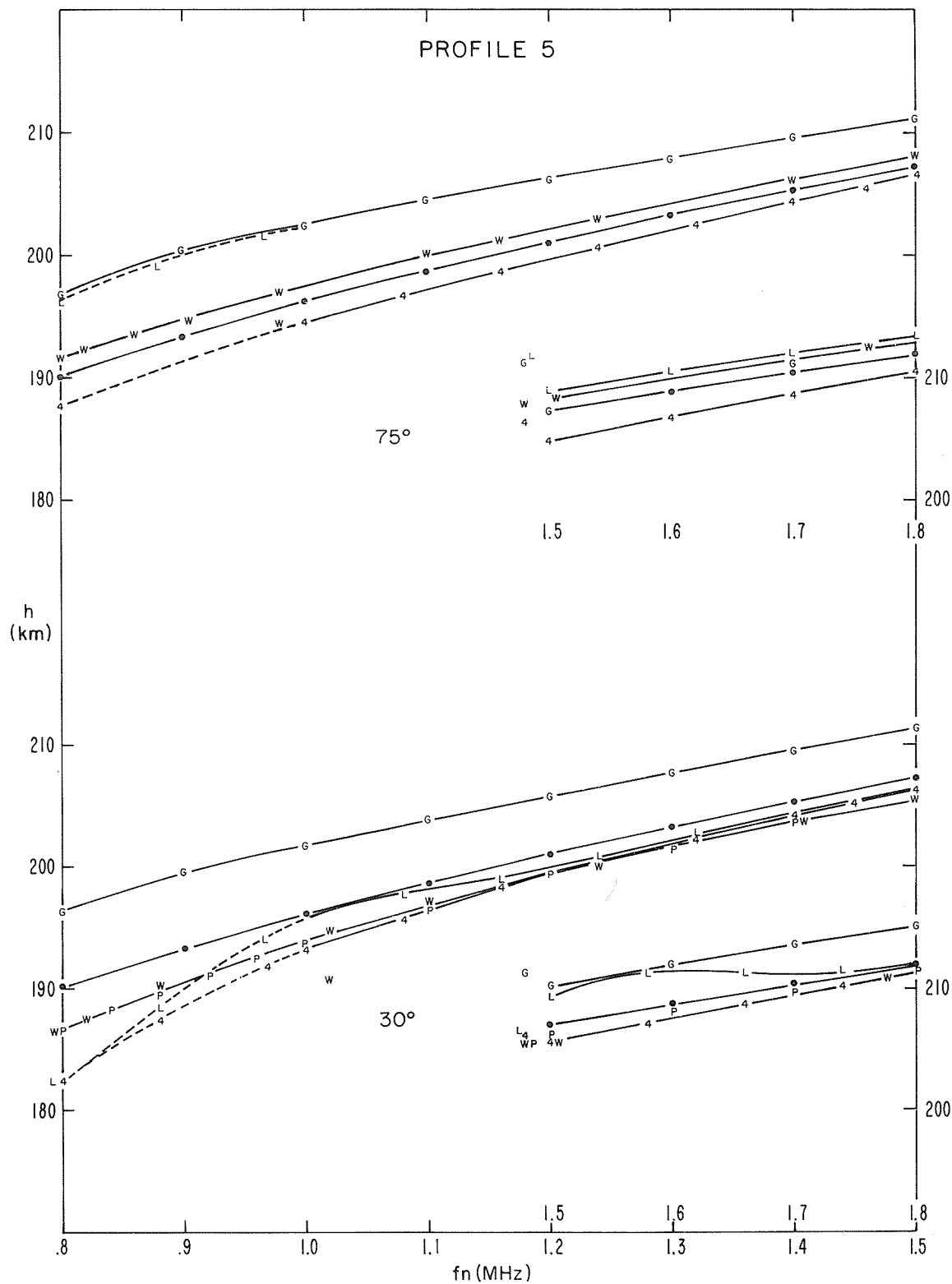
Fig. 8. Calculated and correct real heights for the lower parts of profile 5 used for the underlying ionization tests
