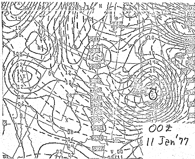
FIG. 1 Flattery 500-mb analyses. — Abs vorticity \times 10^5 \text{ sec} . --- height contours
