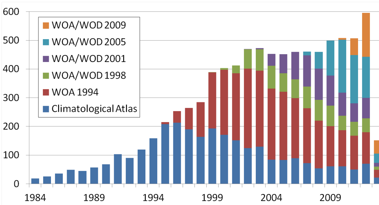
Figure 4: Citation counts received by all versions of the World Ocean Atlas (WOA) and World Ocean Database (WOD) in Web of Science per year. Together, these atlases and databases have been cited over 8,500 times. These counts are accurate as of June 12, 2013.
