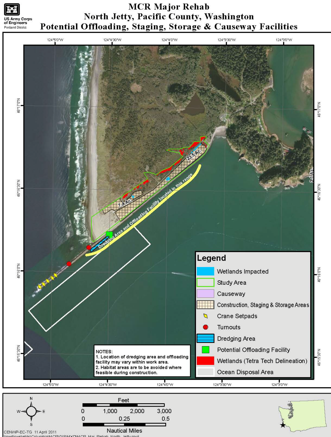
Figure 38. North Jetty Offloading, Staging, Storage and Causeway Facilities
