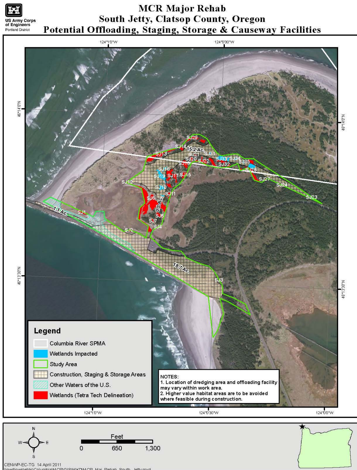
Figure 45. Illustration of Avoidance, Minimization, and Wetland Impacts at South Jetty
