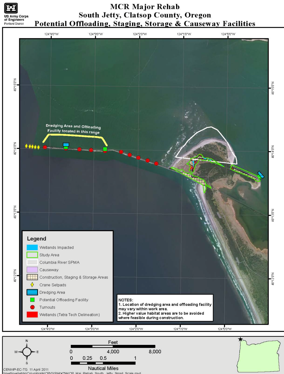
Figure 39. South Jetty Offloading, Staging, Storage and Causeway Facilities
