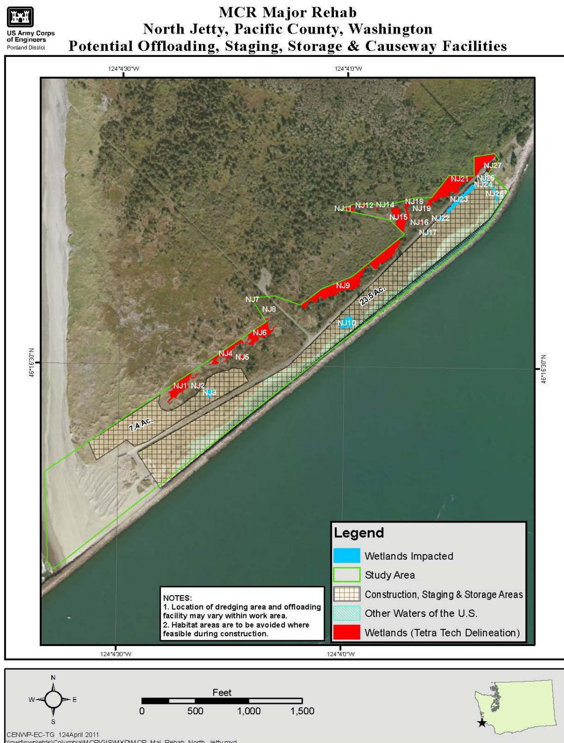
Figure 43. Illustration of Avoidance, Minimization, and Wetland and Waters Impacts at North Jetty
