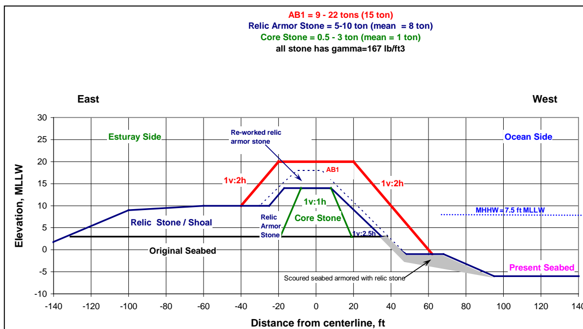
Figure 31. Jetty A Cross Section for Proposed Action (No Longer Proposed. Cross-section Will Be Similar to that of North Jetty)
