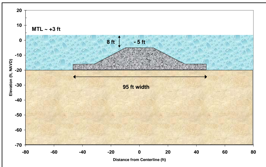
Figure 34. Jetty A Spur Groin JA2O (No Longer Proposed)
