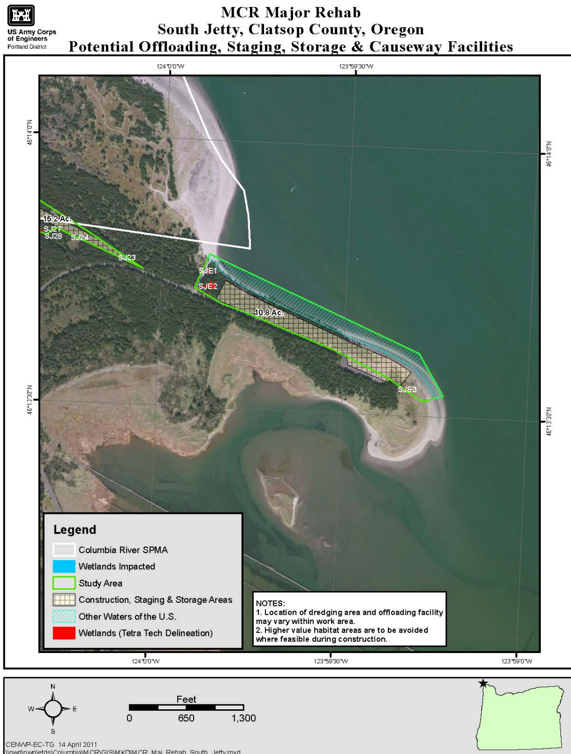
Figure 45 Continued: Illustration of Avoidance, Minimization, and Wetland Impacts at South Jetty
