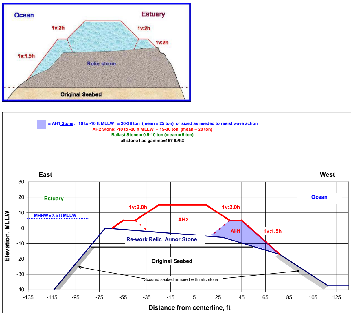
Figure 35. Jetty A Head Cap (No Longer Proposed; Replaced With Reduced Stabilization Measure)
