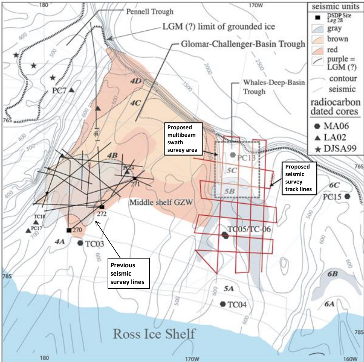
Figure 2. Proposed tracklines for the low-energy seismic survey in the Ross Sea.
