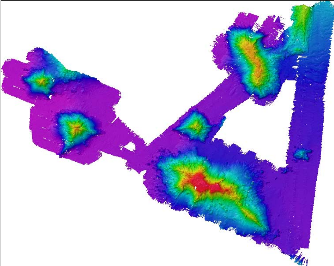
Figure 11. 50 meter cell size grid showing total mapping completed with EM302 during cruise EX0909 Leg 4. Image generated in Fledermaus v. 6.7. Image credit: NOAA.
