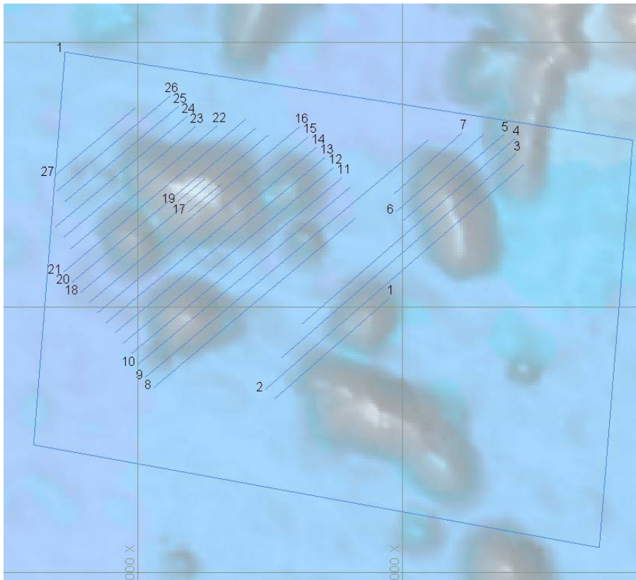
Figure 4. Third line plan (implemented November 3 rd ). Background data: satellite altimetry, source Sandwell and Smith. Image generated in Hypack 2009. Image credit: NOAA.
