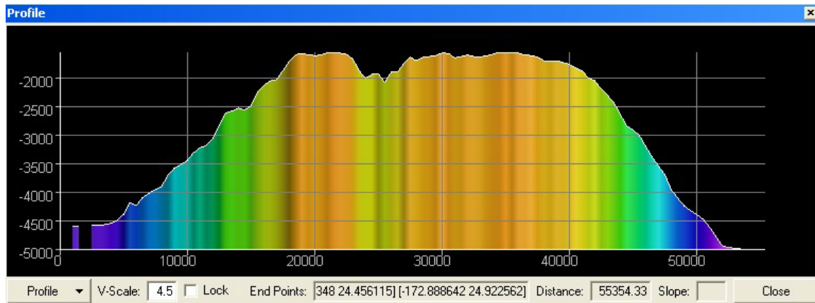
Figure 12. Profile view of Ha'aheo Seamount. Units shown in meters. Height of Ha'aheo Seamount above surrounding seafloor = approx. 3200m.
