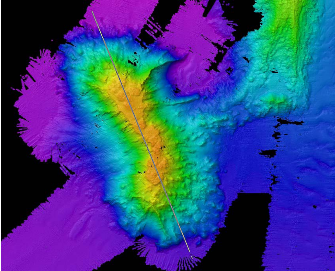
Figure 13. Overview of Ha'aheo Seamount. White line indicates direction of depth profile shown in Fig. 11 above. Image generated in Fledermaus v. 6.7. Image credit: NOAA.
