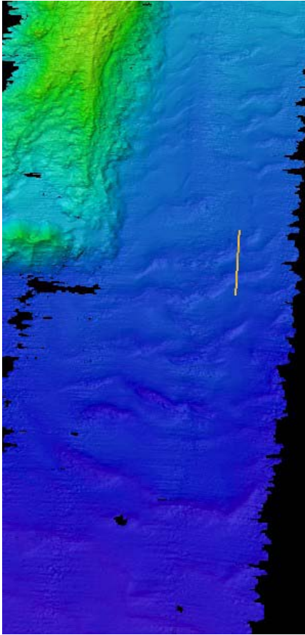
Figure 15. Interesting sediment or lava flow pattern at northeast corner of survey site near Ha'aheo Seamount and Northhampton Seamounts extension. White line indicates profile in Fig. 14 above. Image generated in Fledermaus v. 6.7. Image credit: NOAA.
