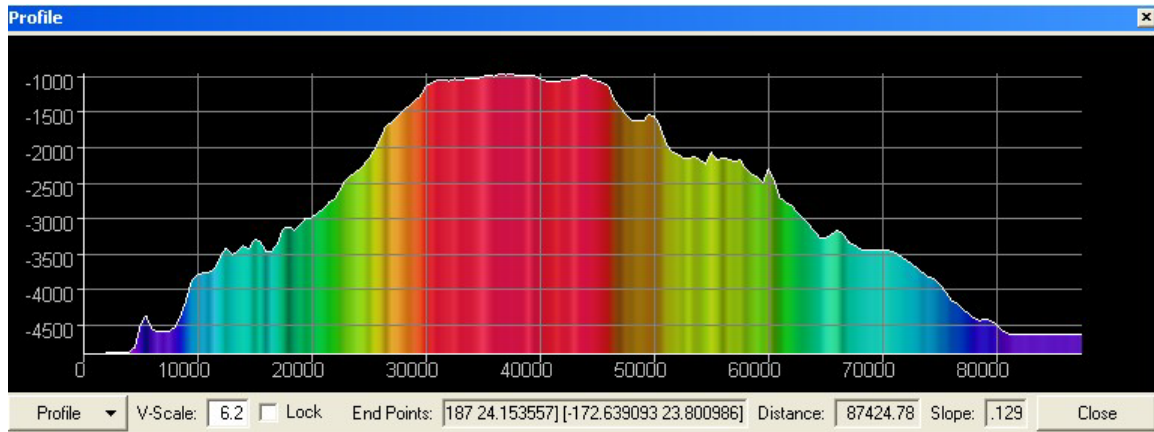
Figure 20. Profile of Tamana seamount. Units shown in meters. Height of Tamana Seamount above surrounding seafloor = approx. 3600m. Image generated in Fledermaus v. 6.7. Image credit: NOAA.
