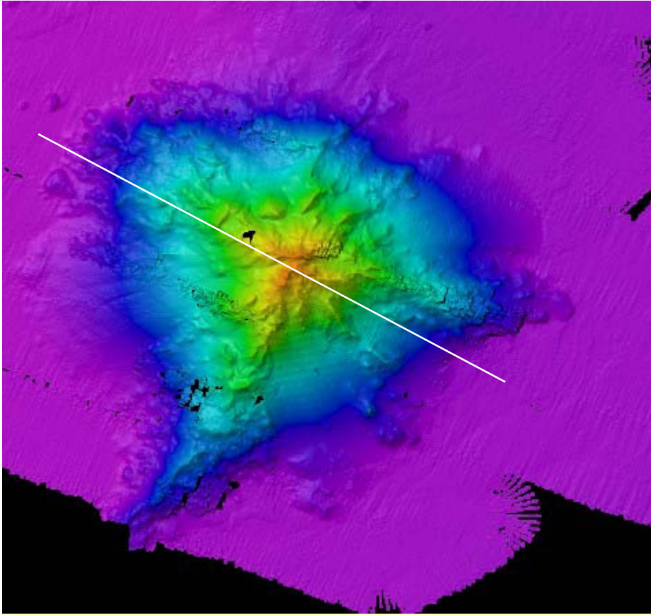
Figure 19. Overview of Euphemia Seamount. White line indicates direction of profile shown in Fig. 17 above. Image generated in Fledermaus v. 6.7. Image credit: NOAA.
