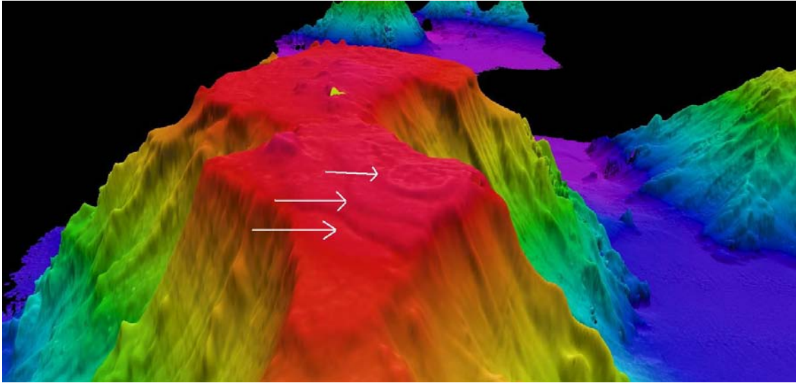
Figure 22. Looking west over Tamana Seamount. Possible extinct coastlines or coral reefs indicated by white arrows. Image generated in Fledermaus v. 6.7. Image credit: NOAA.
