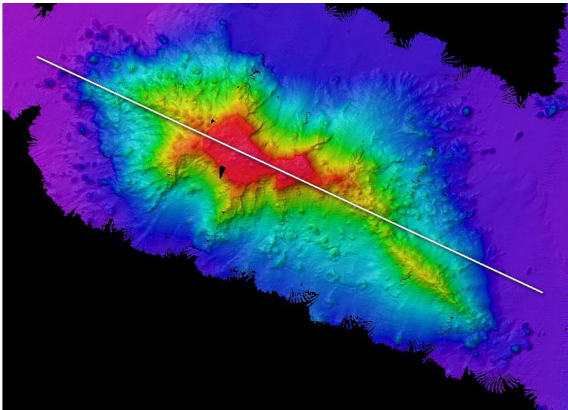
Figure 21. Overview of Tamana Seamount. White line indicates direction of profile shown above in Fig. 19. Image generated in Fledermaus v. 6.7. Image credit: NOAA.
