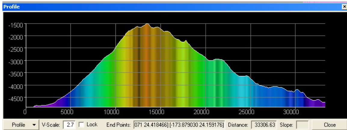
Figure 18. Profile view of Euphemia Seamount. Height of Euphemia Seamount above surrounding seafloor = approx. 3200m.
