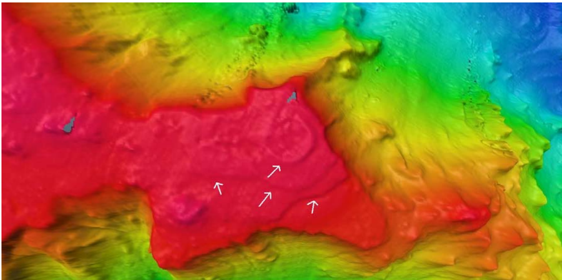
Figure 23. Overview of eastern section of planed top of Tamana Seamount. Possible extinct coastlines or coral reefs indicated by white arrows. Image generated in Fledermaus v. 6.7. Image credit: NOAA.
