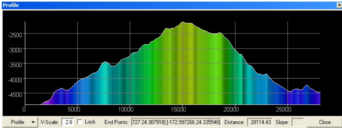
Figure 16. Profile of Sovereign Seamount. Units shown in meters. Height of Sovereign Seamount above surrounding seafloor = approx. 2700m. Image generated in Fledermaus v. 6.7. Image credit: NOAA.
