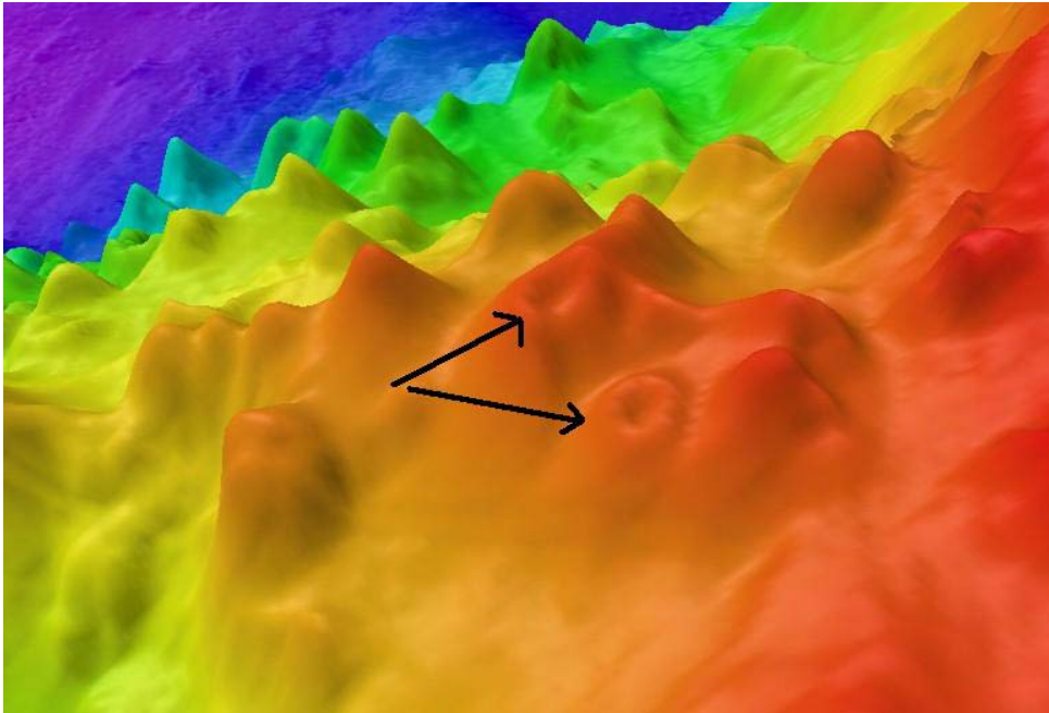
Figure 24. Parasitic cones, indicated by black arrows, found on western flank of Tamana Seamount. White line indicates direction of profile. Parasitic cone centers found to 20m deep or less. Image generated in Fledermaus v. 6.7. Image credit: NOAA.
