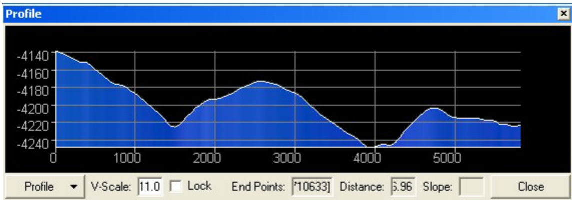
Figure 14. Profile of interesting sediment or lava flow pattern at northeast corner of survey site near Ha'aheo Seamount and Northhampton Seamounts extension. Image generated in Fledermaus v. 6.7. Image credit: NOAA.
