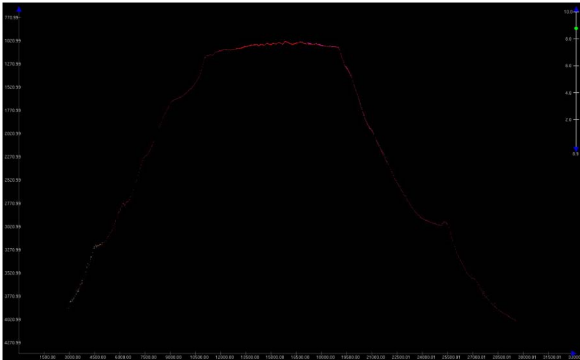
Figure 7. Screengrab of along track view of crossline over Tamana Seamount, showing agreeable crossline comparison with mainscheme lines. Crossline data are shown as red points, mainscheme data are shown as points in various other colors. Image generated in CARIS HIPS and SIPS v. 6.1. Image credit: NOAA.
