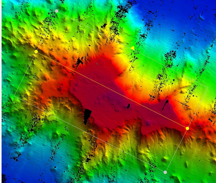
Figure 10. Screenshot showing data of Tamana Seamount loaded into subset editor for across track crossline comparison shown in Fig. 9 above. Image generated in CARIS HIPS and SIPS v. 6.1. Image credit: NOAA.
