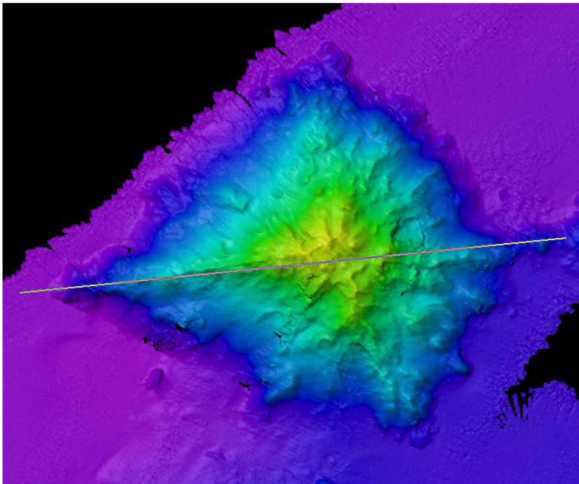
Figure 17. Overview of Sovereign Seamount. White line indicates profile trace shown above in Fig. 16. Image generated in Fledermaus v. 7. Image credit: NOAA.
