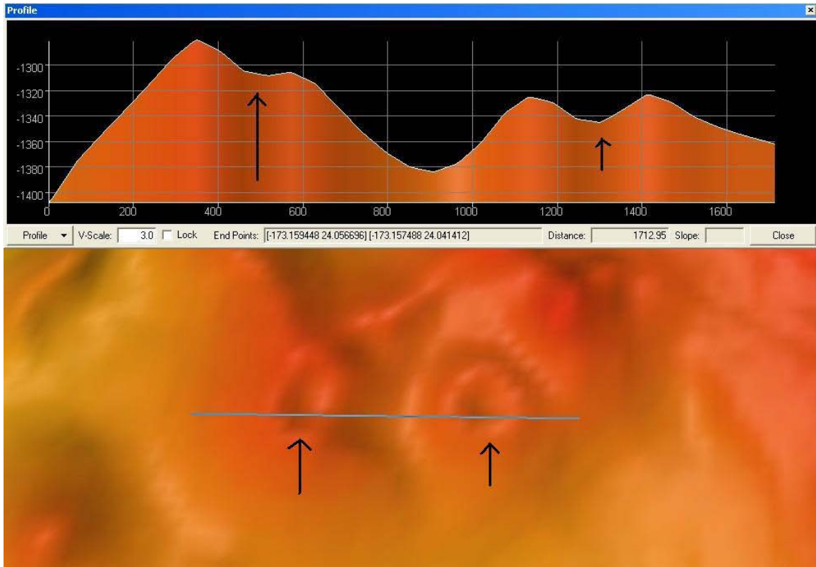
Figure 24. Parasitic cones, indicated by black arrows, found on western flank of Tamana Seamount. White line indicates direction of profile. Parasitic cone centers found to 20m deep or less. Image generated in Fledermaus v. 6.7. Image credit: NOAA.
