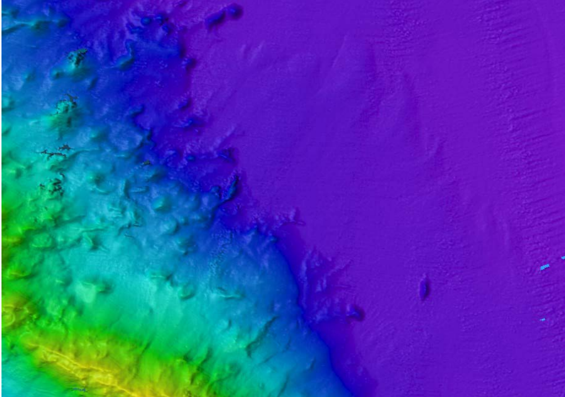
Figure 26. Interesting lava or sediment flow off of eastern flank of Tamana Seamount. Image generated in Fledermaus v. 6.7. Image credit: NOAA.
