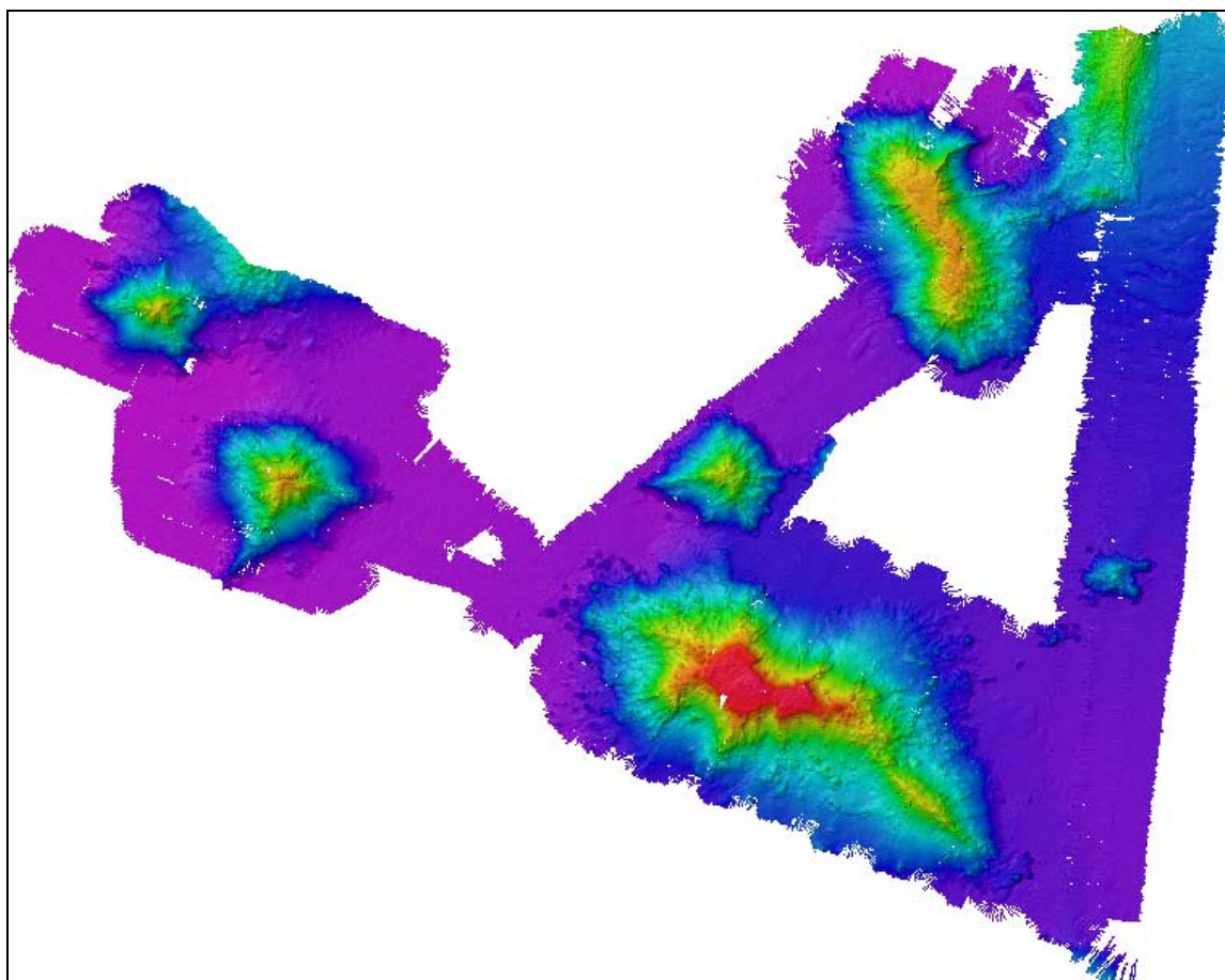
Figure 10. 50 meter cell size grid showing total seamount mapping area completed with EM302 during cruise EX0909 Leg 4. Image generated in Fledermaus. Image credit: NOAA.
