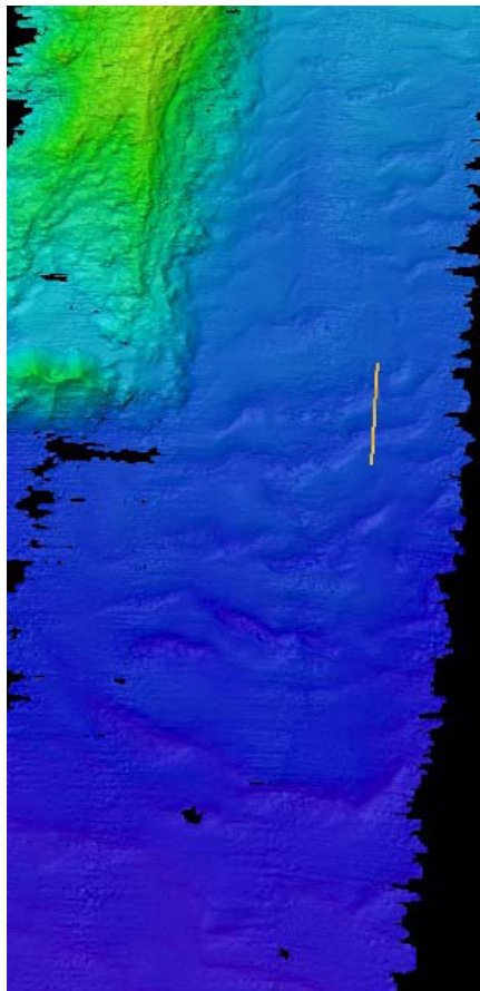
Figure 14. Interesting sediment or lava flow pattern at northeast corner of survey site near Ha'aheo Seamount and Northhampton Seamounts extension. White line indicates profile in Fig. 13 above. Image generated in Fledermaus. Image credit: NOAA.
