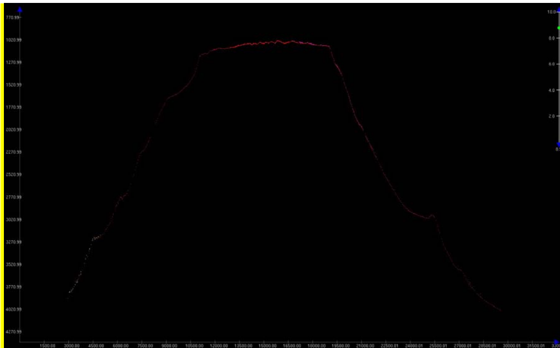
Figure 7. Screenshot of along track view of crossline over Tamana Seamount, showing agreeable crossline comparison with mainscheme lines. Crossline data are shown as red points, mainscheme data are shown as points in various other colors. Image generated in CARIS. Image credit: NOAA.
