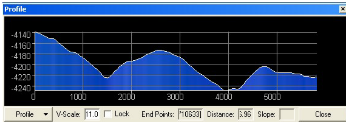
Figure 13. Profile of interesting sediment or lava flow pattern at northeast corner of survey site near Ha'aheo Seamount and Northhampton Seamounts extension. Image generated in Fledermaus. Image credit: NOAA.
