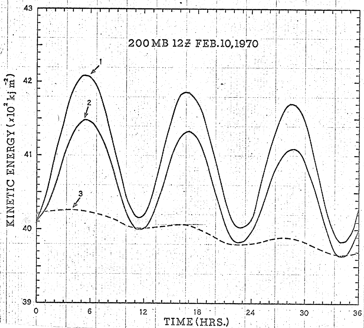
Fig. 5. The average kinetic energy as forecasted by the barotropic primitive equation model for experiments I, II and III.
