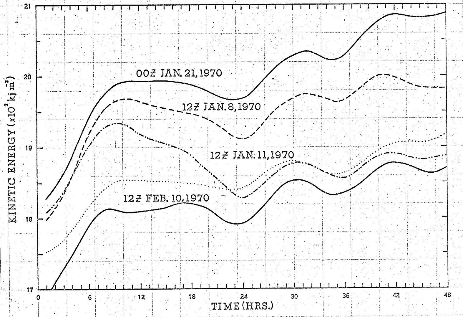
Fig. 1. Examples of the average kinetic energy as forecasted by the NMC six-layer primitive equation model. The dotted curve represents the modified forecast of 1200 GMT February 10, 1970.
