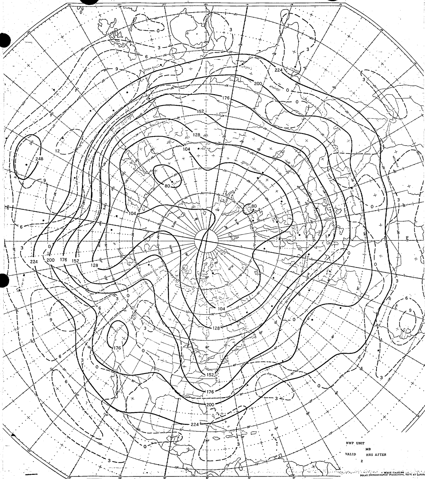
Fig. 4. The 200-mb analyzed geopotential height field (solid) and the analyzed minus ellipticized height field (dashed) for 1200 GMT February 1970. Units are decameters.
