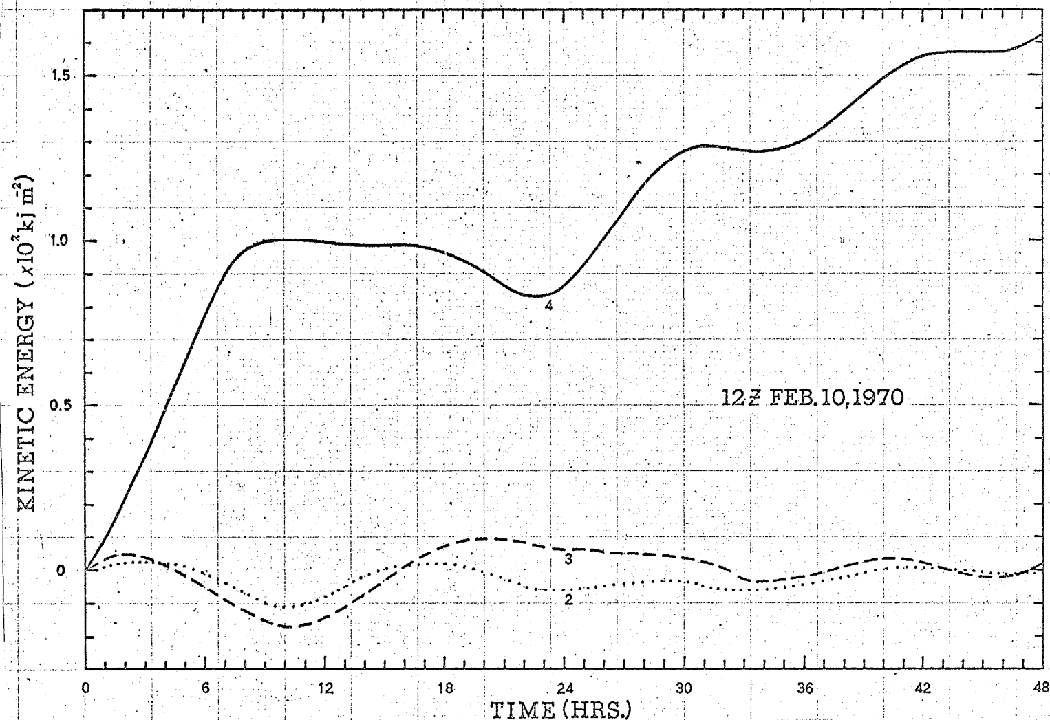
Fig. 2. The average kinetic energy variation as forecasted from 1200 GMT February 10, 1970 by the NMC six-layer primitive equation model for the three layers initially comprising the entire troposphere above the boundary layer. The values have been normalized as described in the text.
