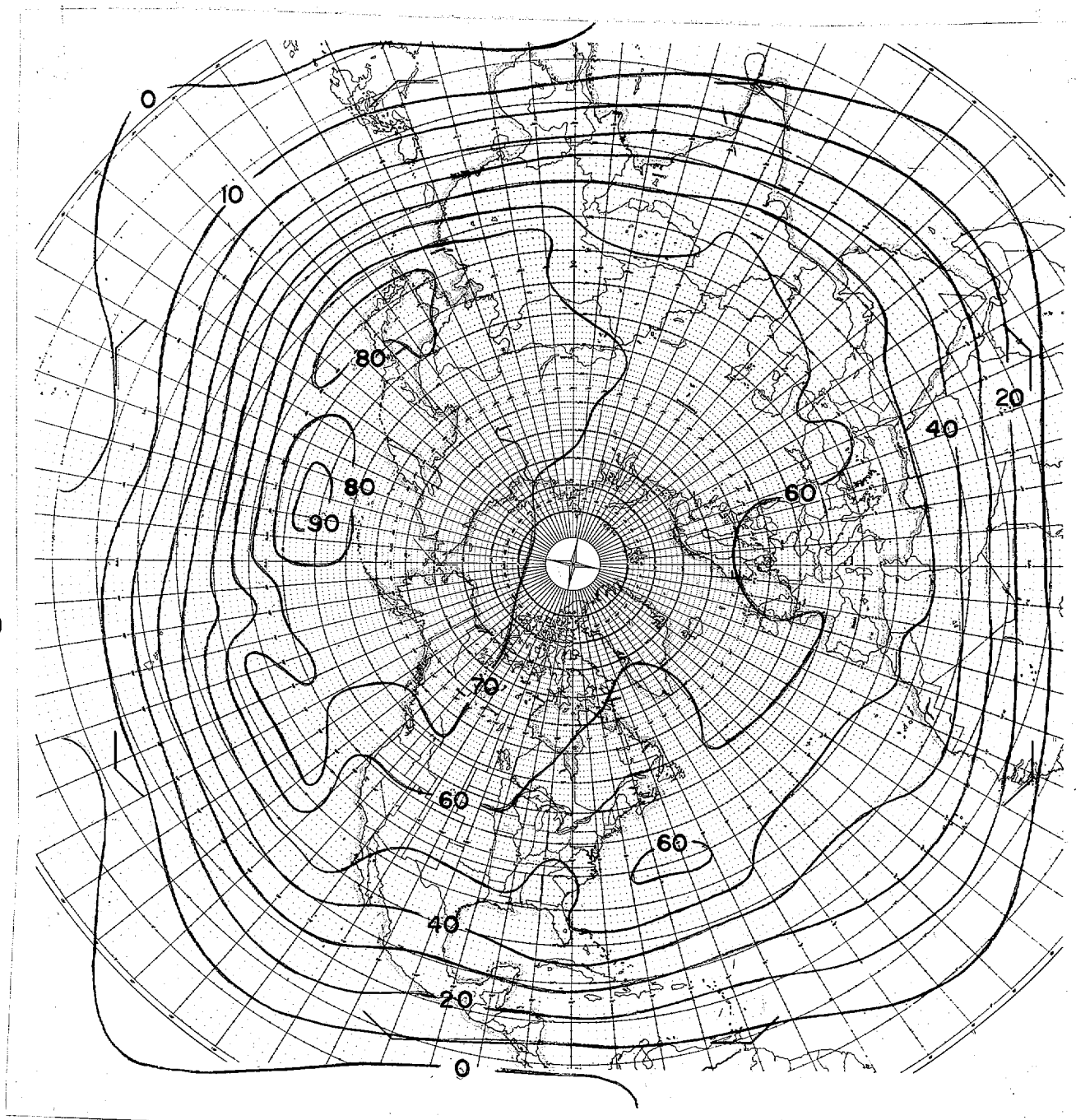
Fig. 6. The field of \phi^* in meters.
