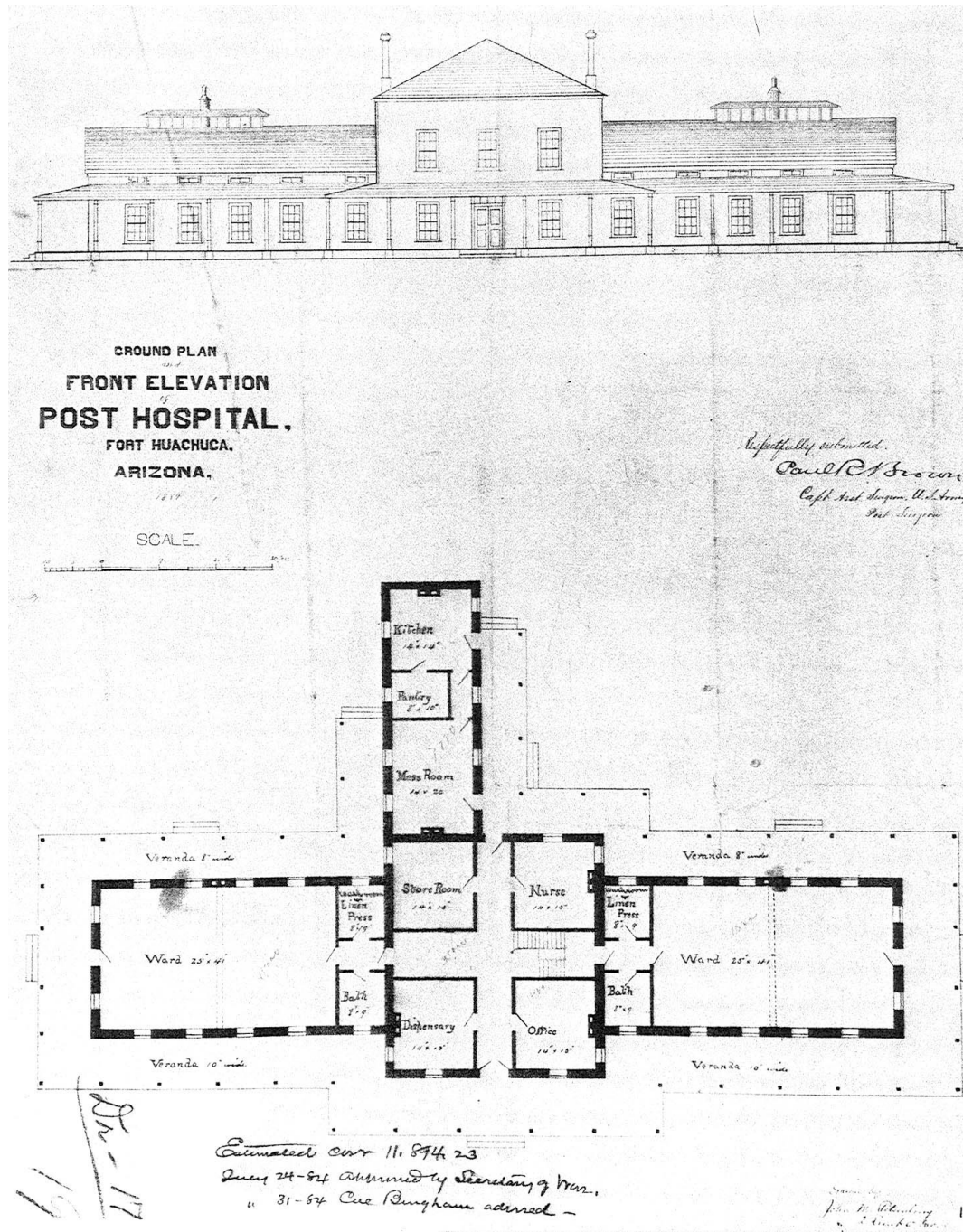
Figure 3. Plans for Hospital, 1884 Source: Fort Huachuca Museum
