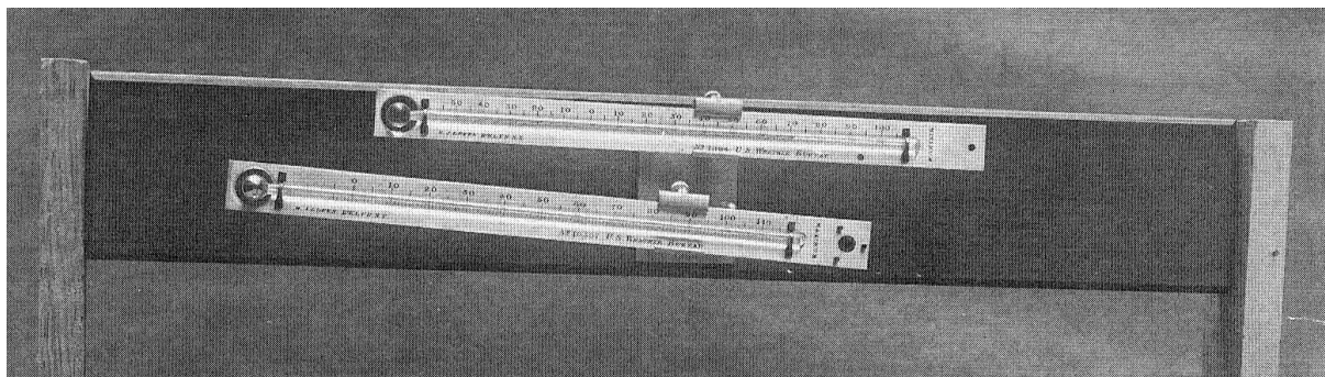
Figure 10. Green Maximum and Minimum Thermometers on a Townsend Mount Source: National Archives and Records Administration
