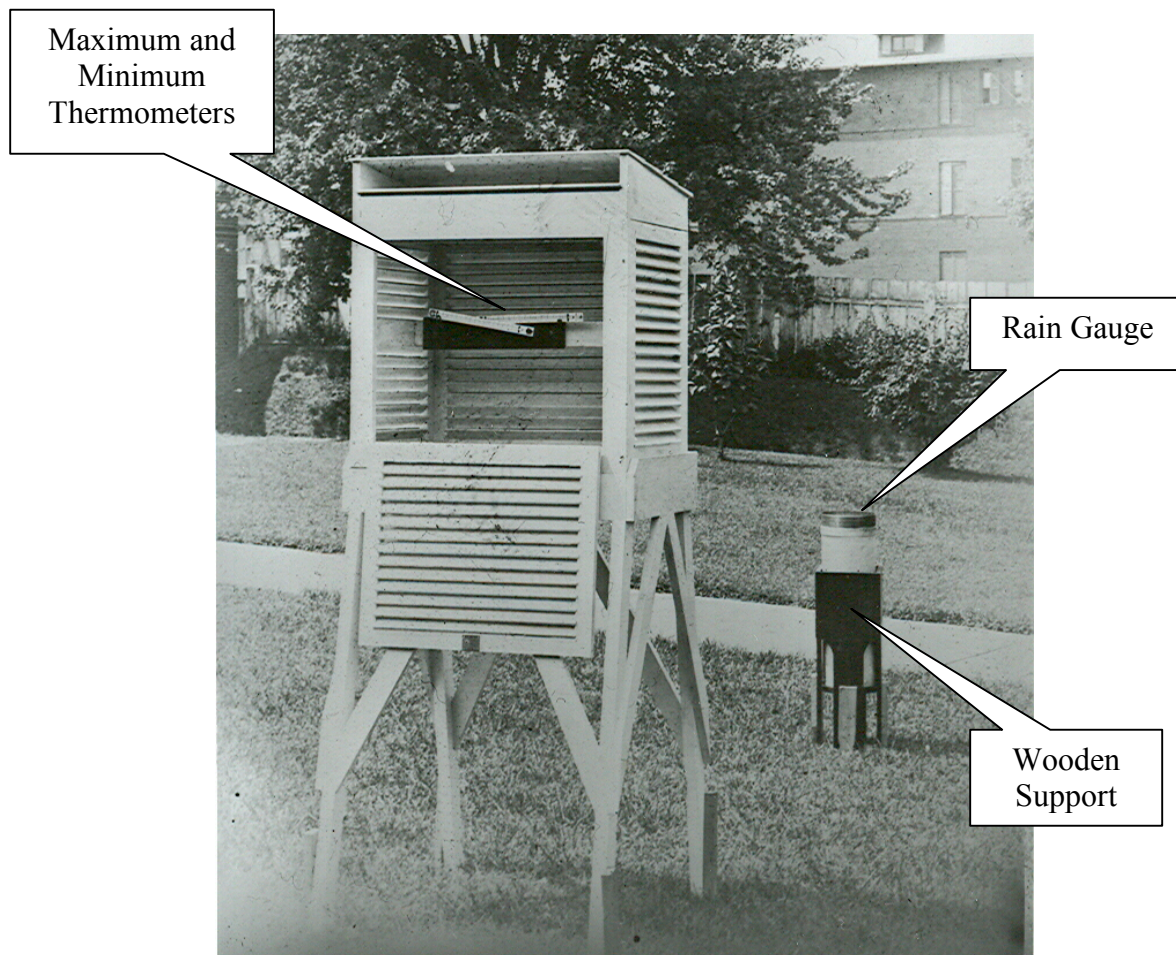
Figure 15. Maximum-Minimum Thermometers in Instrument Shelter, Rain Gauge on Right Source: Utah Historical Society, J. Cecil Alter Collection, C-102 Box 1
