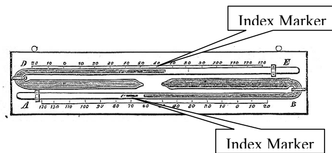
Figure 9. Self-Registering Thermometer Source: Loomis' Treatise on Meteorology, 1868
