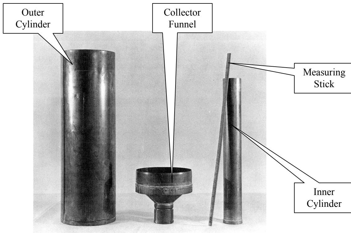
Figure 14. Standard Eight Inch Rain Gauge Source: National Archives and Records Administration
