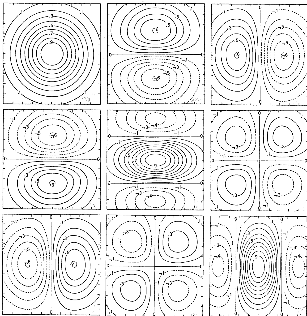
Figure 7. Horizontal correlation functions for geopotential and wind. Left to right, top row: h-h , h-u , h-v ; middle row: u-h , u-u , u-v ; bottom row: v-h , v-u , v-v . Distance intervals correspond to 300 km. After Bergman (1979).
