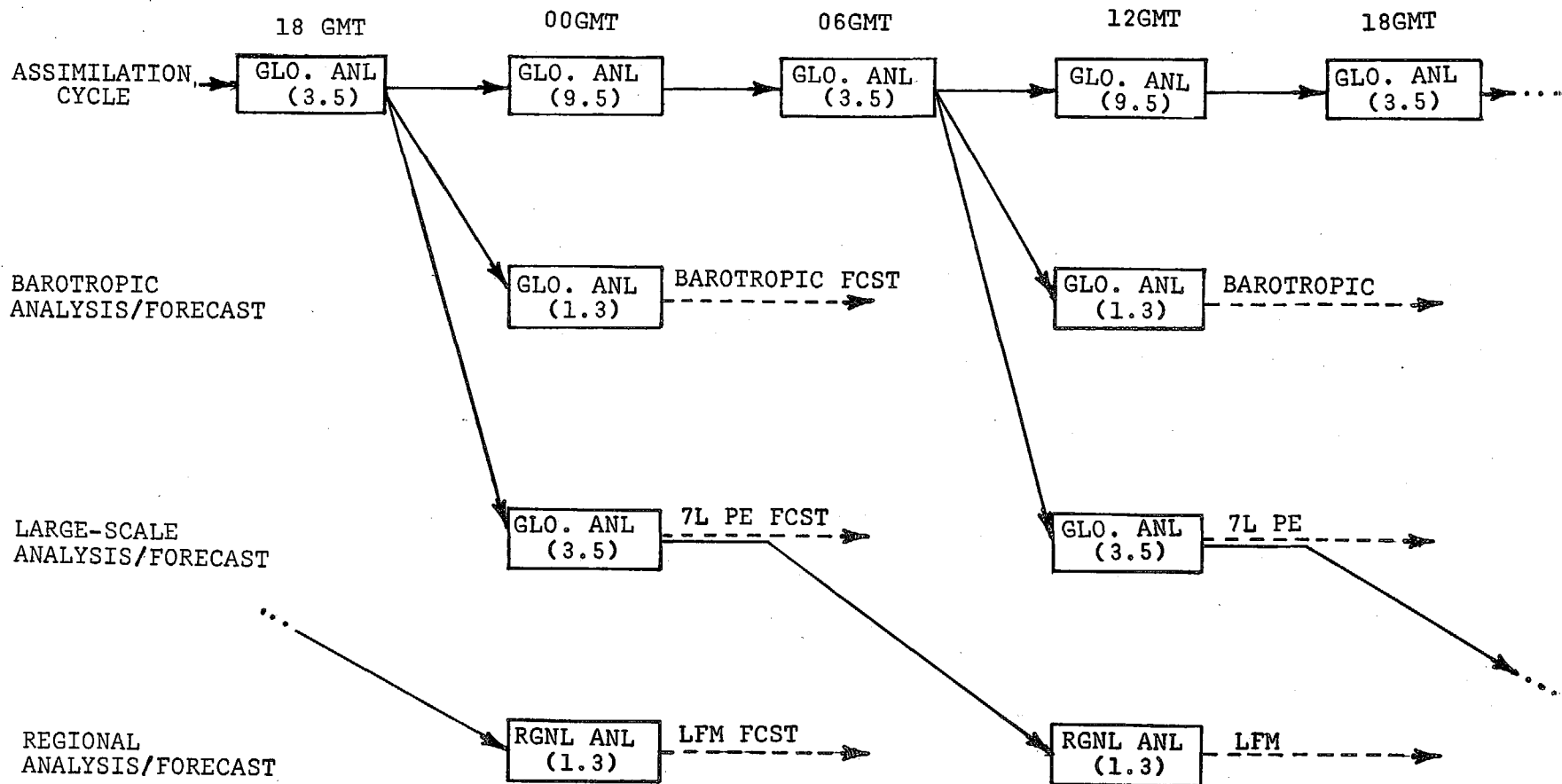
Figure 5. Schematic diagram of the NMC operational assimilation and analysis/forecast system as of 1 January 1980. Boxes represent analyses (updates), with parenthetical numbers indicating cutoff time. Solid lines denote the origin of the background fields for each update, and the dashed lines represent operational forecasts.
