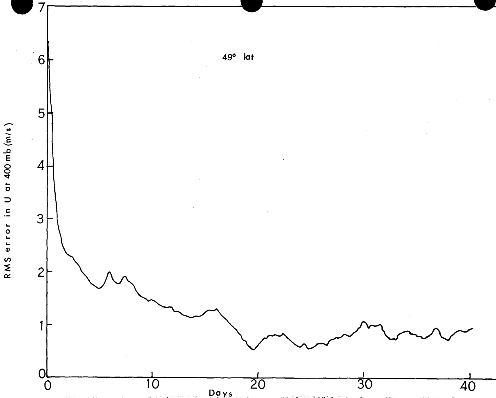
Figure 3. RMS error in 400-mb zonal wind component for 49° latitude as a function of time. Wind induced by inserting "perfect" simulated temperatures plus random error of 1°C. After Charney, Halem, and Jastrow (1969).
