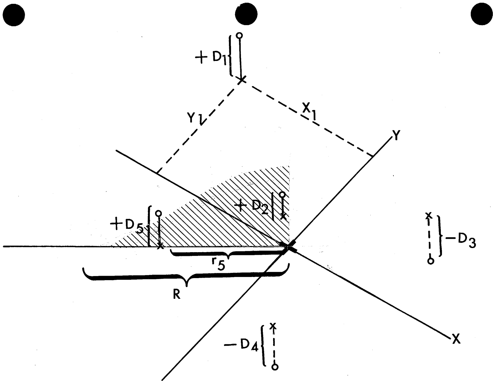
Figure 2. Distribution of observations as in Fig. 1, but with the successive-corrections weighting function superimposed.
