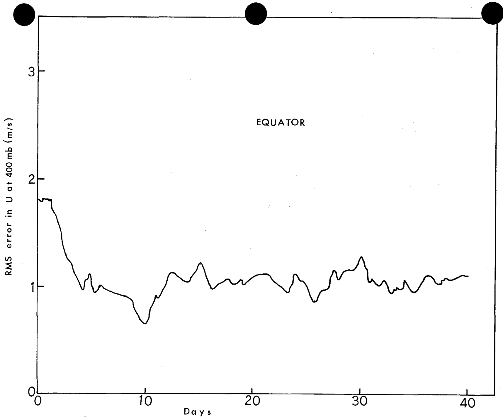
Figure 4. Same as Fig. 3, but for the equator. After Charney, Halem, and Jastrow (1969).
