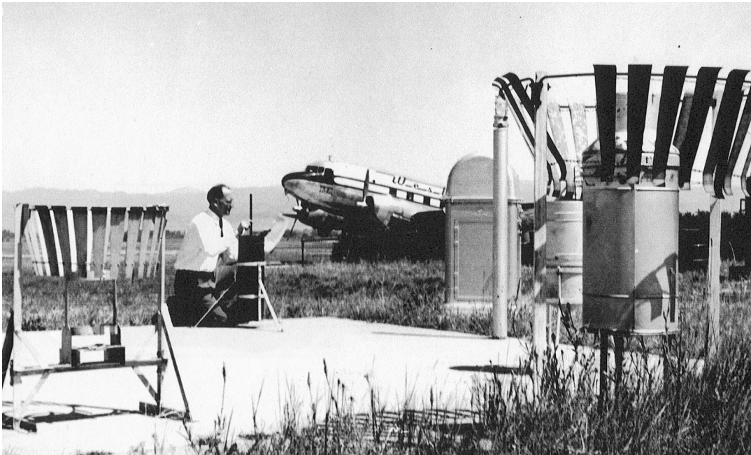
Figure 23. Rain Gauges at the Helena Airport Observation Site Source: Montana Historical Society
