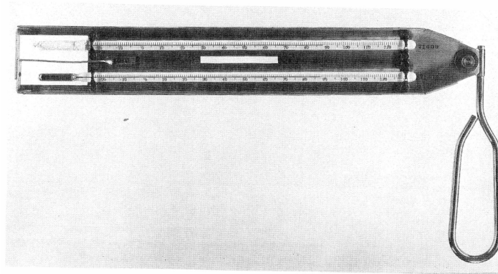
Figure 20. Sling Psychrometer, Wet Bulb above, Dry Bulb Below Source: National Archives and Records Administration
