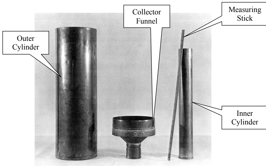
Figure 22. Standard Eight Inch Rain Gauge Source: National Archives and Records Administration
