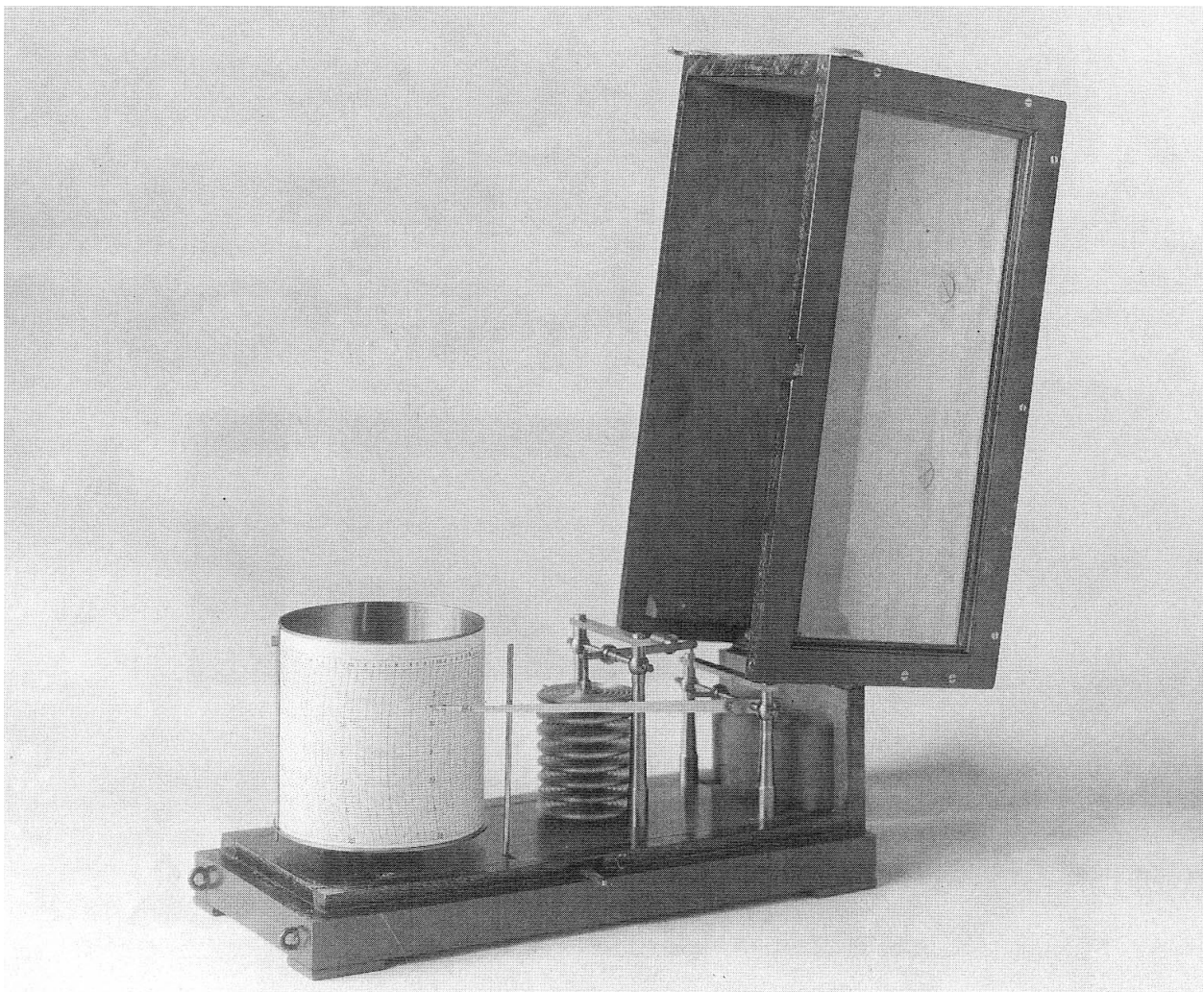
Figure 26. Barograph
