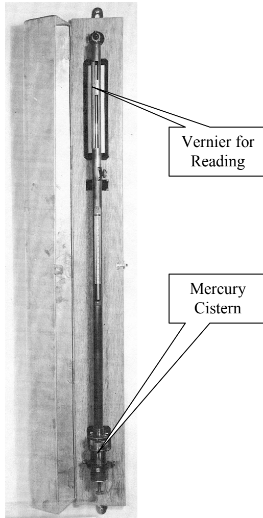
Figure 25. Mercury Barometer Source: National Archives and Records Administration
