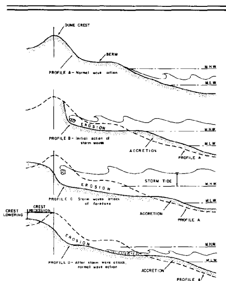
Figure 3 — Creation of nearshore bar during a storm.
