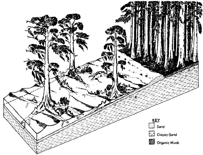
Figure 4 — The cypress fringe damping erosion wave forces and trapping sediments is illustrated in this figure. The cypress trees can form a natural bulkhead which dissipates wave energy and traps sand.
