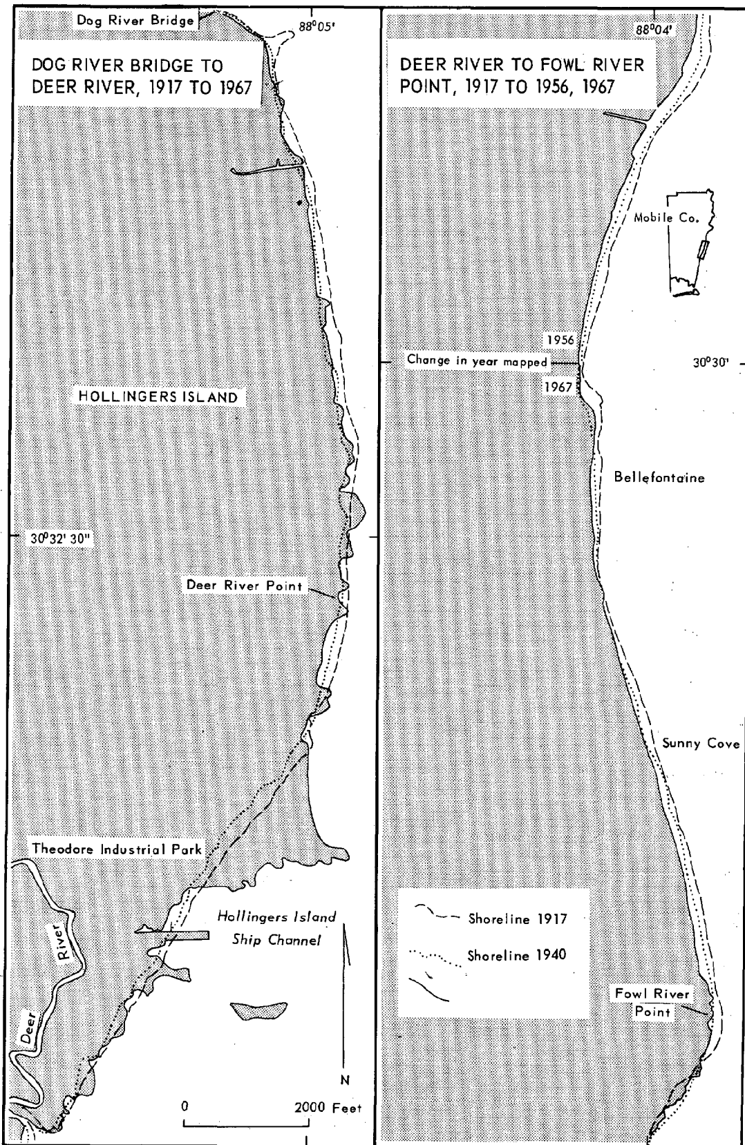
Figure 36. --Shoreline changes between Dog River Bridge and Fowl River Point between 1917 and 1967.
