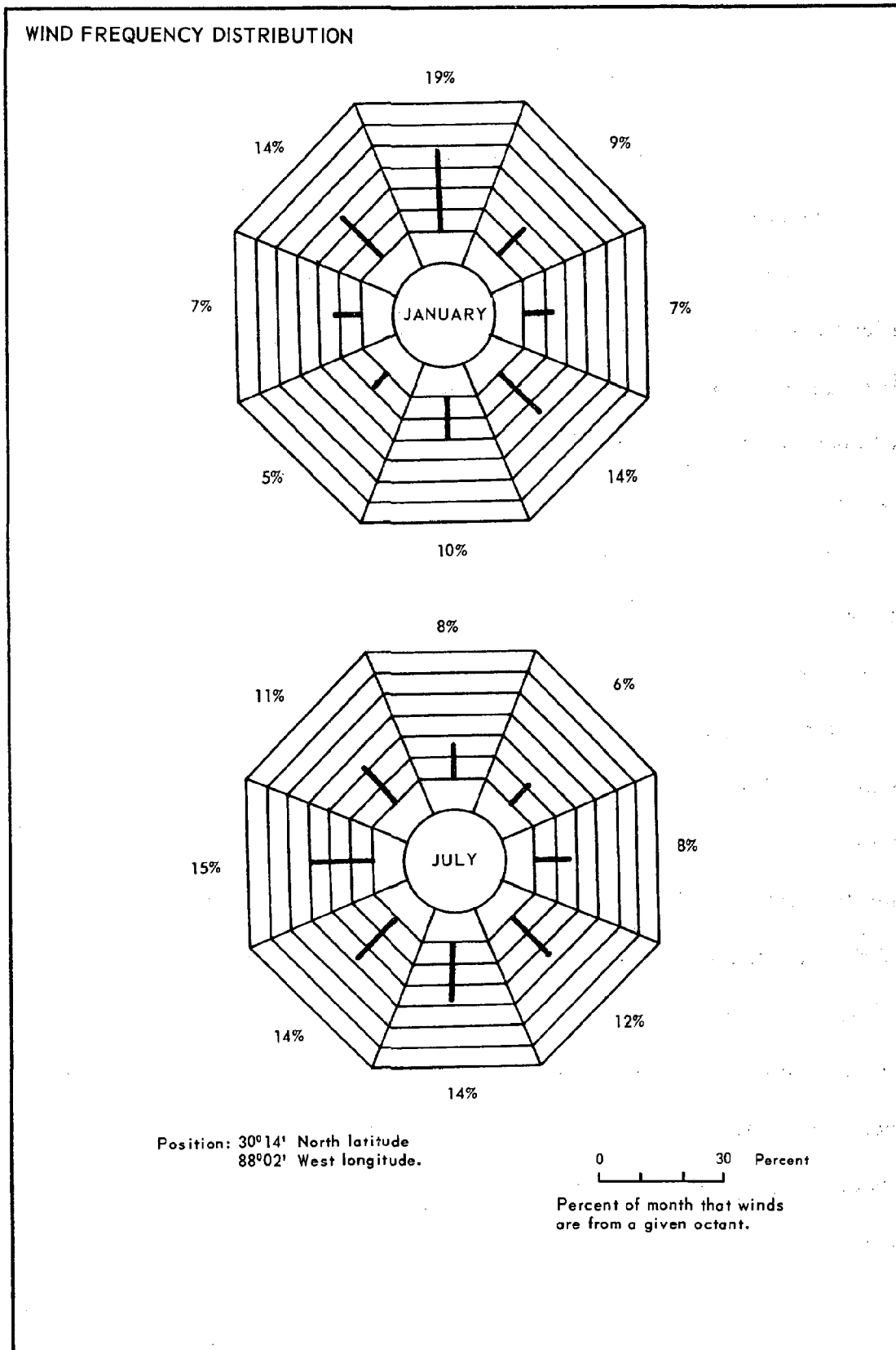
Figure 29. --Wind roses for coastal Alabama, January and July.
