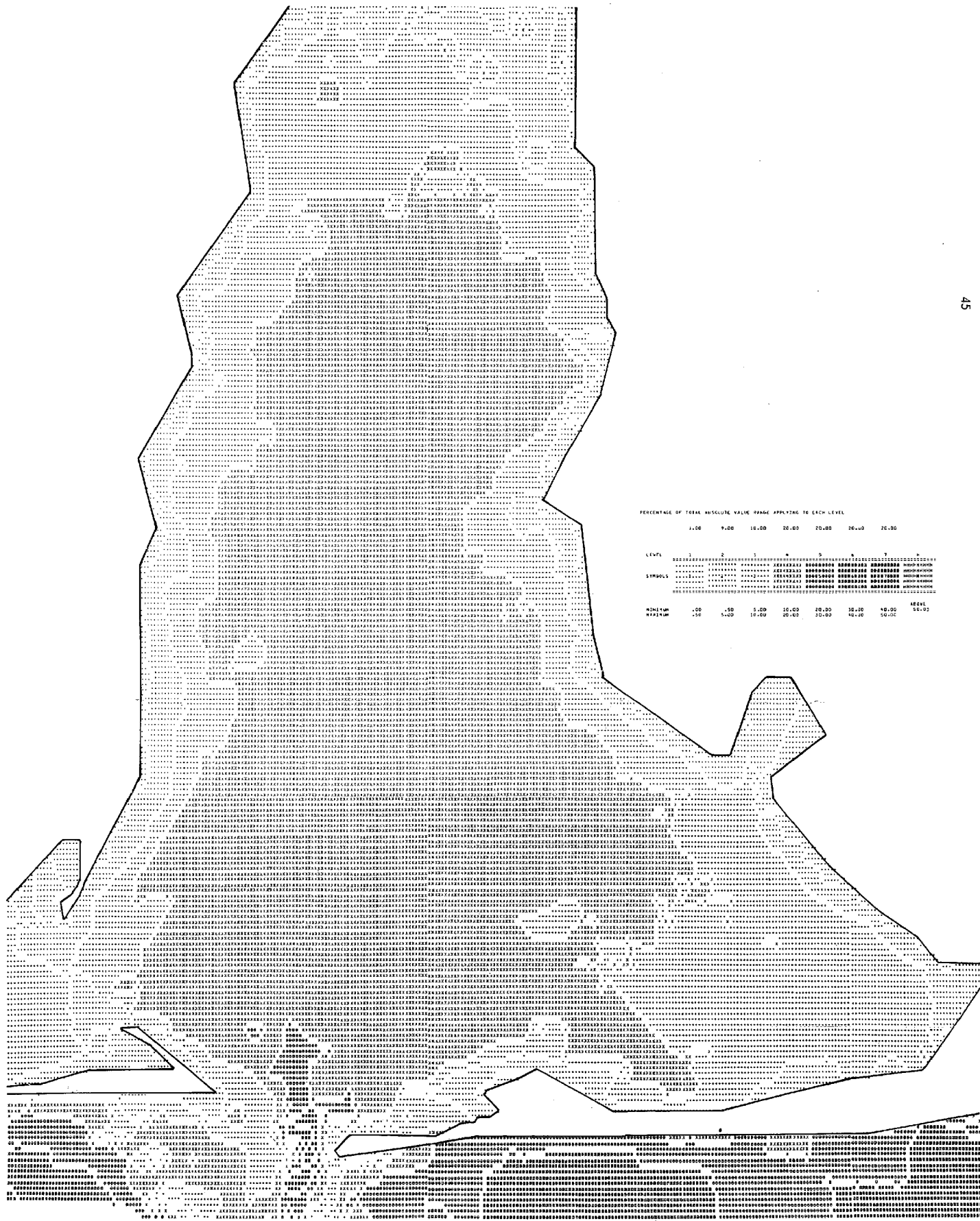
Figure 12. Mobile Bay bathymetry 1852
