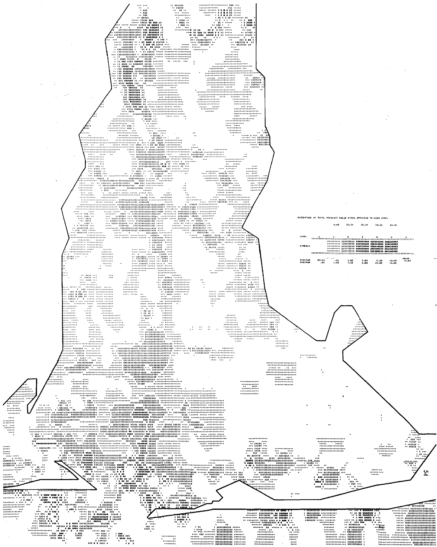
Figure 19. Areas of deposition in Mobile Bay 1920-1973
