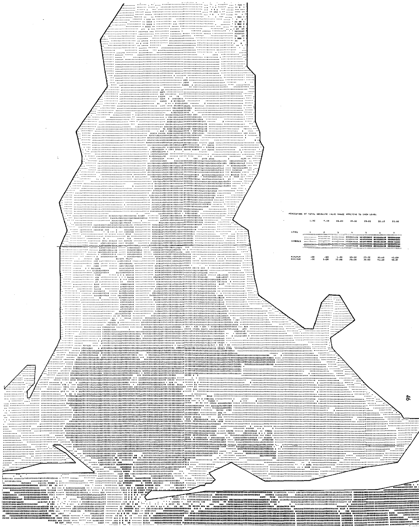
Figure 13. Mobile Bay bathymetry 1920
