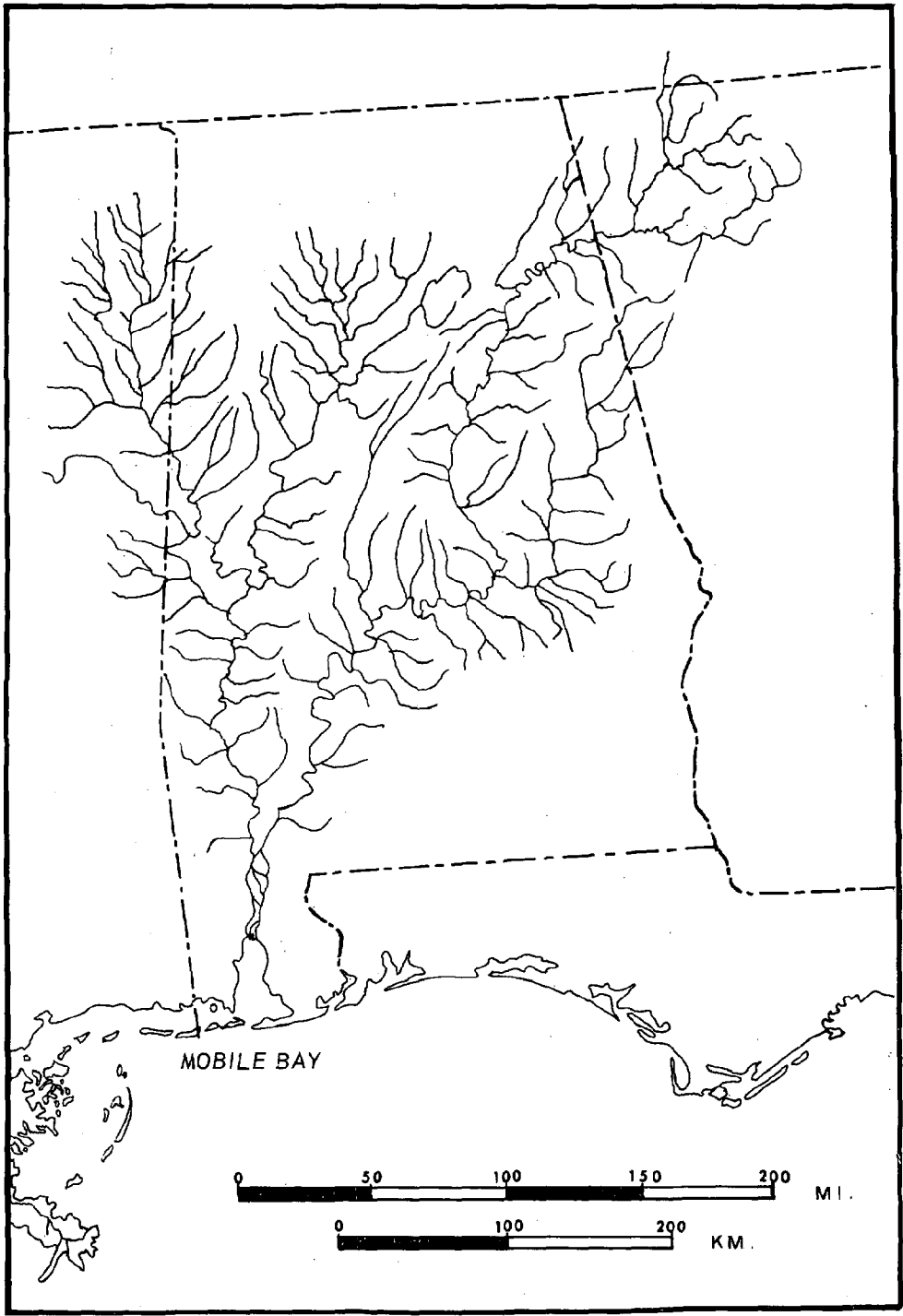
Figure 3.--Mobile River drainage basin.
