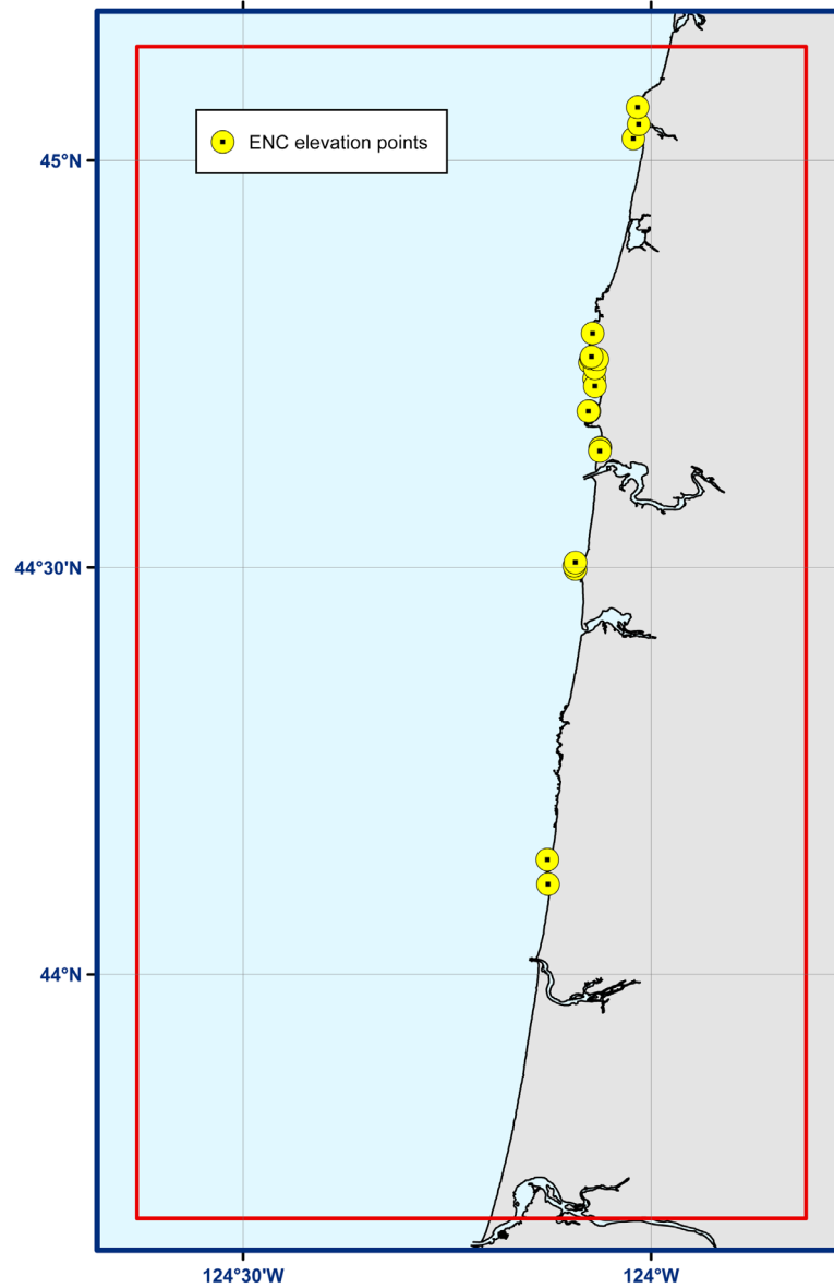
Figure 20. The spatial coverage of the extracted ENC land elevation data.
