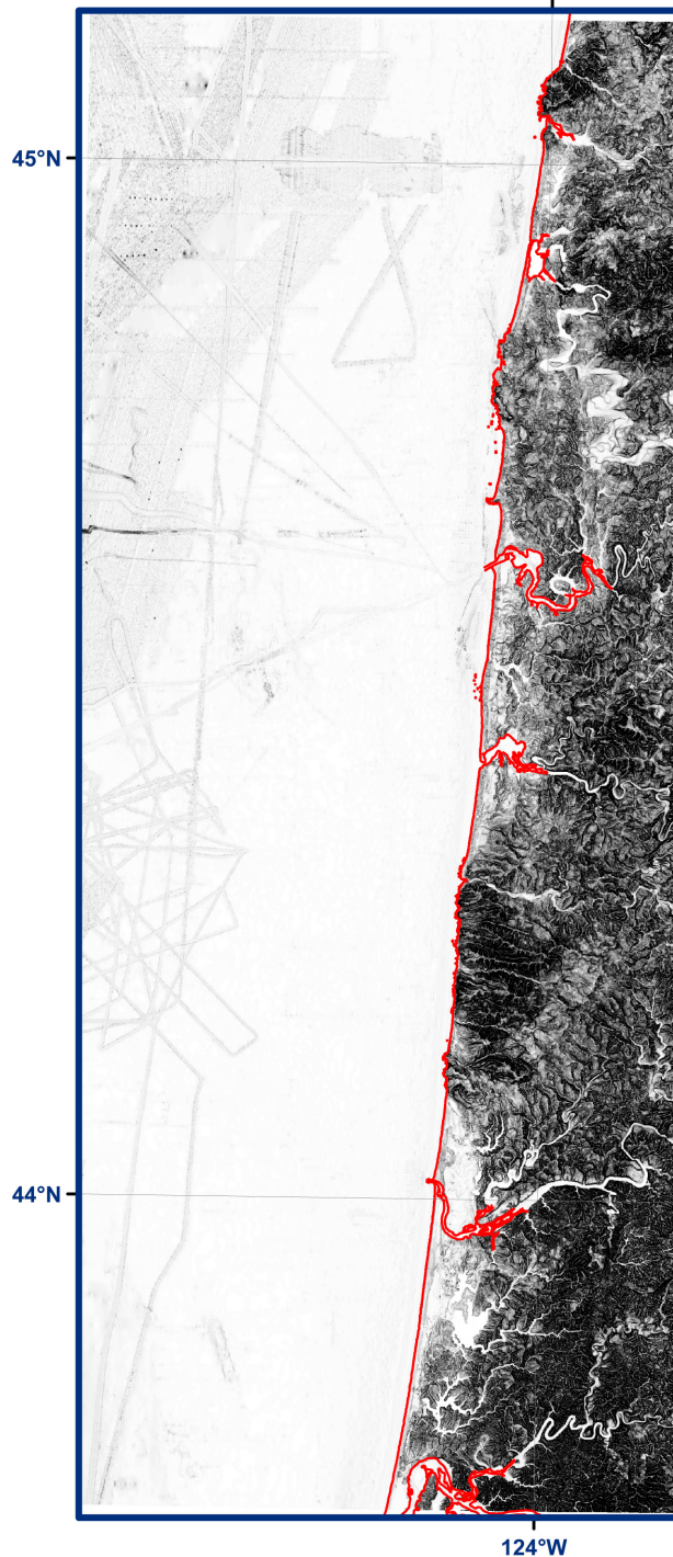
Figure 28. Slope map of the Central Oregon Coast DEM. Flat-lying slopes are white; dark shading denotes steep slopes; Central Oregon Coast coastline in red.
