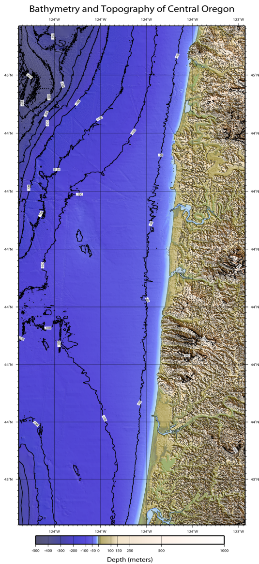
Figure 1. Shaded-relief image of the Central Oregon Coast DEM. Contour interval is 50 meters in water and 100 meters on land. Image is in Mercator projection.
