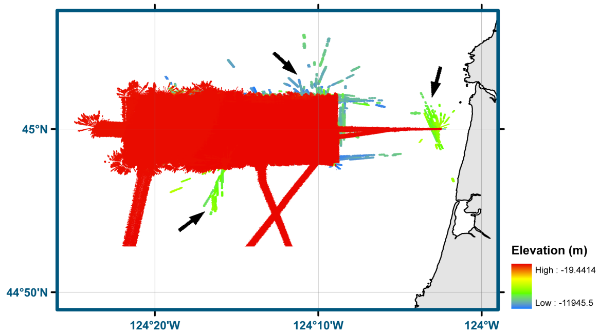
Figure 11. The CNTL04RR multibeam survey located offshore of Cascade Head and Siletz Bay colored by elevation. The arrows point to areas where elevations were incorrect by hundreds of meters. These values were deleted.
