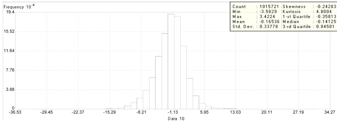
Figure 21. Histogram of the difference between one post-Katrina JALBTCX coastal bathymetric–topographic LiDAR survey (438,007 points) and the Biloxi DEM.
