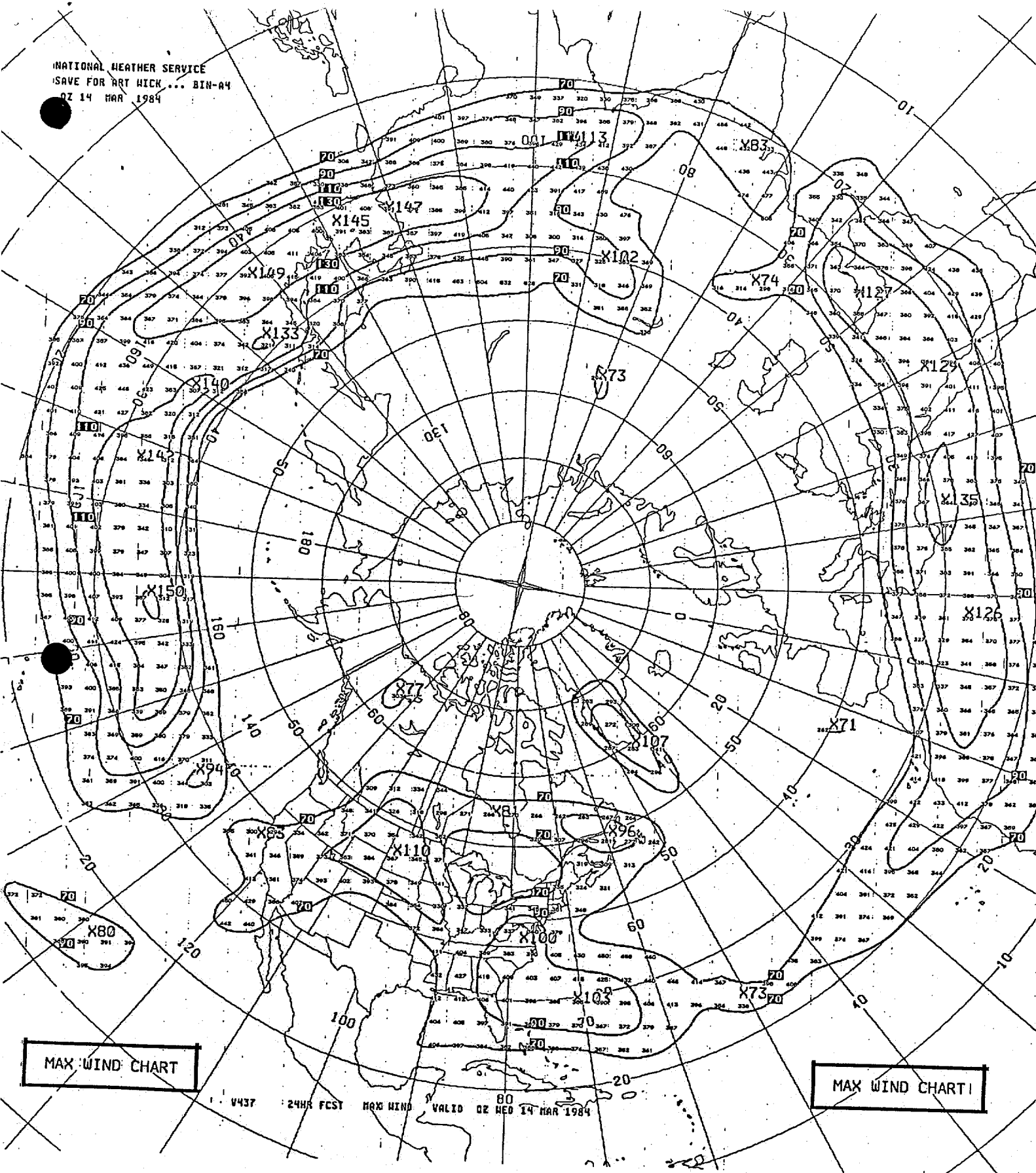
Figure 8. 24 hour forecast of maximum wind speed and level valid
