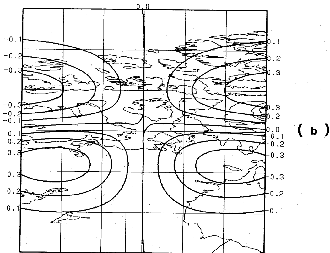
Figure 1. The uv forecast error correlation as computed from (a) the exact spherical distance s_0 , (b) Schlatter's distance approximation s_2 and (c) the currently operational distance approximation s_3 at latitude 70^\circ\text{N} . The contour interval is 0.1.
