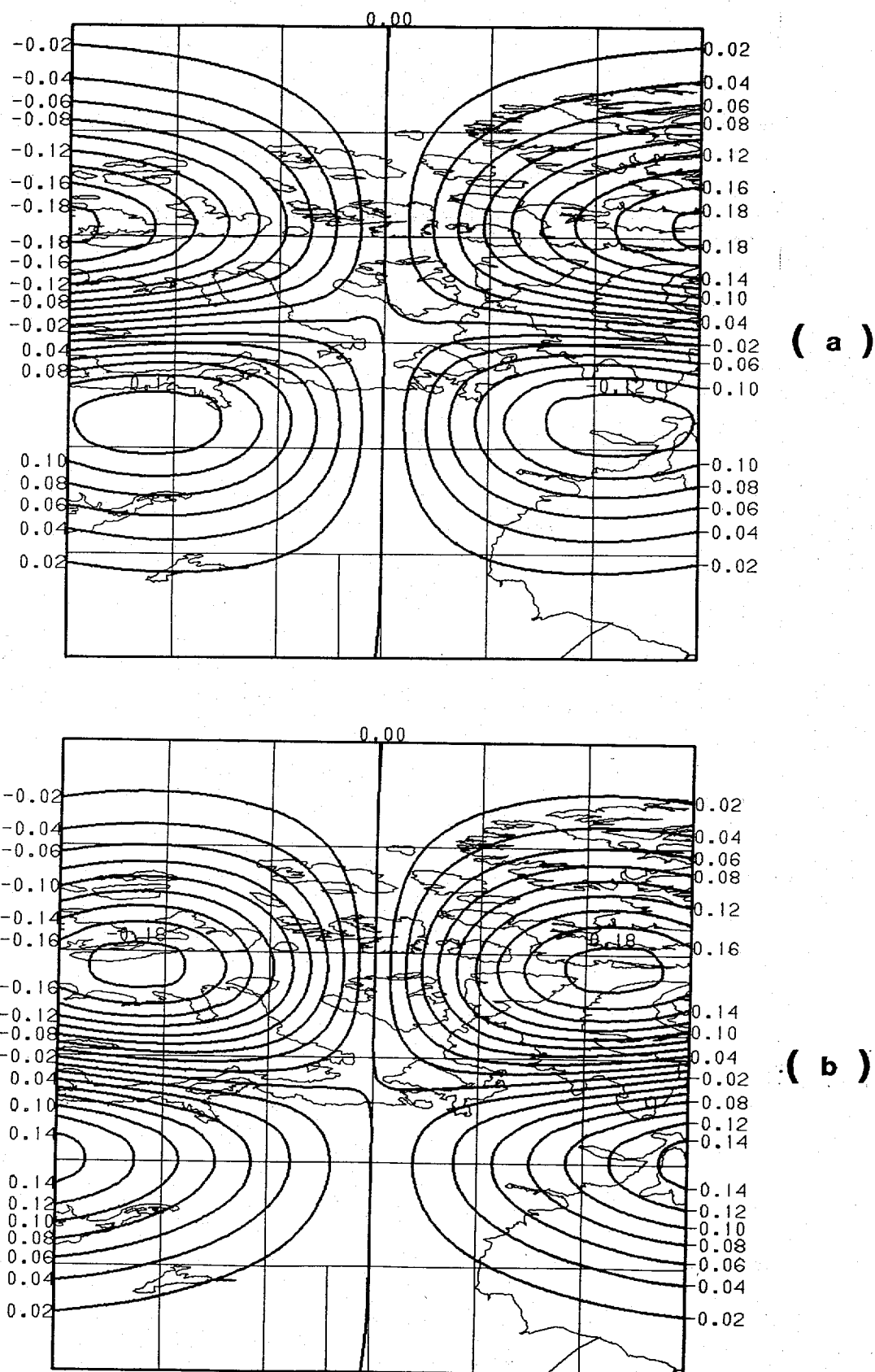
Figure 2. Error fields portraying the difference between uv forecast error correlations computed from the exact spherical distance s_0 and (a) Schlatter's distance approximation s_2 and (b) the currently operational distance approximation s_3 . The contour interval is 0.02.
