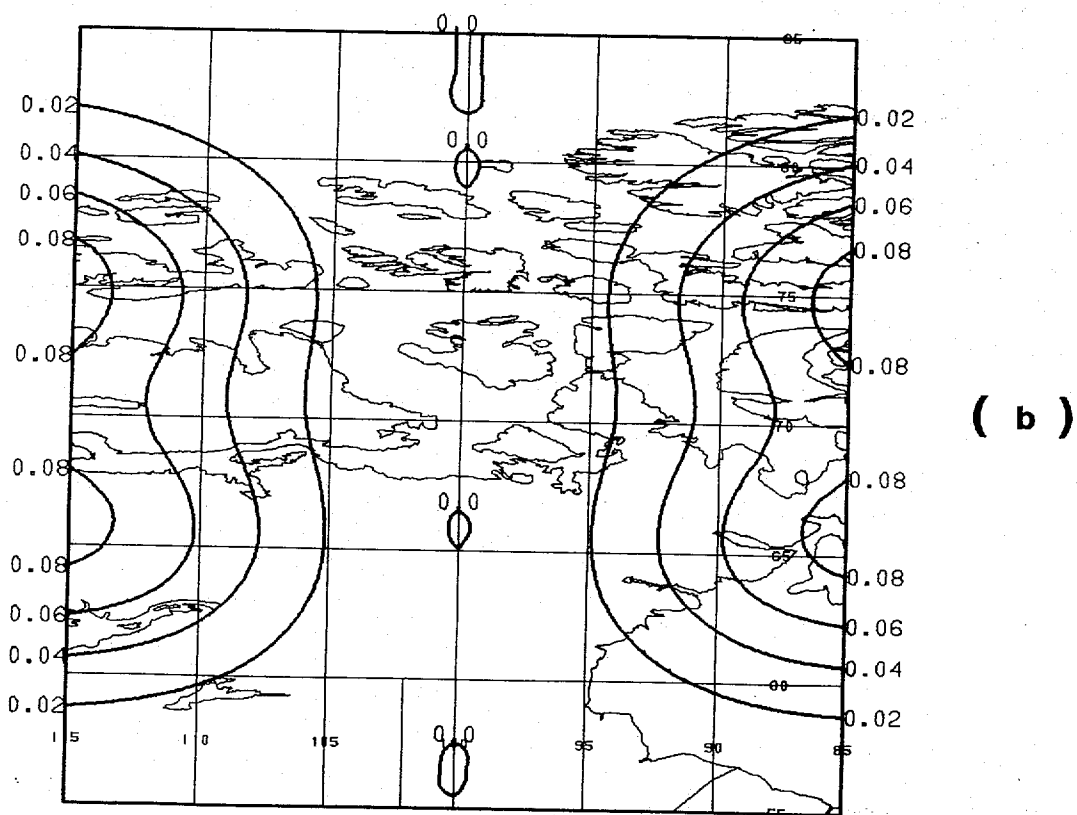
Figure 4. Error fields portraying the difference between uv forecast error correlations computed from the exact spherical distance s_0 and (a) Schlatter's distance approximation s_2 and (b) the currently operational distance approximation s_3 . The contour interval is 0.02.
