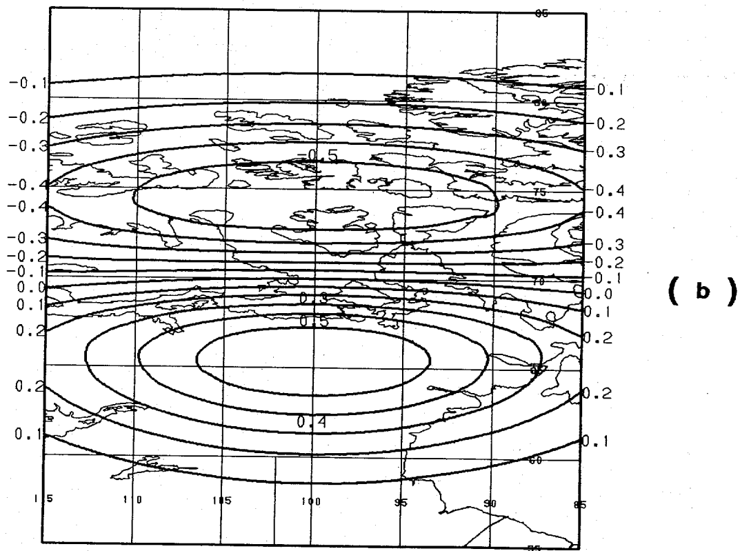
Figure 3. The uz forecast error correlation as computed from (a) the exact spherical distance s_0 , (b) Schlatter's distance approximation s_2 and (c) the currently operational distance approximation s_3 at latitude 70^\circ\text{N} . The contour interval is 0.1.
