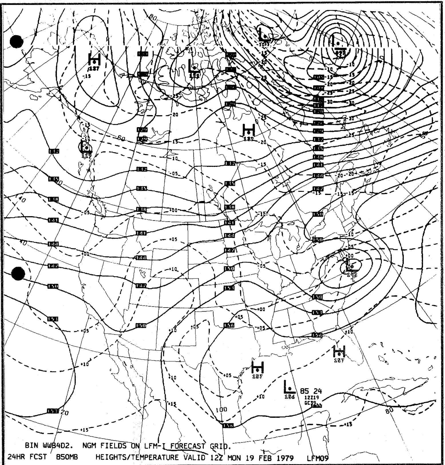
Fig. 3 24-h forecasts for Experiment 1 valid at 12 GMT 19 February 1979: 850-mb height (solid line; units: dekameters; contour interval: 3 dekameters) and 850-mb temperature (dashed line; units: °C; contour interval: 5°C).
