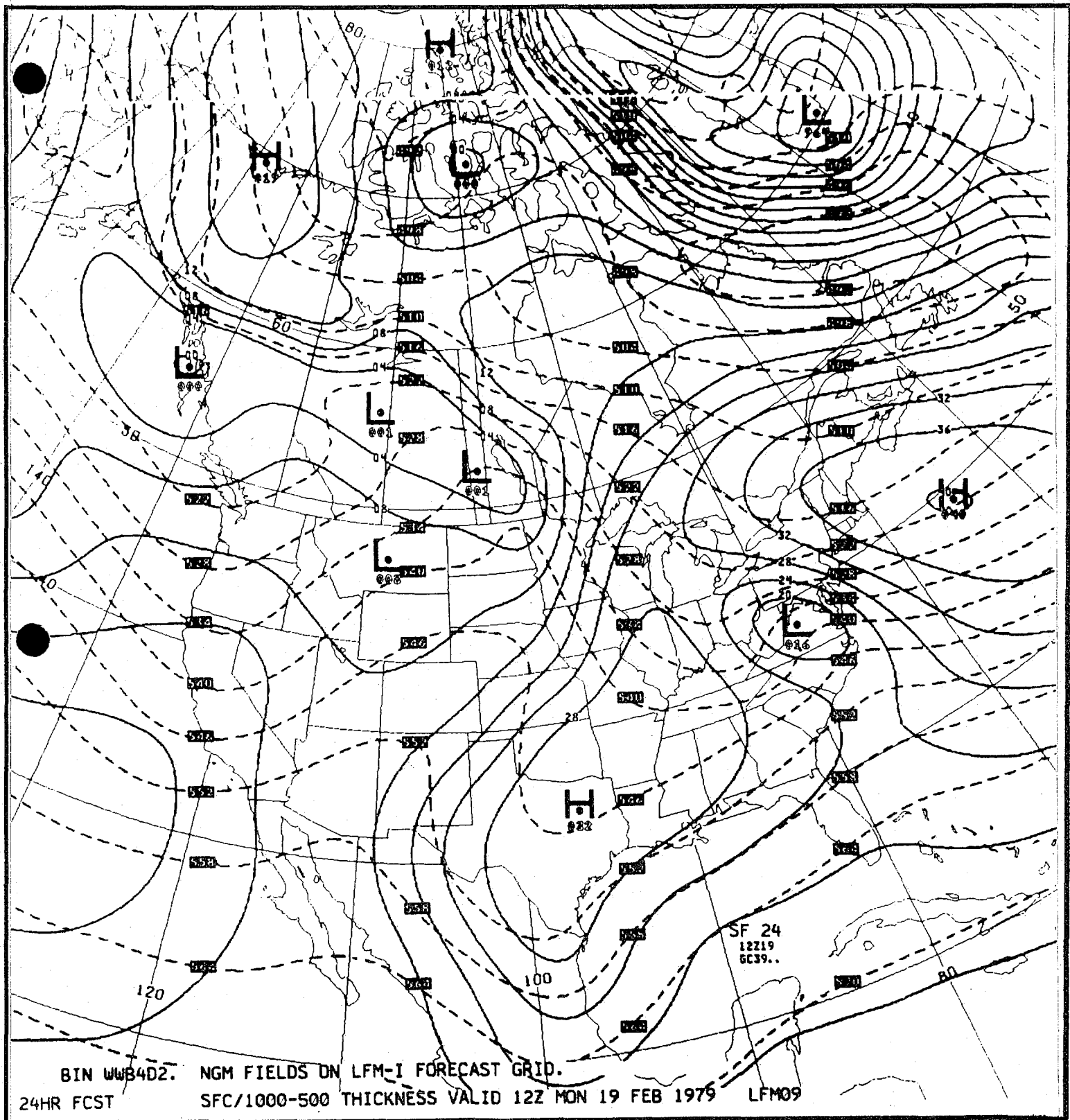
Fig. 5 The influence of the feedback of latent heating: 24-h forecasts for Experiment 3 valid at 12 GMT 19 February 1979 for mean-sea-level pressure (solid line; contour interval: 4 mb), and 1000/500-mb thickness (dashed line; units: dekameters; contour interval: 6 dekameters).
