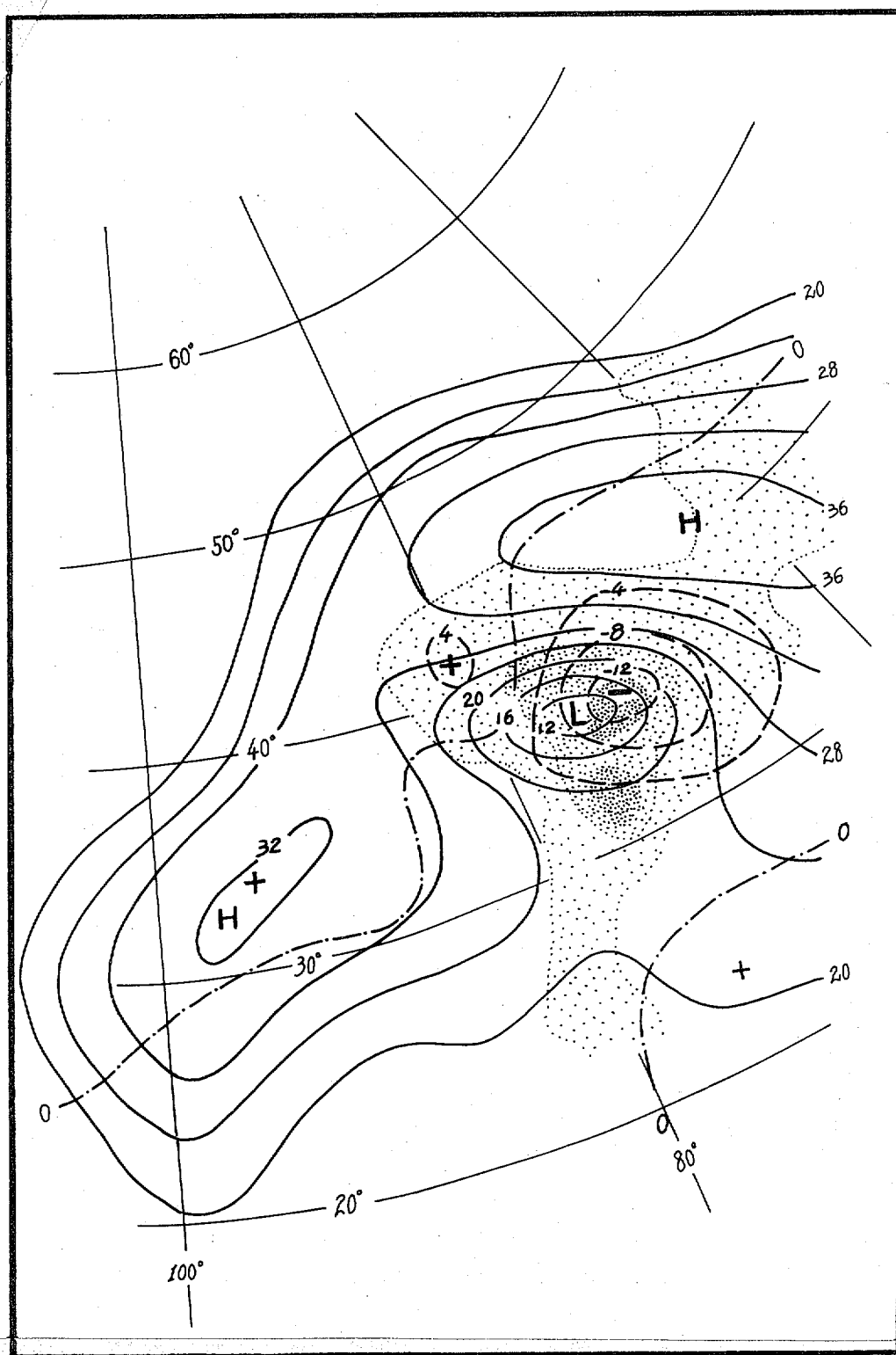
Fig. 6 The influence of the feedback of latent heating on mean-sea-level pressure: 24-h forecast of mean-sea-level pressure (solid line; contour interval: 4 mb) valid at 12 GMT 19 February 1979; difference of the 24-h forecast of mean-sea-level pressure (Experiment 1 minus Experiment 3; dashed line; units: mb; contour interval: 4 mb); and 12-24 h precipitation area (stippled) as forecast in Experiment 1.
