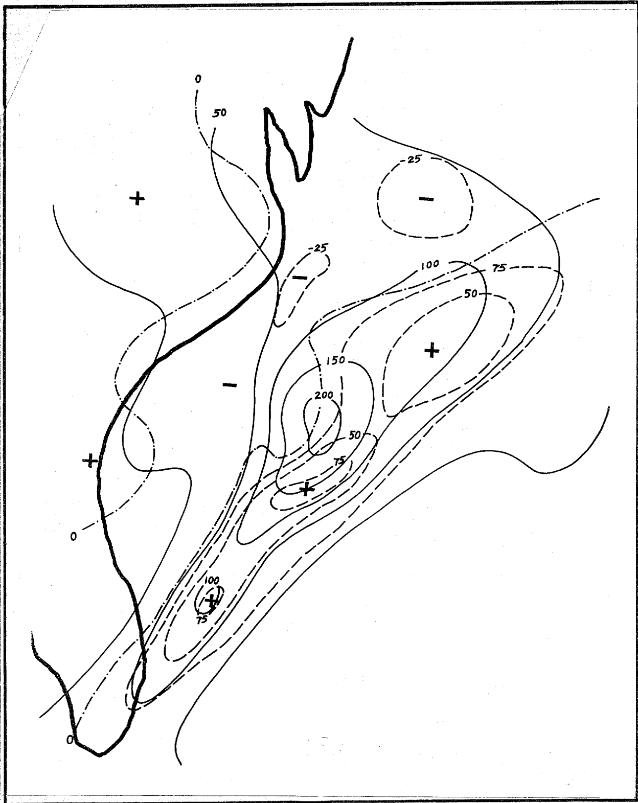
Fig. 4 The influence of moist convective adjustment: accumulated precipitation from 12-24 h (solid line; units: 0.01 inches; contour interval: 0.50 inches) for Experiment 2 ending at 12 GMT 19 February 1979, and the difference (Experiment 2 minus Experiment 1; dashed line; units: 0.01 inches; contour interval: 0.25 inches) for 12-24 h accumulated precipitation ending at 12 GMT 19 February 1979.
