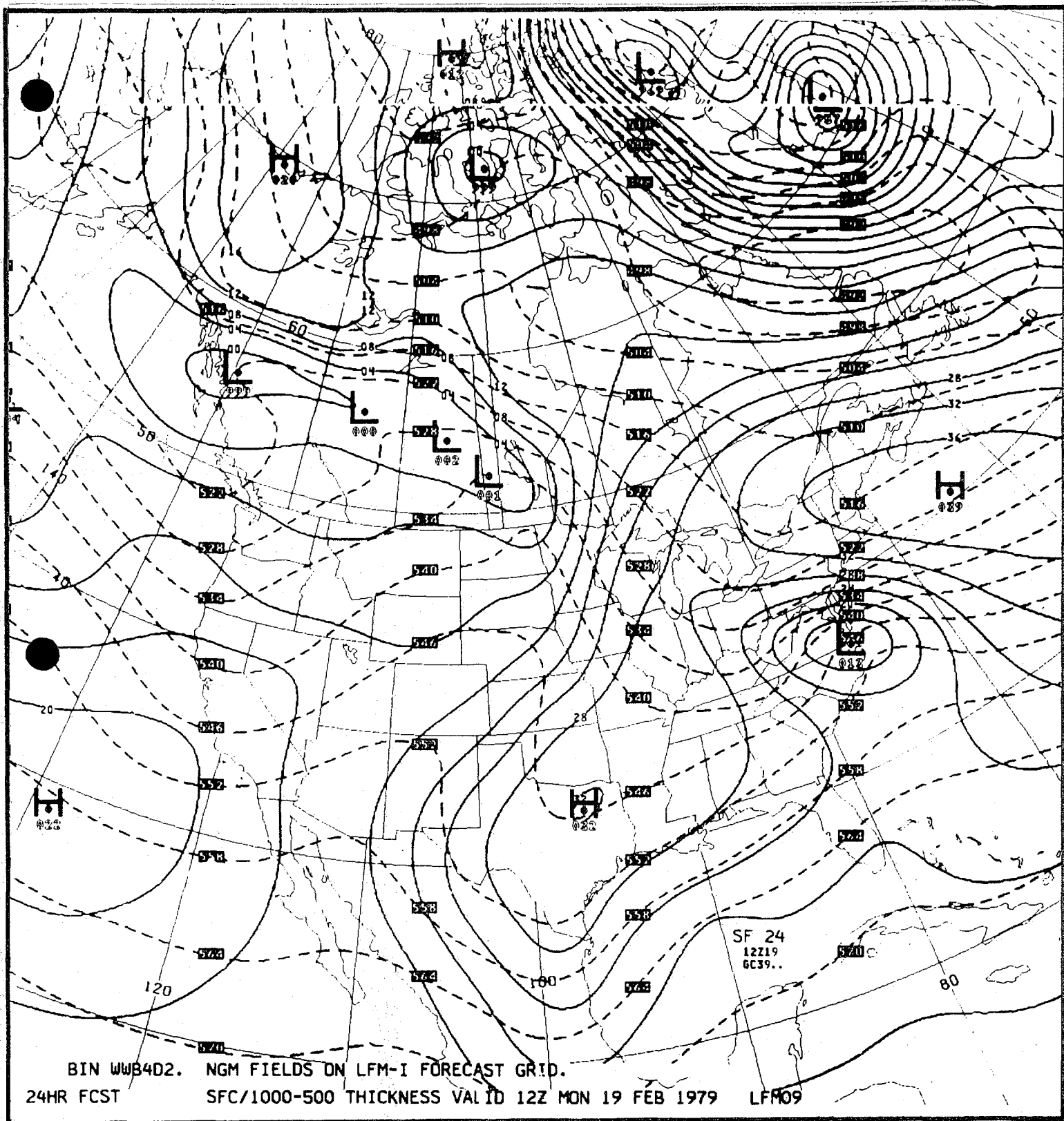
Fig. 8 The influence of moisture flux from the ocean: 24-h forecasts of mean-sea-level pressure (solid line; contour interval: 4 mb) and 1000/500-mb thickness (dashed line; units: dekameters; contour interval: 6 dekameters) for Experiment 5 valid at 12 GMT 19 February 1979.
