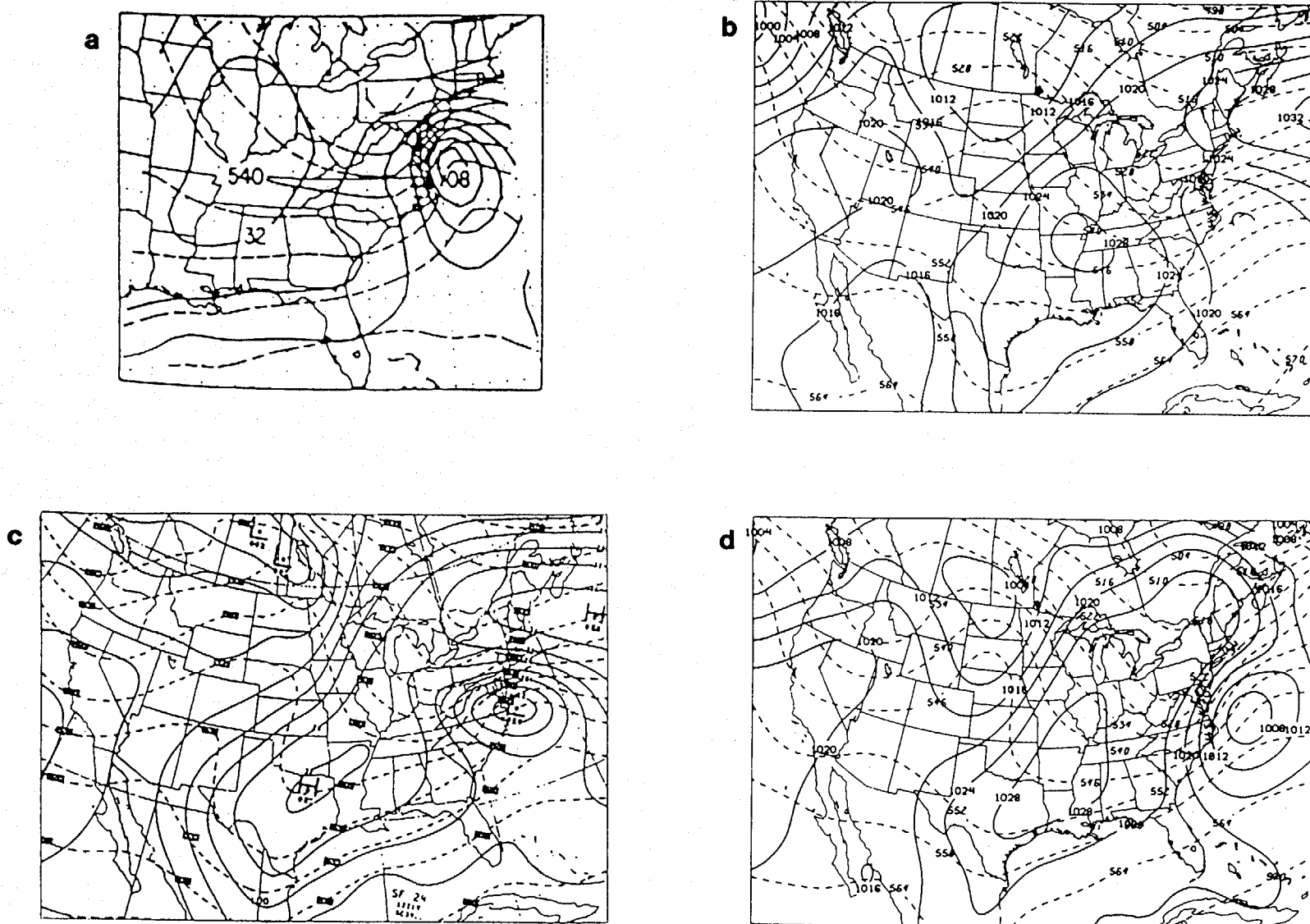
Fig. 14 Surface pressure (mb) and 1000-500 mb thickness (dam) at 12Z 19 February 1979: (a) objective analysis from Bosart and Lin (1984); (b) LFM forecast; (c) NGM forecast from Guo and Hoke (1985); (d) isentropic forecast.
