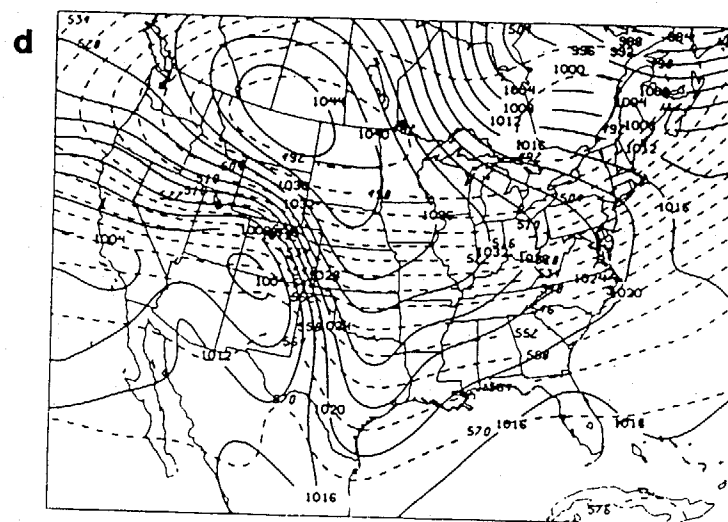
Fig. 13 Same as Fig. 12 except verifying at 12Z 24 December 1983.
