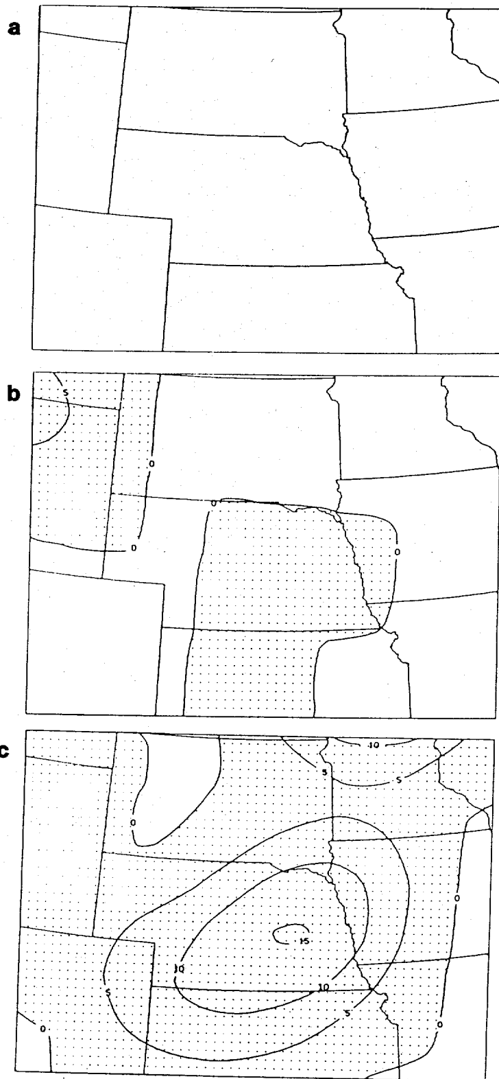
Fig. 9 Forecasts of cumulative precipitation (0.01 inches) for 12-hour period ending 00Z 29 September 1983: (a) LFM; (b) NGM; (c) isentropic model.
