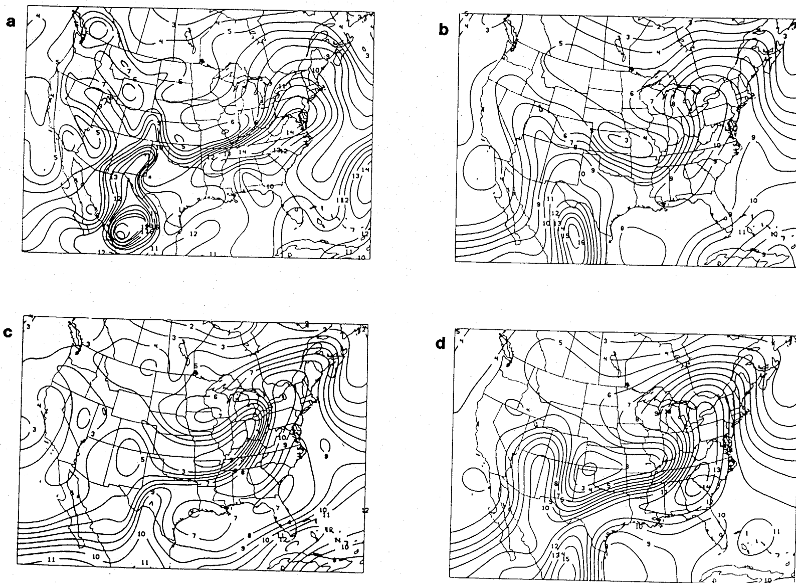
Fig. 6 The 850 mb specific humidity (g/kg) at 00Z 1 June 1985: (a) LFM analysis; (b) LFM forecast; (c) NGM forecast; (d) isentropic forecast.
