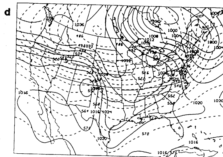
Fig. 12 Surface pressure (mb) and 1000-500 mb thickness (dam) at 12Z 23 December 1983: (a) LFM analysis; (b) LFM forecast; (c) NGM forecast; (d) isentropic forecast.
