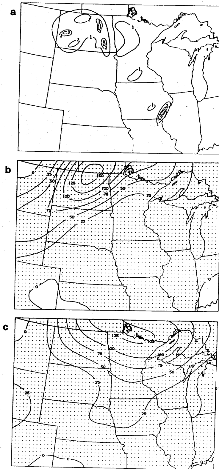
Fig. 4 Cumulative precipitation for 24-hour period ending 00Z 12 May 1985: (a) observed amounts exceeding one inch; (b) LFM forecast; (c) isentropic forecast. Units are inches in (a) and 0.01 inches in (b) and (c).
