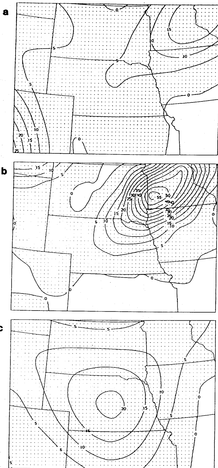
Fig. 10 Same as Fig. 9 except for 12-hour period ending 12Z 29 September 1983.
