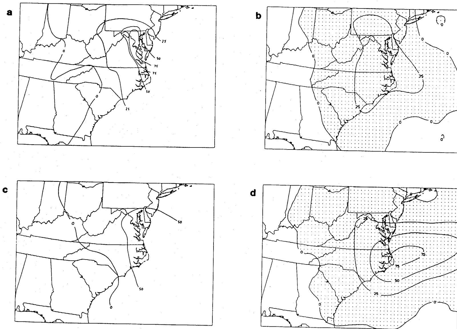
Fig. 15 Cumulative precipitation (0.01 inches) for 12-hour period ending 12Z 19 February 1979: (a) observed; (b) LFM forecast; (c) NGM forecast from Guo and Hoke (1985); (d) isentropic forecast.
