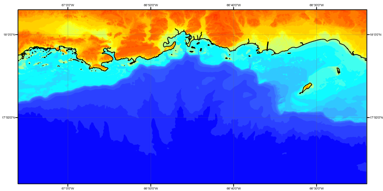
Figure 14e. Color image of the 1/3 arc-second Ponce DEM. Elevations colored as in Figure 14b; combined coastline in black.
