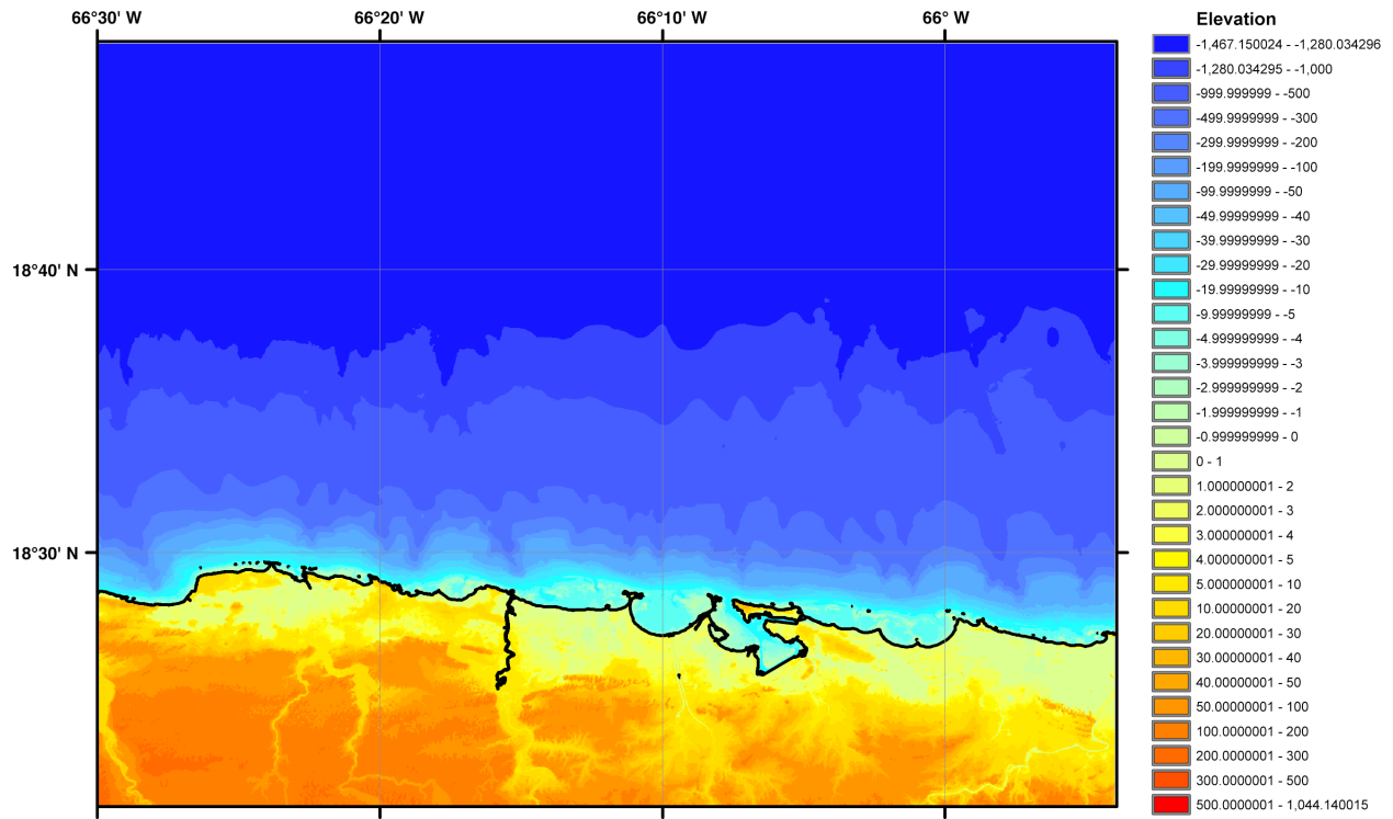
Figure 14b. Color image of the 1/3 arc-second San Juan DEM. Combined coastline in black.
