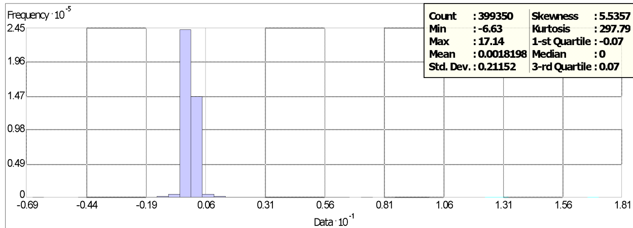
Figure 15. Histogram of the differences between one SHOALS bathymetric LiDAR survey and the Arcibo DEM.
