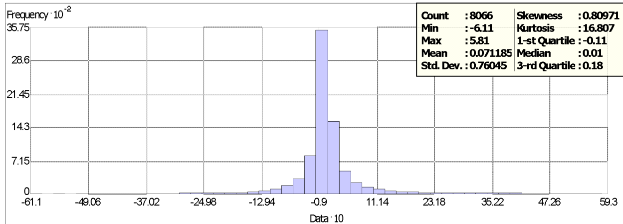
Figure 11. Histogram of the differences between NOS hydrographic survey H09491 (Bahia de Jobos, south coast) and the 3 arc-second pre-surfaced bathymetric grid. Large discrepancies between survey soundings and the pre-surface bathymetric grid occur where multiple, closely spaced points, in regions with significant relief, contribute to one cell value.
