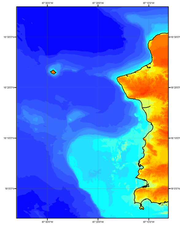
Figure 14f. Color image of the 1/3 arc-second Mayagüez DEM. Elevations colored as in Figure 14b; combined coastline in black.
