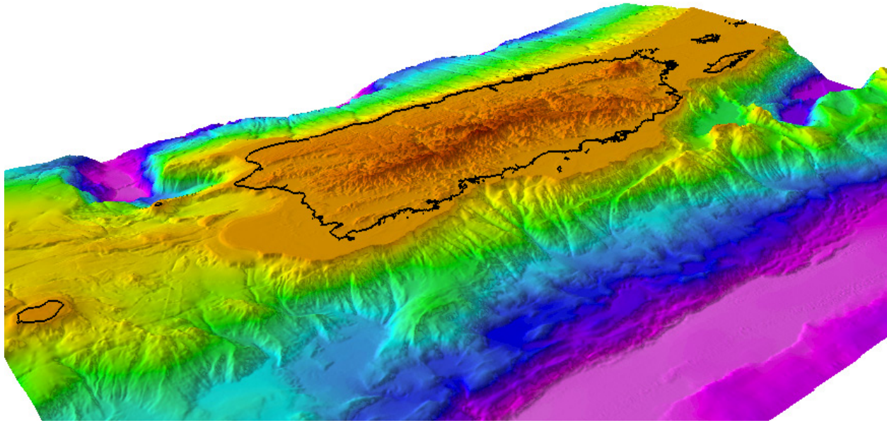
Figure 13. Perspective view of the 1 arc-second Puerto Rico DEM. Vertical exaggeration times 3; combined coastline in black.
