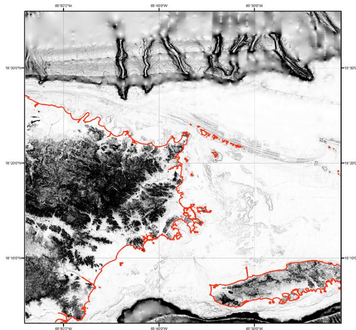
Figure 12. Slope map of the 1/3 arc-second Fajardo DEM. Flat-lying slopes are white; dark shading denotes steep slopes; combined coastline in red.
