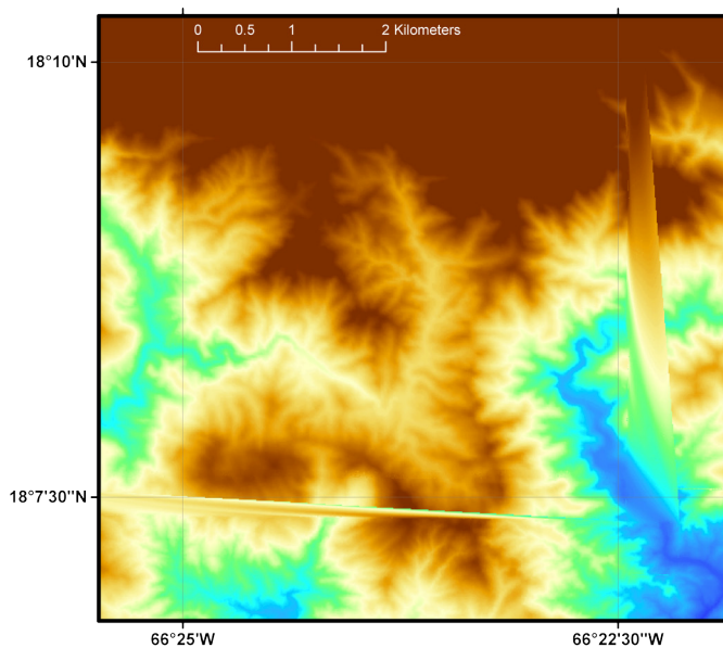
Figure 10. Detail of NED 1/3 arc-second DEM showing processing errors generated by USGS gridding algorithm.
