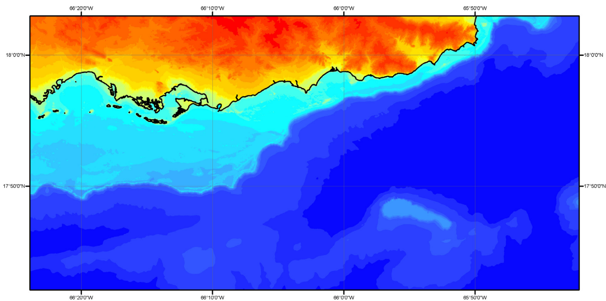
Figure 14d. Color image of the 1/3 arc-second Guayama DEM. Elevations colored as in Figure 14b; combined coastline in black.
