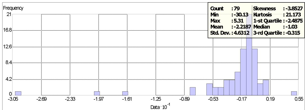
Figure 17. Histogram of the differences between NGS monuments and the Ponce DEM.
