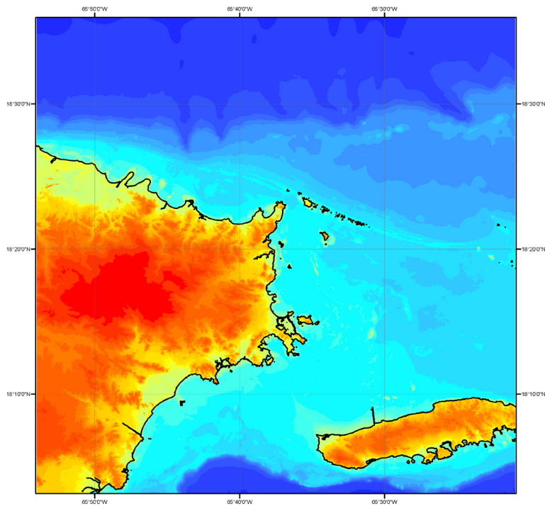
Figure 14c. Color image of the 1/3 arc-second Fajardo DEM. Elevations colored as in Figure 14b; combined coastline in black.
