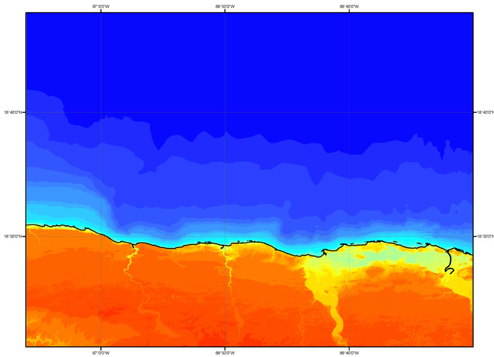
Figure 14g. Color image of the 1/3 arc-second Arecibo DEM. Elevations colored as in Figure 14b; combined coastline in black.
