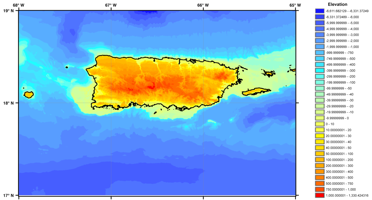
Figure 14a. Color image of the 1 arc-second Puerto Rico DEM. Combined coastline in black.
