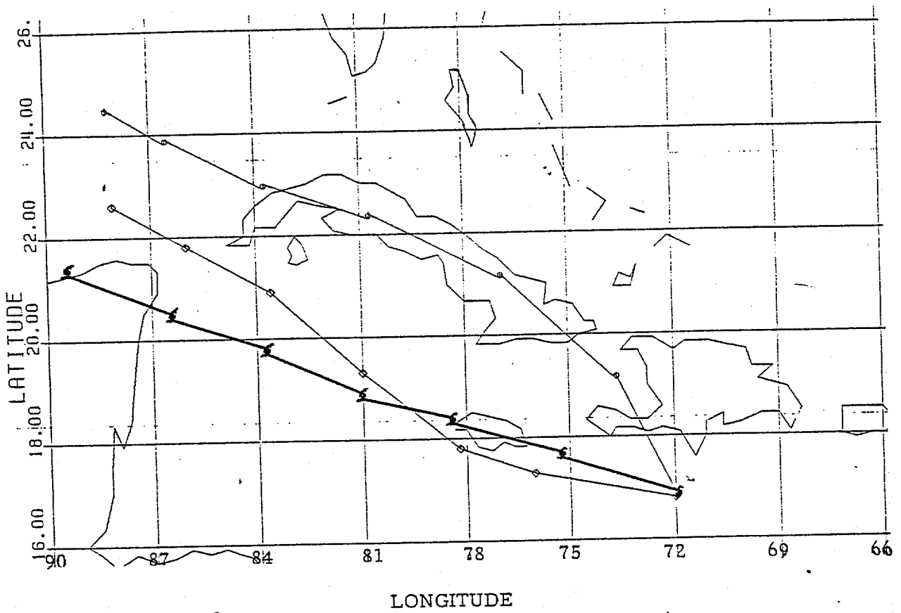
Figure 6. Gilbert 88/9/12/00z.
