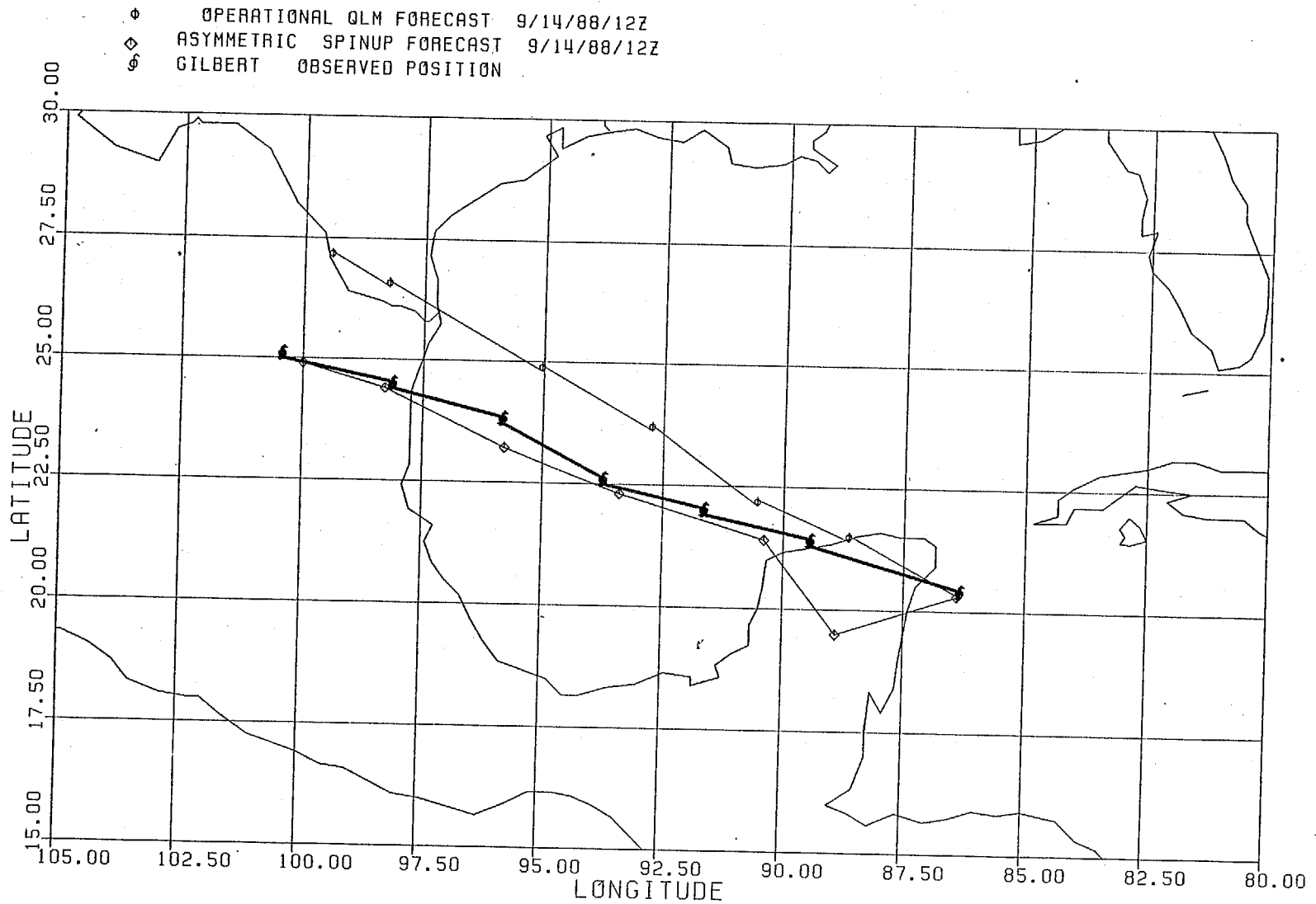
Figure 7. Gilbert 88/9/14/12z.
