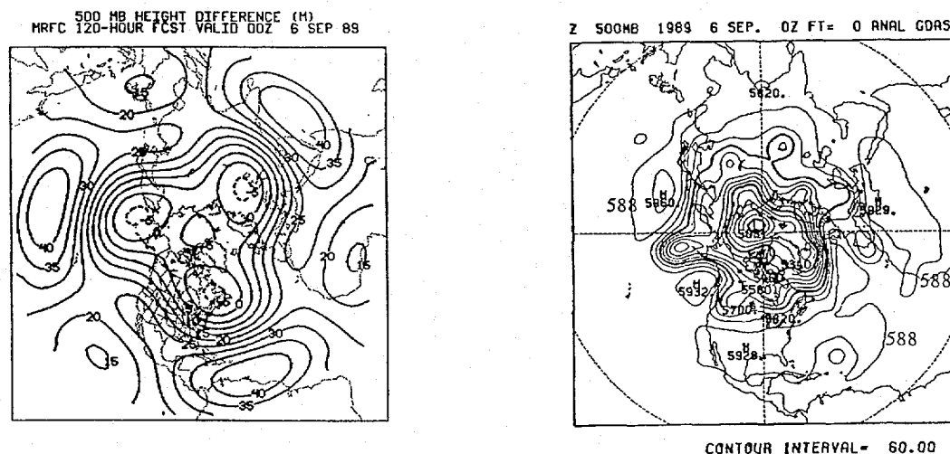
Fig 9 Difference (5m contour) between the operational and error corrected forecasts shown in Fig 8 (left) and the 500 mb operational analysis (right) valid for 6 September 89.
