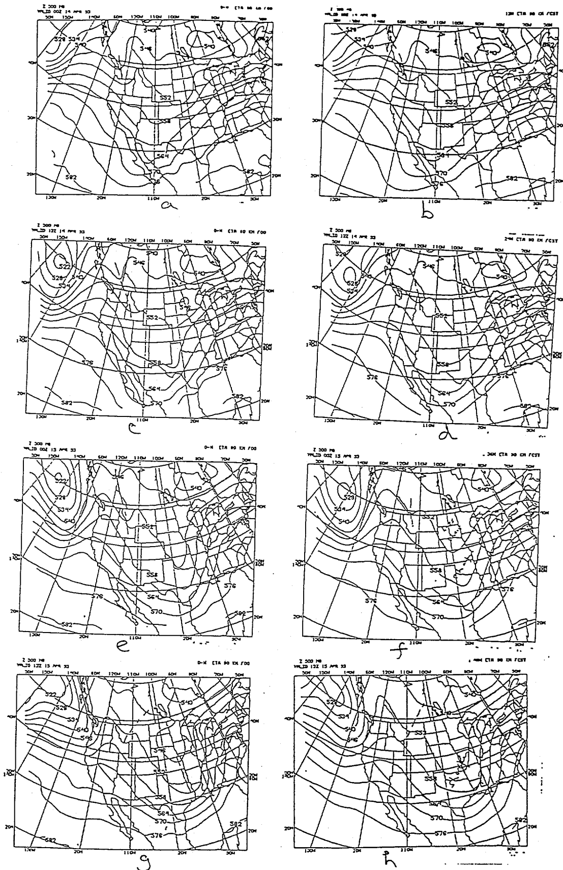
Fig. 3. Verifying and forecast height of 500 mb surface: (a) Analysis at 0000 UTC 14 April 1993, (b) 12 h forecast valid at 0000 UTC 14 April 1993, (c) analysis at 1200 UTC 14 April 1993, and (d) 24 h forecast valid at 1200 UTC 14 April 1993, (e) analysis at 0000 UTC 15 April 1993, (f) 36 h forecast valid at 0000 UTC 15 April 1993, (g) analysis at 1200 UTC 15 April 1993, and (h) 48 h forecast valid at 1200 UTC 15 April 1993. Units: tens of meters.
