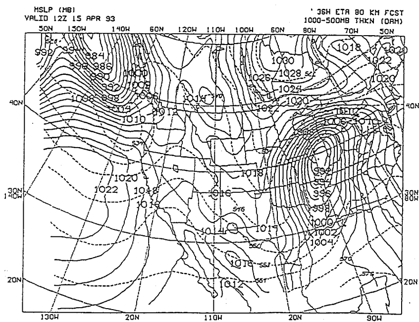
Fig. 7. Forecast mean sea level pressure at 36 h from 0000 UTC 14 April 1993. Units: mb.
