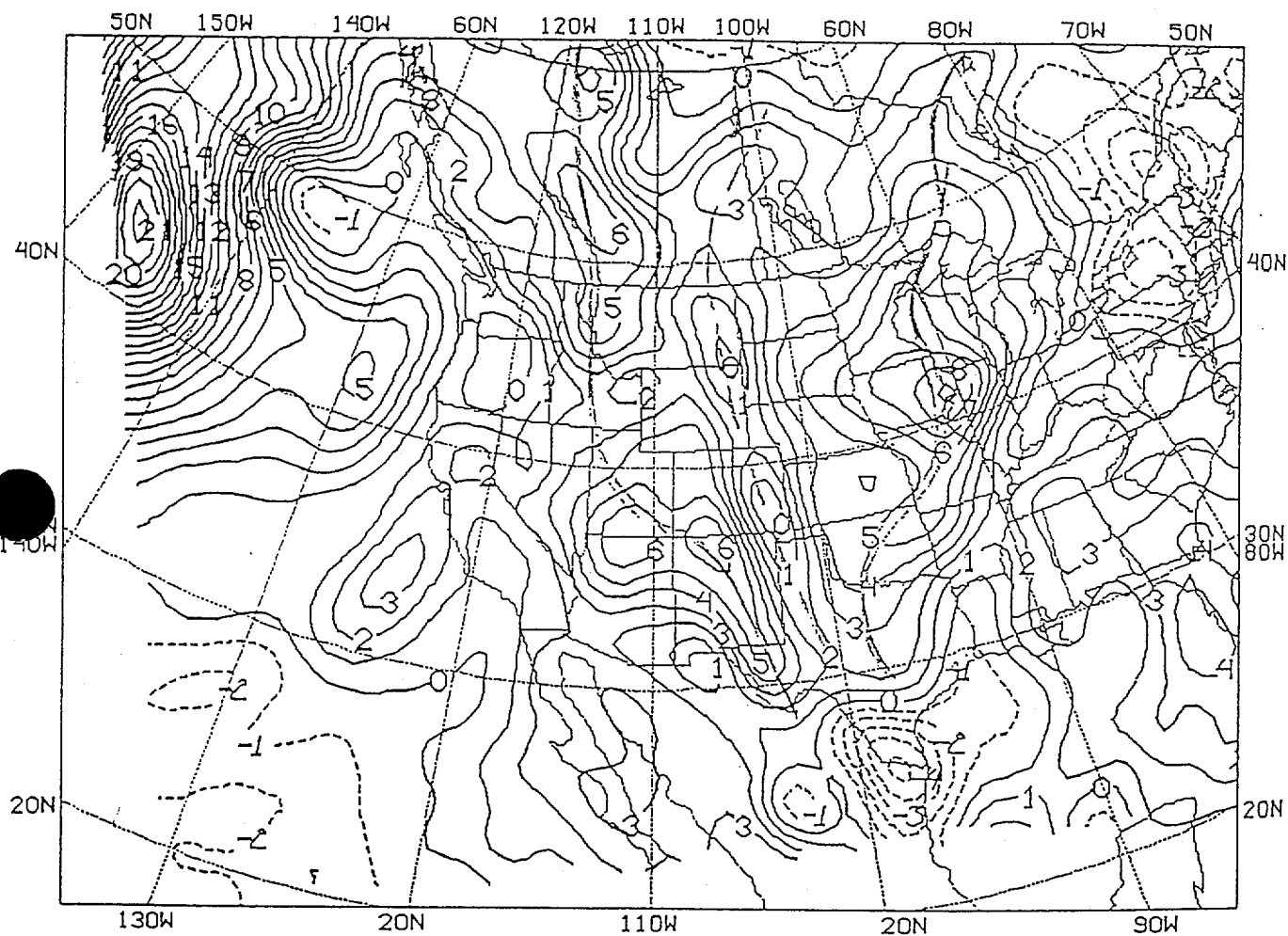
Fig. 2. Forecast mean sea level pressure errors at 48 h from 1200 UTC 13 April 1993. Units: mb.
