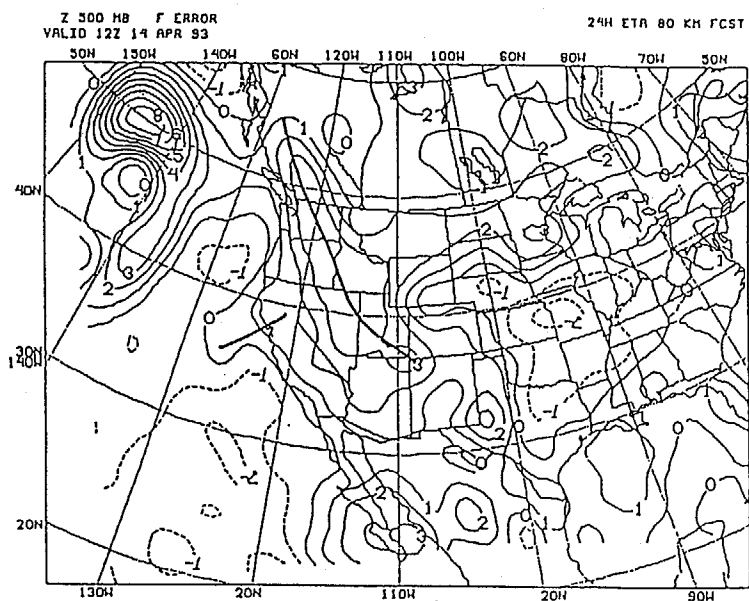
Fig. 4. Forecast errors in height of 500 mb surface at : (a) 12 h, (b) 24 h, (c) 36 h, and (d) 48h. Initial time 1200 UTC 13 April 1993. Units: tens of meters.
