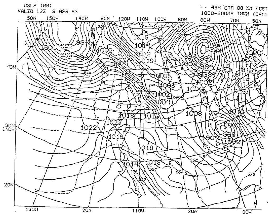
Fig. 9. Verifying and forecast Mean sea level pressure fields: (a) Analysis at 1200 UTC 9 April 1993, (b) 48 h forecast valid at 1200 UTC 9 April 1993. Units: mb.
