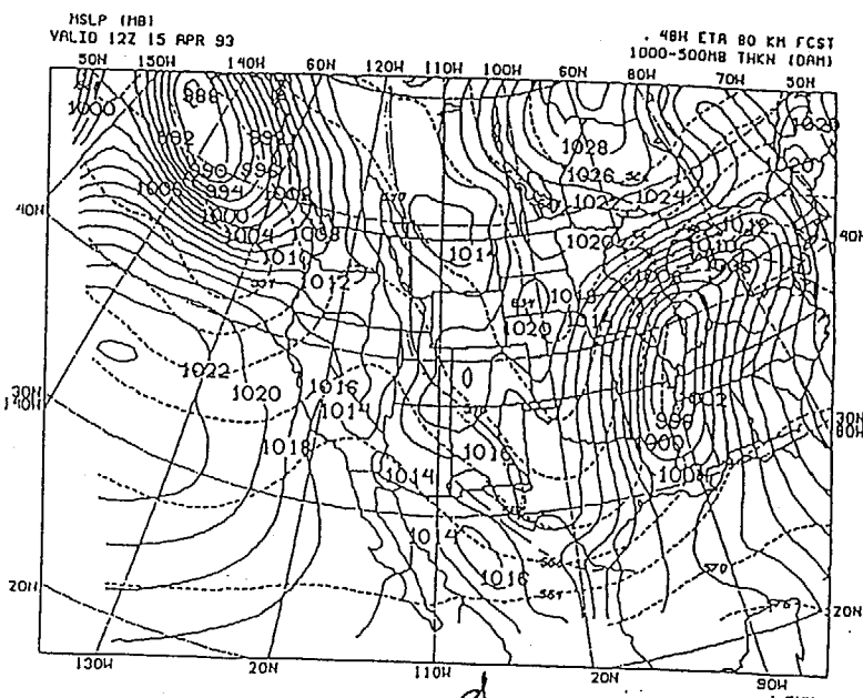
Fig. 1. Verifying and forecast Mean sea level pressure (units: mb) and 1000 - 500 mb thickness (units: tens of meters) fields: (a) Analysis at 1200 UTC 14 April 1993, (b) 24 h forecast valid at 1200 UTC 14 April 1993, (c) analysis at 1200 UTC 15 April 1993, and (d) 48 h forecast valid at 1200 UTC 15 April 1993.
