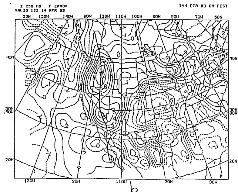
Fig. 5. Forecast errors in height of 250 mb surface at : (a) 12 h, (b) 24 h, (c) 36 h, and (d) 48h. Initial time 1200 UTC 13 April 1993. Units: tens of meters.
