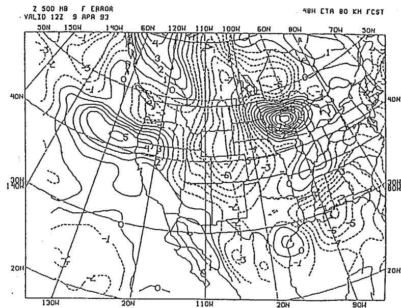
Fig. 8. Forecast errors in height of 500 mb surface at : (a) 12 h, (b) 24 h, (c) 36 h, and (d) 48h. Initial time 1200 UTC 7 April 1993. Units: tens of meters.
