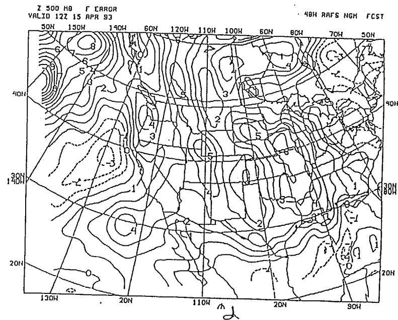
Fig. 6. Forecast errors in height of 500 mb surface in NGM at : (a) 12 h, (b) 24 h, (c) 36 h, and (d) 48h. Initial time 1200 UTC 13 April 1993. Units: tens of meters.
