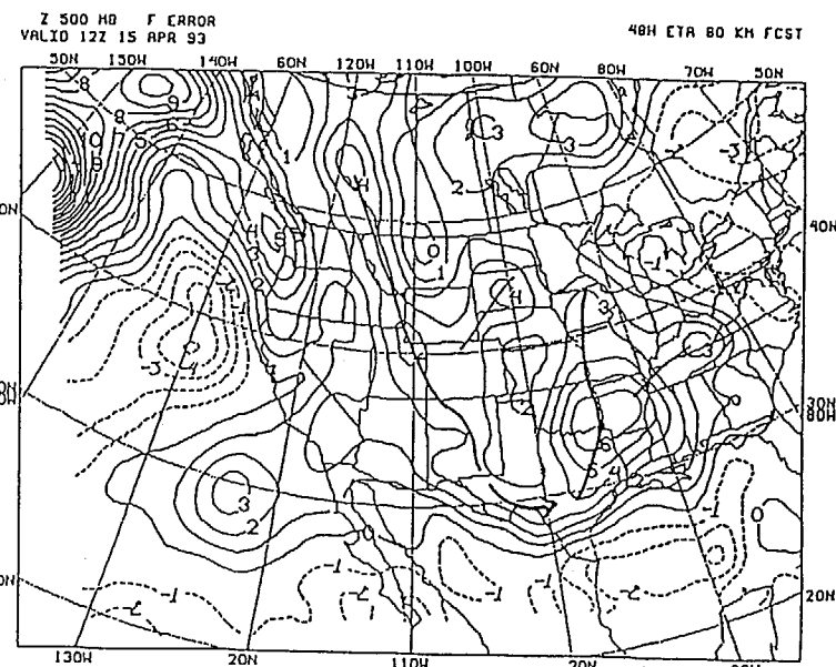
Fig. 4. Forecast errors in height of 500 mb surface at : (a) 12 h, (b) 24 h, (c) 36 h, and (d) 48h. Initial time 1200 UTC 13 April 1993. Units: tens of meters.
