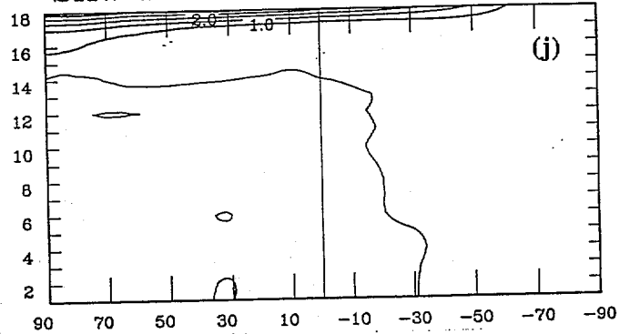
SHW FT=24 JJA 1990
