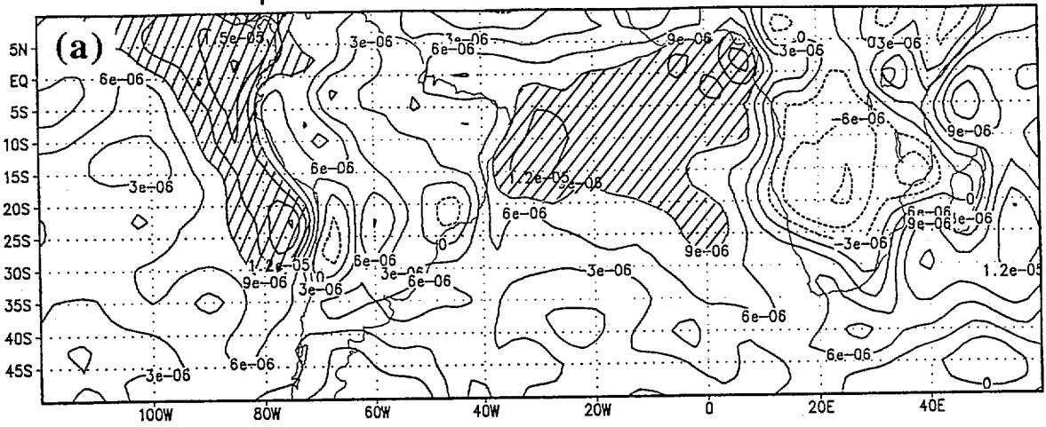
Temp Error N.H. Winter 1990 Lev=10
