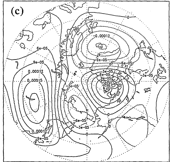
Temp Advdiv+Lnps+Vadv Winter 1990 Lev=17
