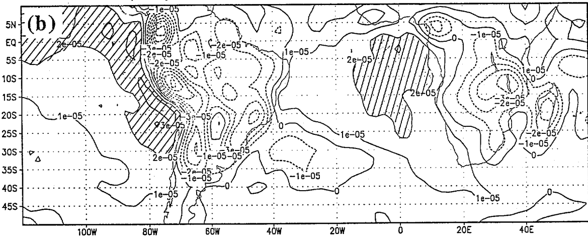
Temp Dynamics N.H. Winter 1990 Lev=10
