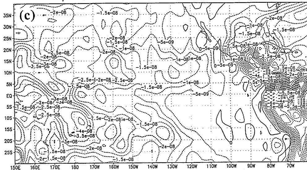
q Convection N.H. Winter 1990 Lev=5
