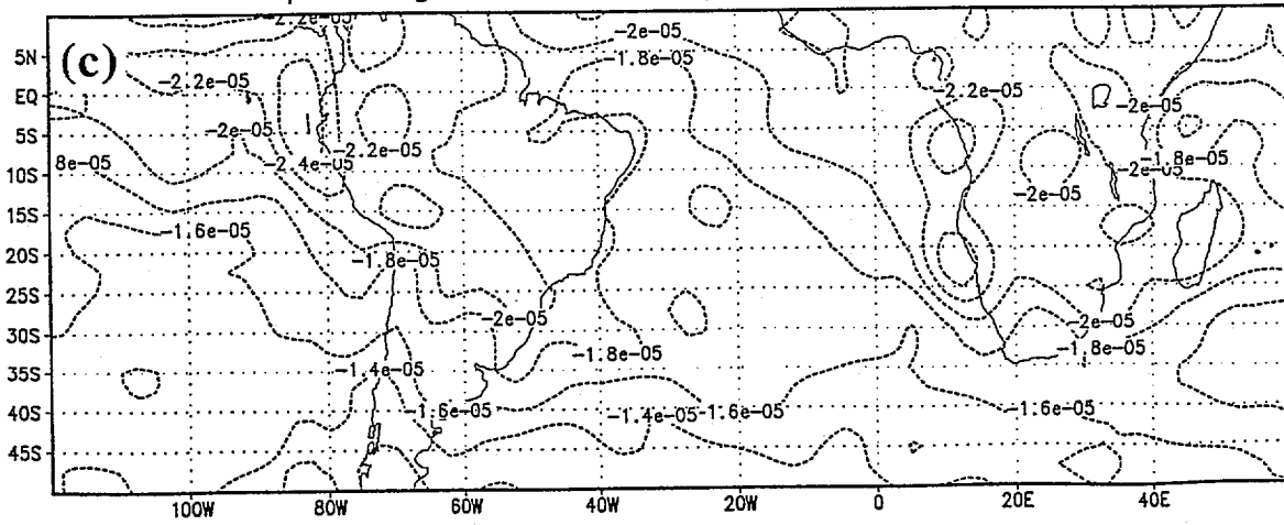
Temp Longwave N.H. Winter 1990 Lev=10
