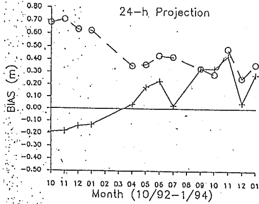
Figure 4. RMS and BIAS comparison statistics between the NOW and NOAA/WAM models for 24-, 48-, and 72-h forecasts.
