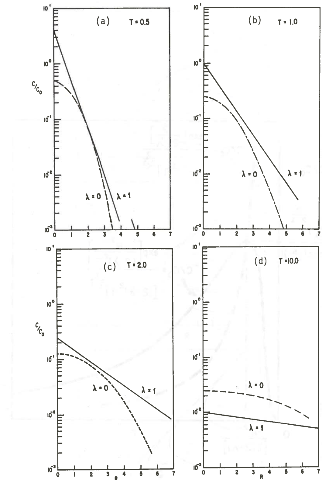
Fig. 40. Theoretical curves of particulate concentration vs. equivalent radius for \lambda = 0 and 1 at different fixed times.
