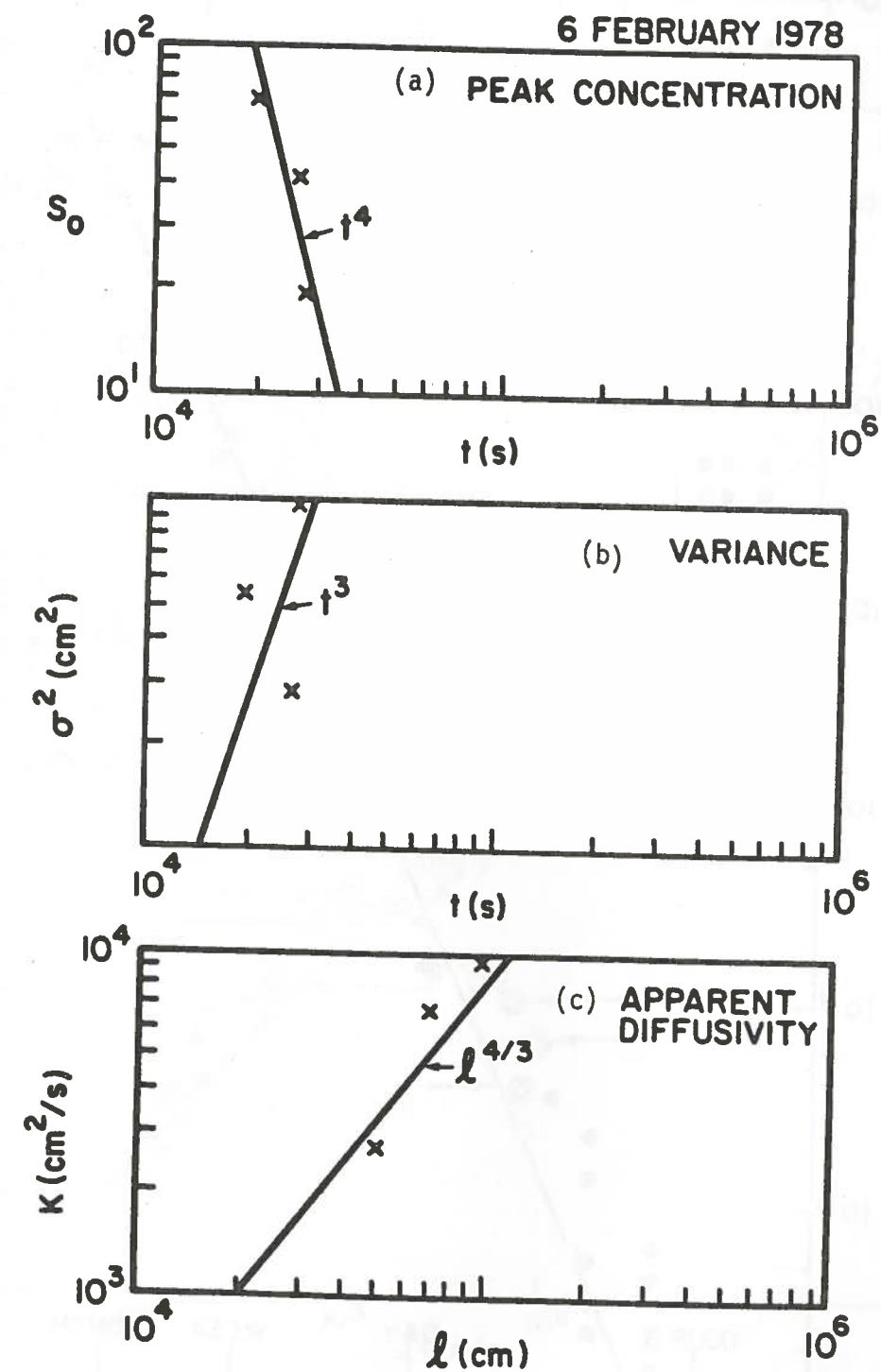
Fig. 50. (a) Peak concentration and (b) variance as a function of time, and (c) apparent diffusivity as a function of length scale for the Puerto Rico Arecibo Industrial Waste Dumping Experiment.
