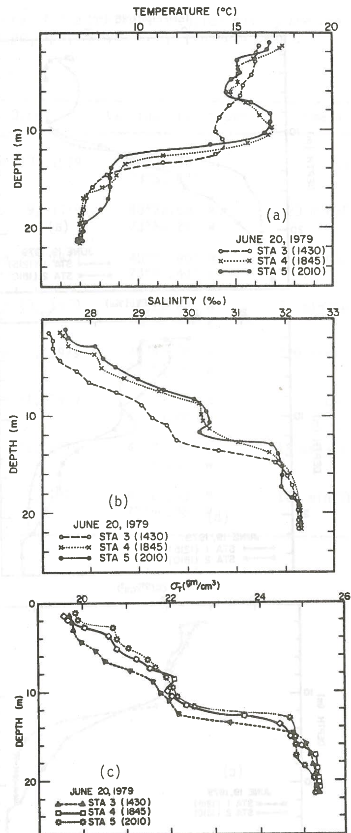
Fig. 13. Vertical profiles of (a) temperature, (b) salinity, and (c) \sigma_t for Stations 3, 4, and 5 in Fig. 11(b).
