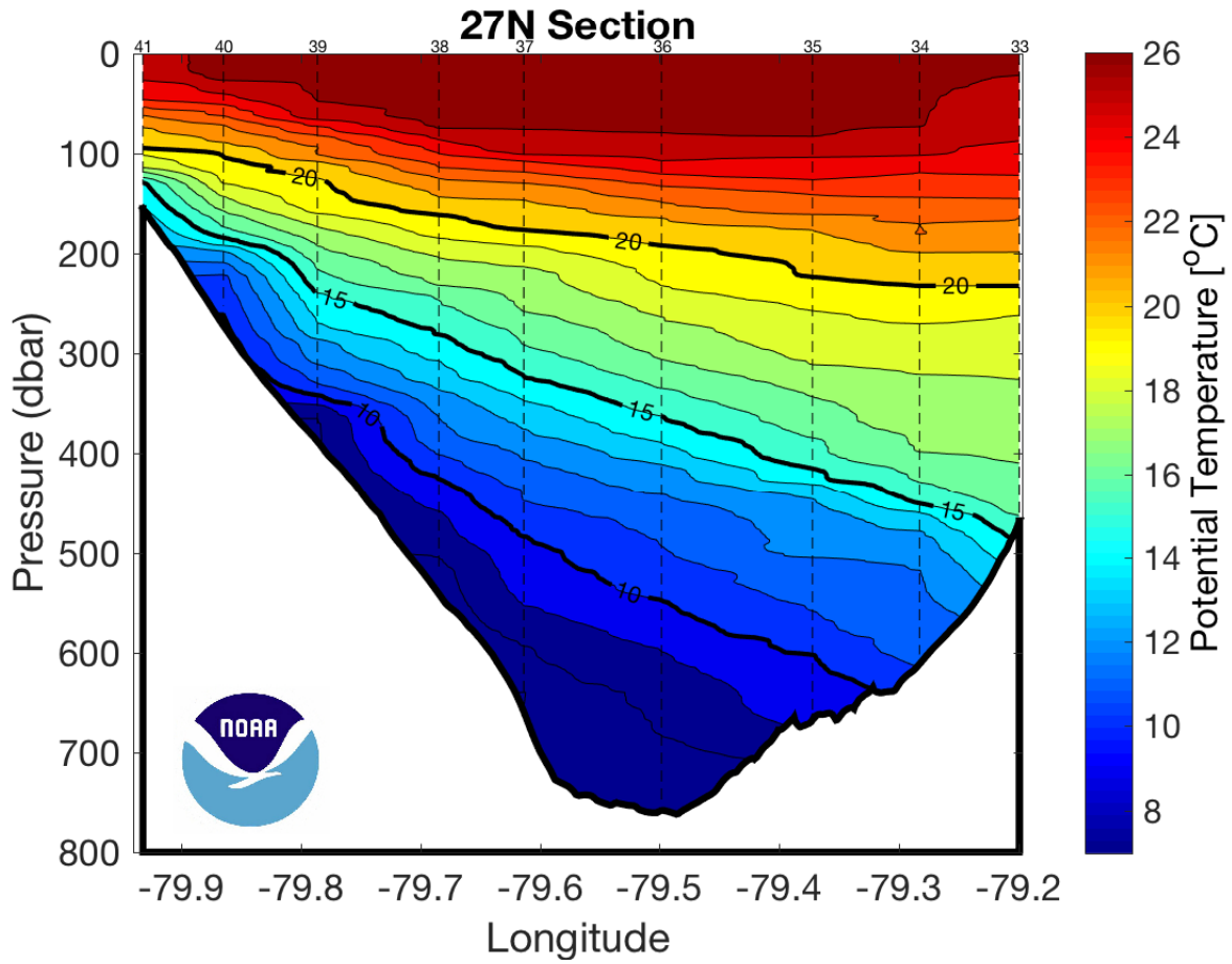
Figure 34: Potential Temperature (°C) section for the Florida Current North section. Dashed vertical lines are the CTD station locations.
