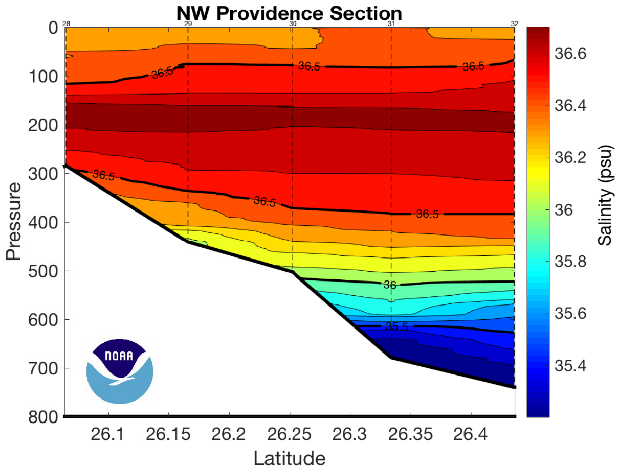
Figure 39: Salinity (PSS 78) section for the Northwest Providence Channel section. Dashed vertical lines are the CTD station locations.
