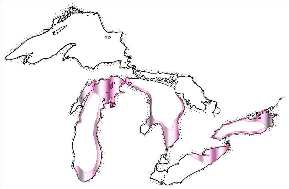
Figure 1. Area of the Great Lakes where Diporeia were once present but are now completely gone (hatched area). There is some evidence that Diporeia are now gone from portions of Georgian Bay and North Channel, Lake Huron, but the spatial extent of its disappearance is not known. Because of warm water temperatures, Diporeia are naturally not found in Green Bay, Saginaw Bay, Lake St. Clair, and in the western and central basins of Lake Erie.
