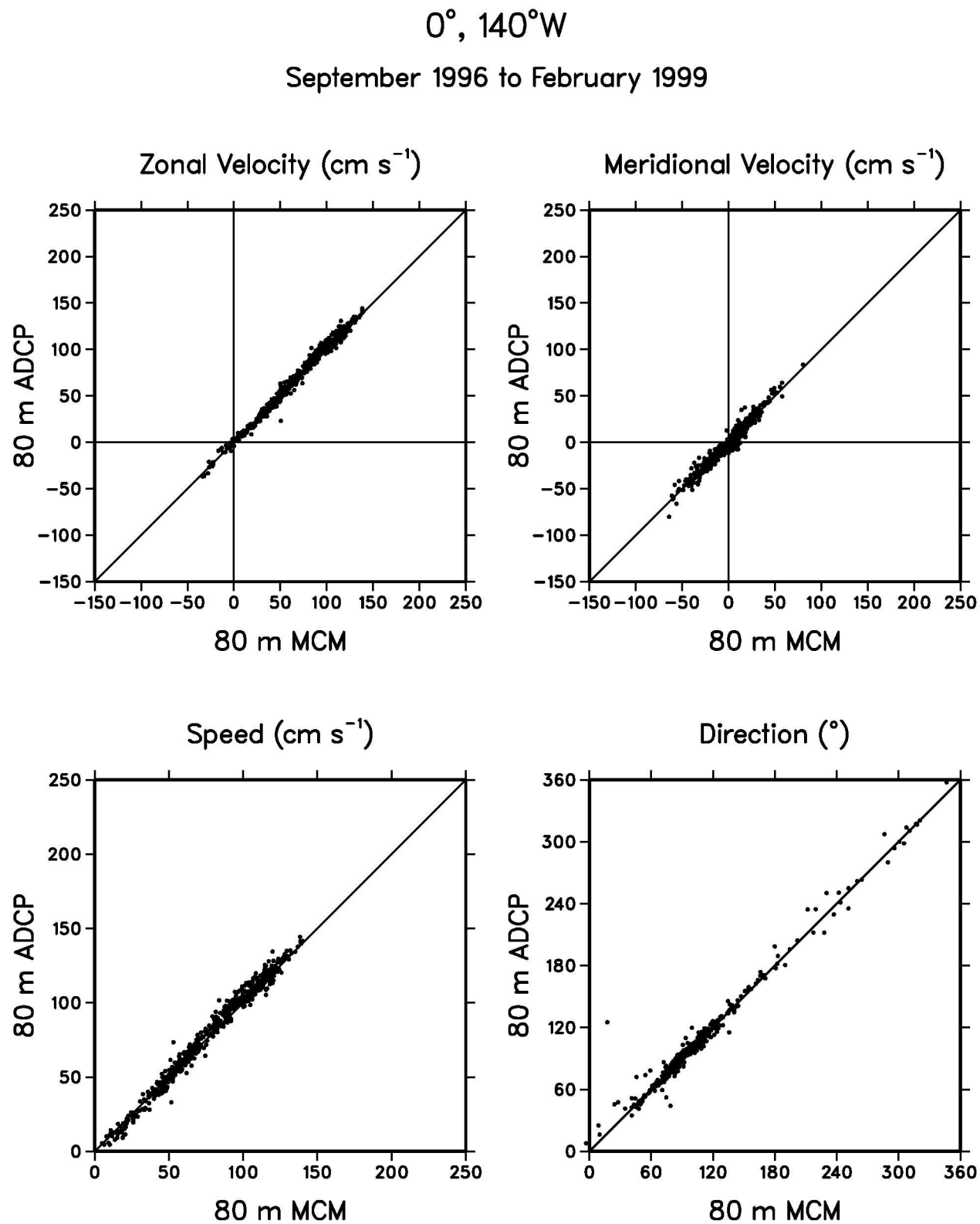
Figure 9: Scatter plot of 80 m daily averaged zonal velocity, meridional velocity, and direction from MCMs and ADCPs measured from September 1996 to February 1999 at 0^{\circ}, 140^{\circ}\text{W} .
