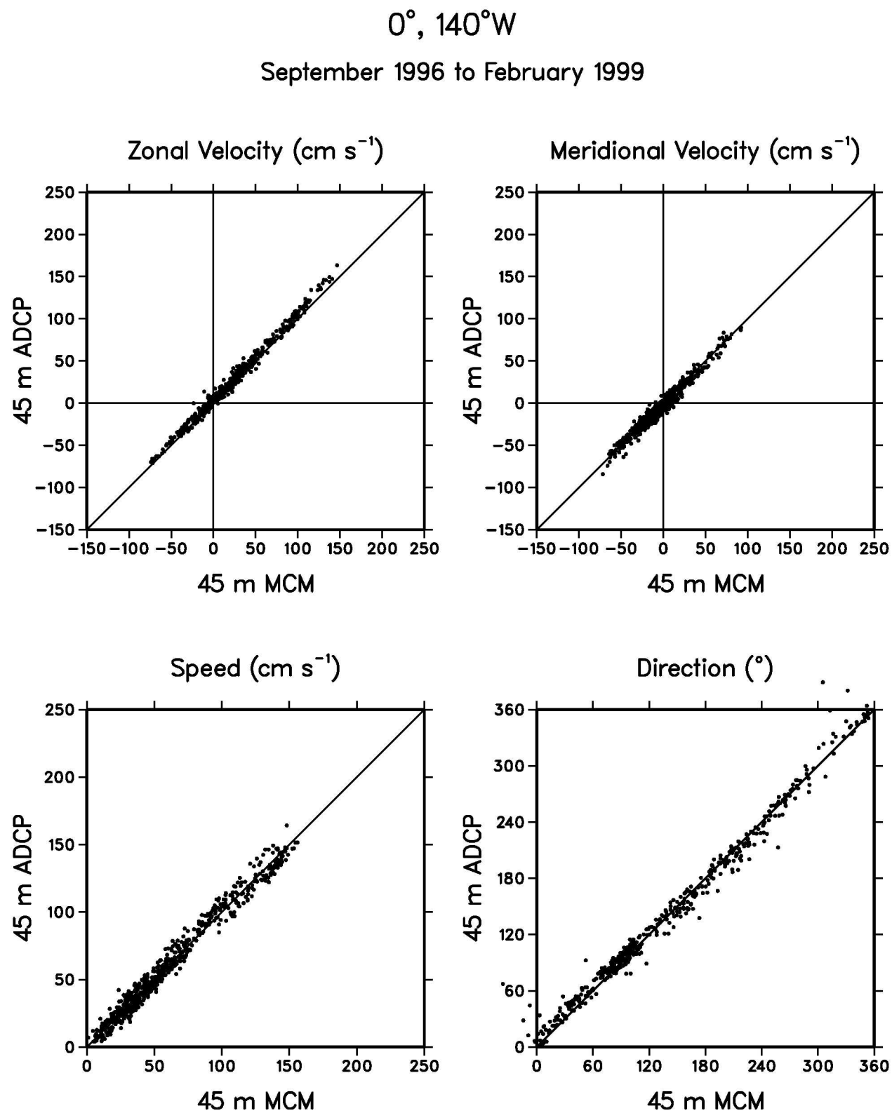
Figure 8: Scatter plot of 45 m daily averaged zonal velocity, meridional velocity, and direction from MCMs and ADCPs measured from September 1996 to February 1999 at 0^{\circ}, 140^{\circ}\text{W} .
