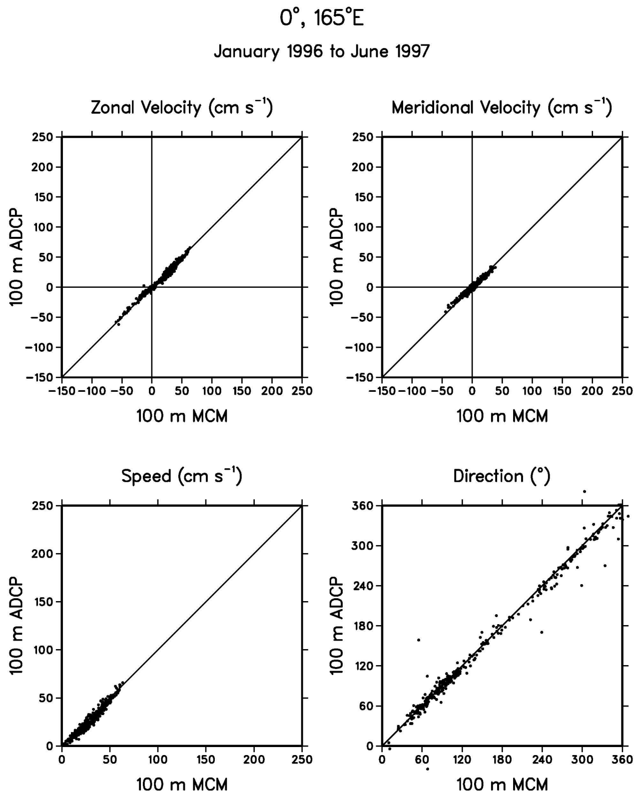
Figure 12: Scatter plot of 100 m daily averaged zonal velocity, meridional velocity, speed, and direction from MCMs and ADCPs measured from January 1996 to June 1997 at 0^{\circ}, 165^{\circ}\text{E} .
