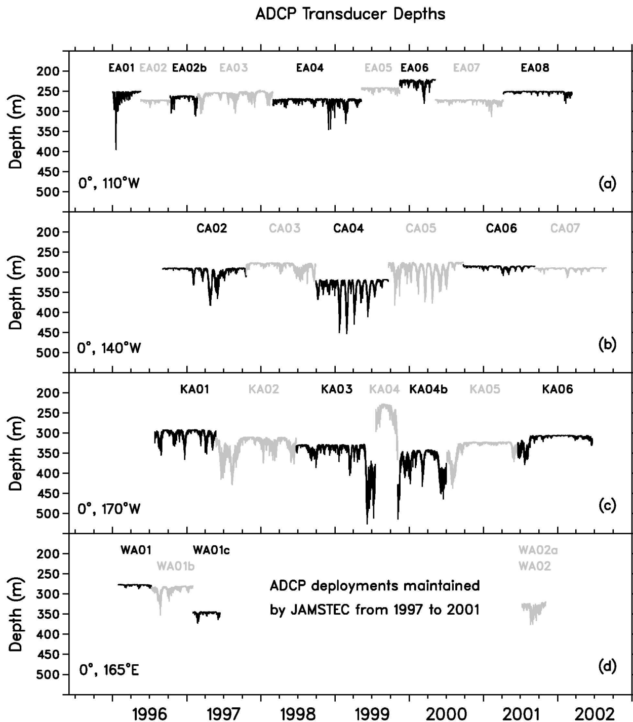
Figure 2: Hourly transducer depths for subsurface ADCP deployments at 0^\circ, 110^\circ\text{W} (a), at 0^\circ, 140^\circ\text{W} (b), at 0^\circ, 170^\circ\text{W} (c), and at 0^\circ, 165^\circ\text{E} (d).
