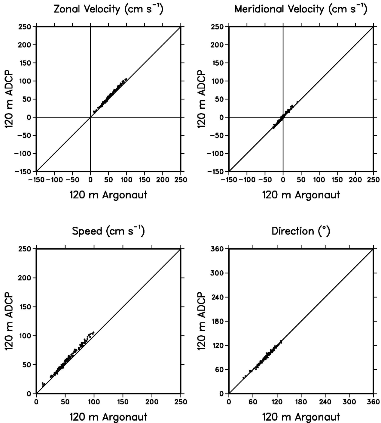
Figure 15: Scatter plot of 120 m daily averaged zonal velocity, meridional velocity, speed, and direction from Sontek Argonaut-MD current meters and ADCPs measured from April to September 2001 at 0°, 110°W.
