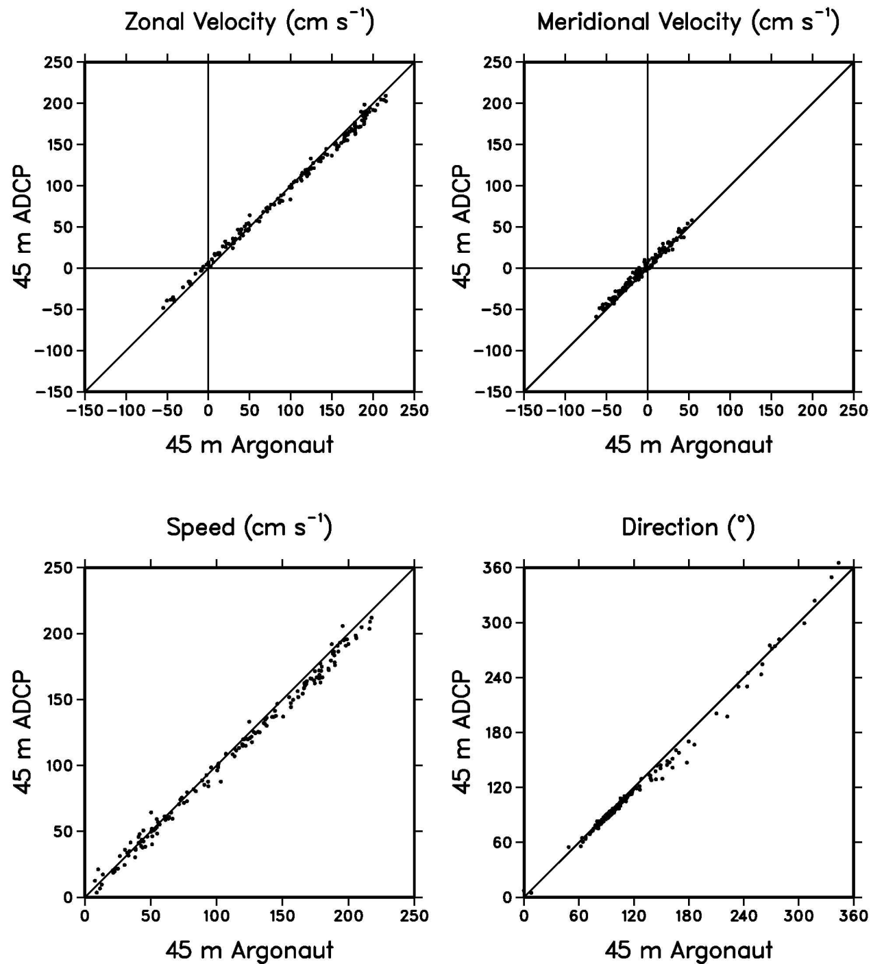
Figure 14: Scatter plot of 45 m daily averaged zonal velocity, meridional velocity, speed, and direction from Sontek Argonaut-MD current meters and ADCPs measured from April to September 2001 at 0°, 110°W.
