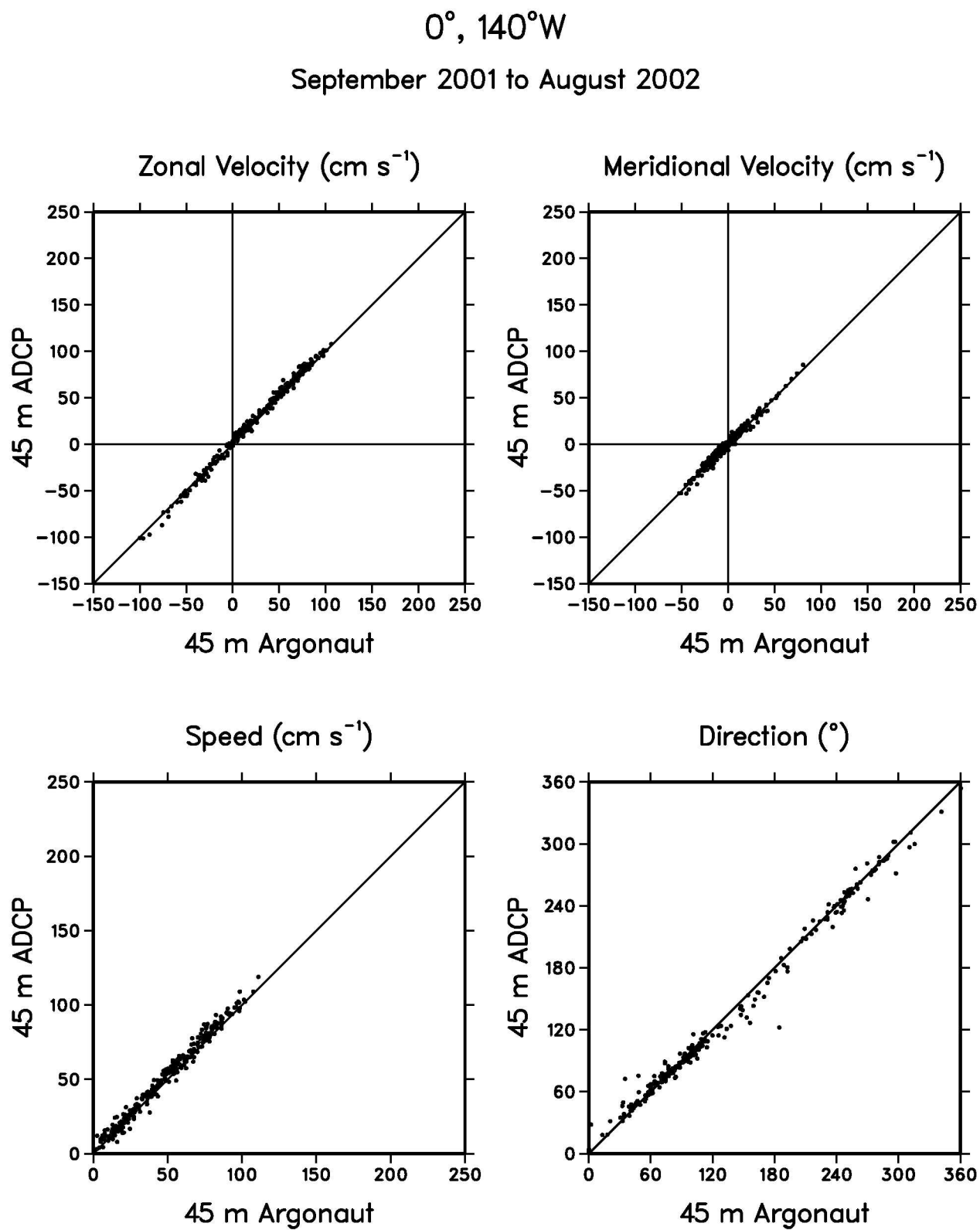
Figure 17: Scatter plot of 45 m daily averaged zonal velocity, meridional velocity, speed and direction from Sontek Argonaut-MD current meters and ADCPs measured from September 2001 to August 2002 at 0^{\circ}, 140^{\circ}\text{W} .
