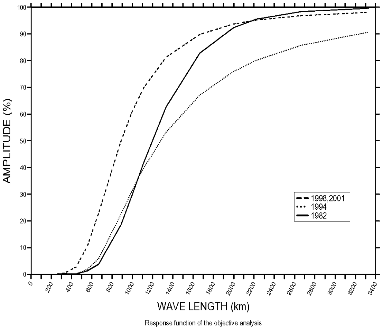
Figure 2. Response function of the WOA01, WOA98, WOA94, and Levitus (1982) objective analysis schemes.
