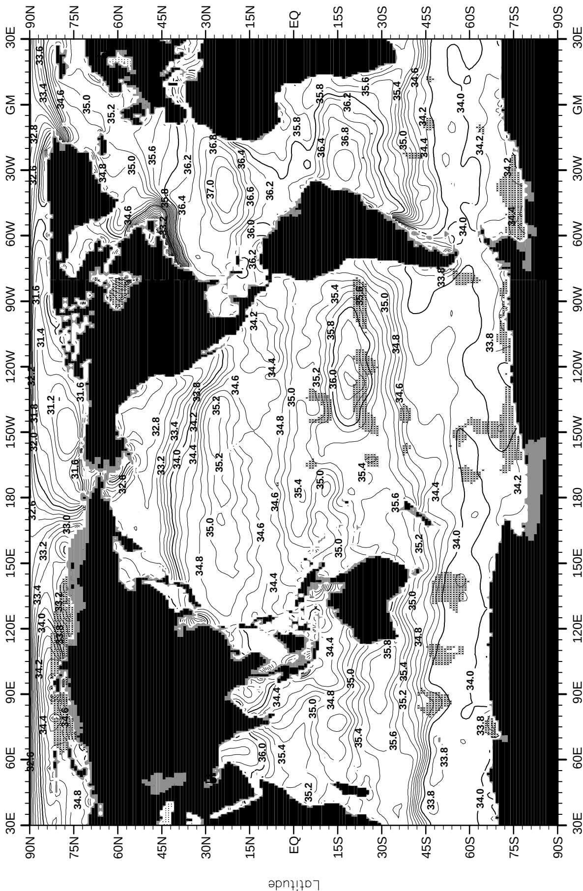
Fig. B39. Spring (Apr.-Jun.) mean salinity (PSS) at 50 m. depth.
