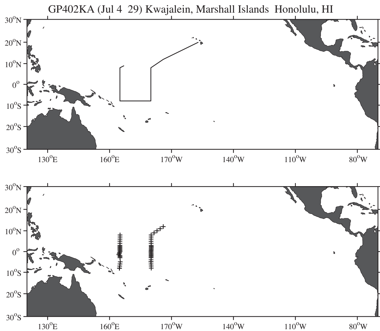
Figure 2l: GP4-02-KA cruise track and station locations.
