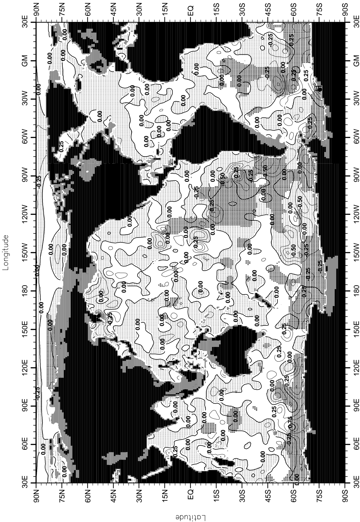
Fig. B40. Summer (Jul.-Sep.) minus annual oxygen (ml/l) at 250 m. depth.
