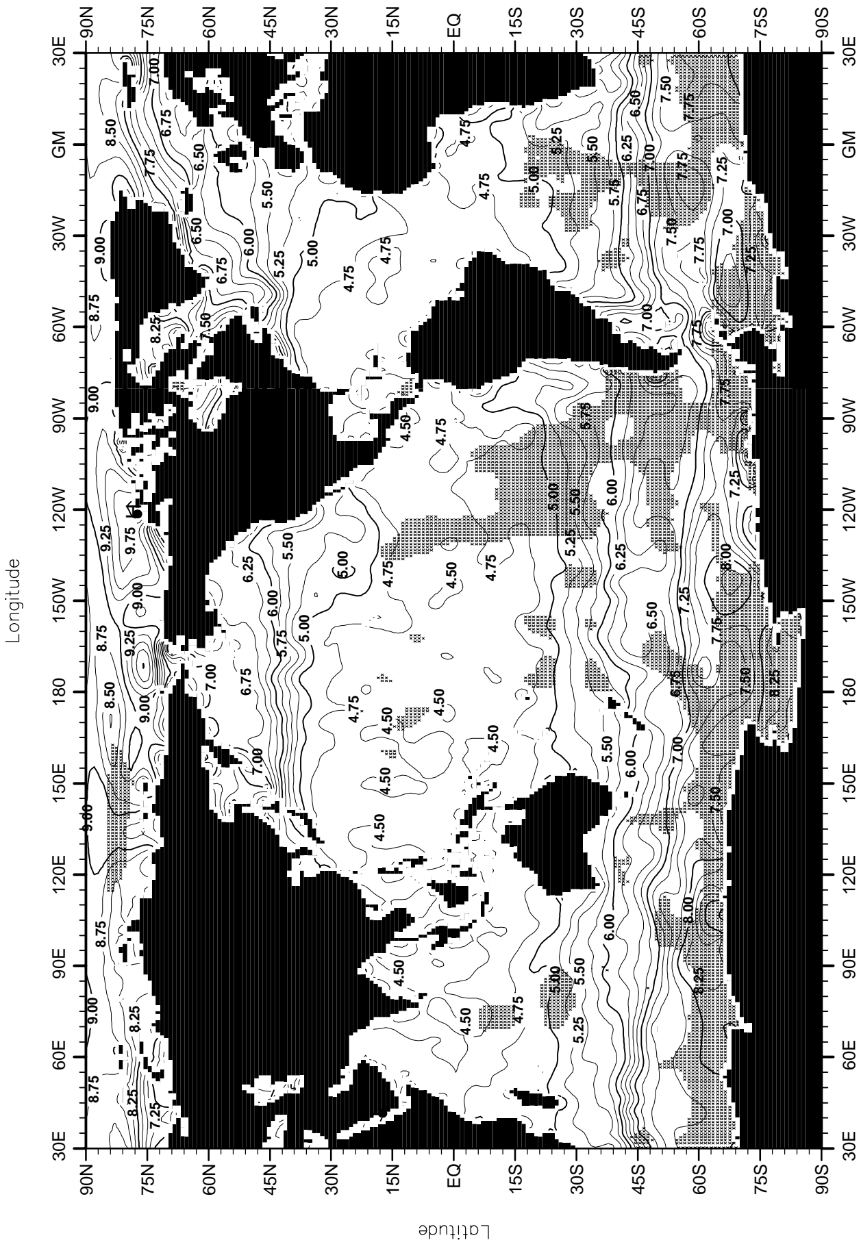
Fig. B33. Summer (Jul.-Sep.) mean oxygen (m/l) at the surface.
