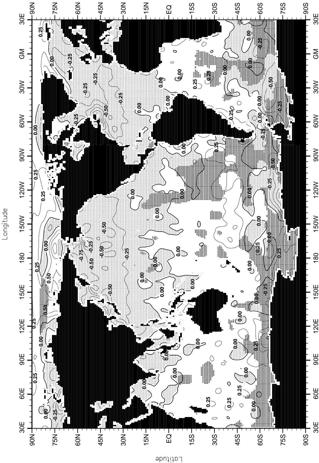
Fig. B34. Summer (Jul.-Sep.) minus annual oxygen (mM/l) at the surface.
