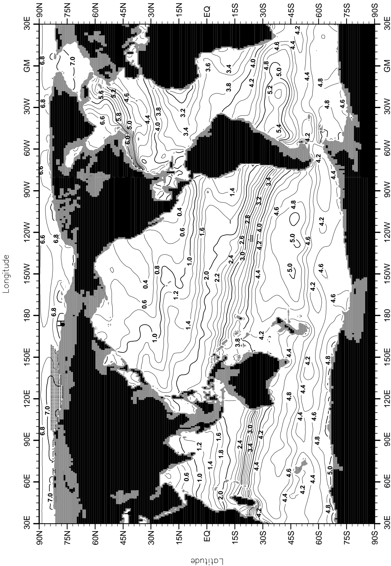
Fig. A27. Annual mean oxygen (ml/l) at 1000 m. depth.
