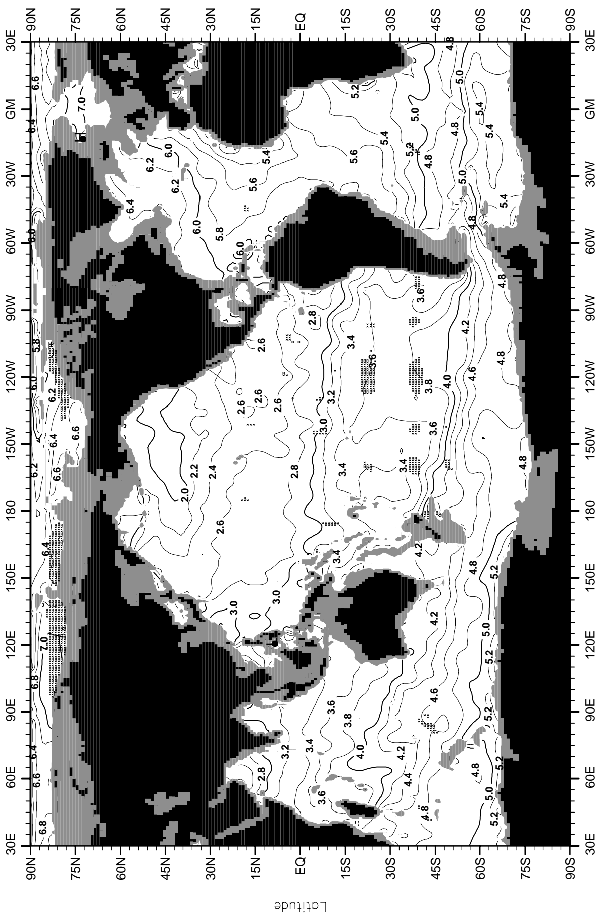
Fig. A30. Annual mean oxygen (ml/l) at 2500 m. depth.
