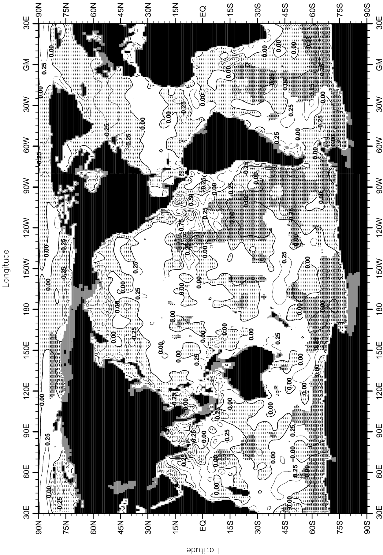
Fig. B36. Summer (Jul.-Sep.) minus annual oxygen (ml/l) at 75 m. depth.
