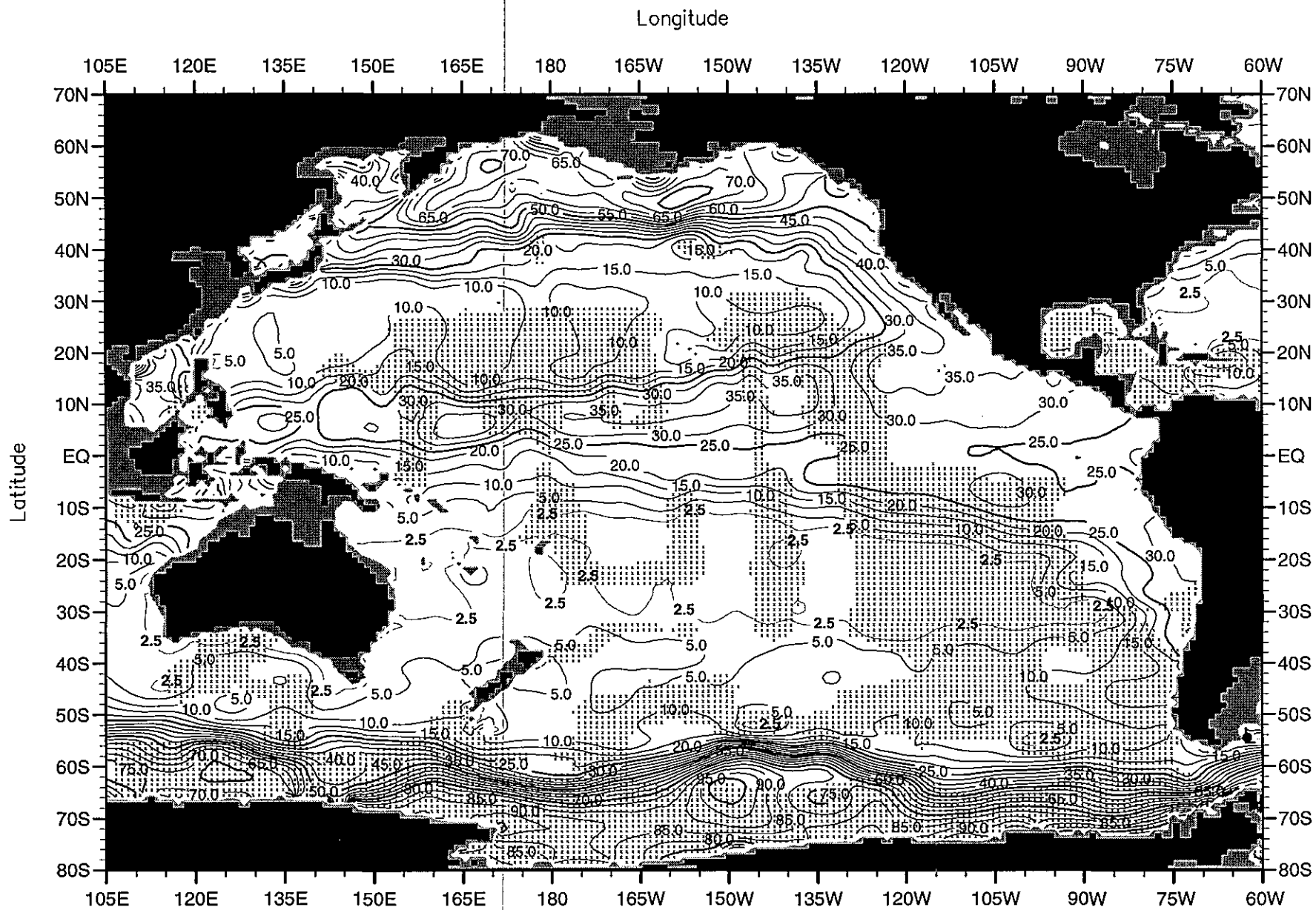
Fig. F42. Summer (Jul.-Sep.) mean silicate ( \mu\text{M} ) at 250 m. depth .
