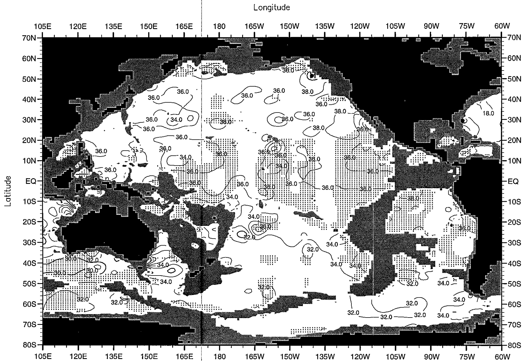
Fig. C32. Annual mean nitrate ( \mu\text{M} ) at 4000 m. depth.
