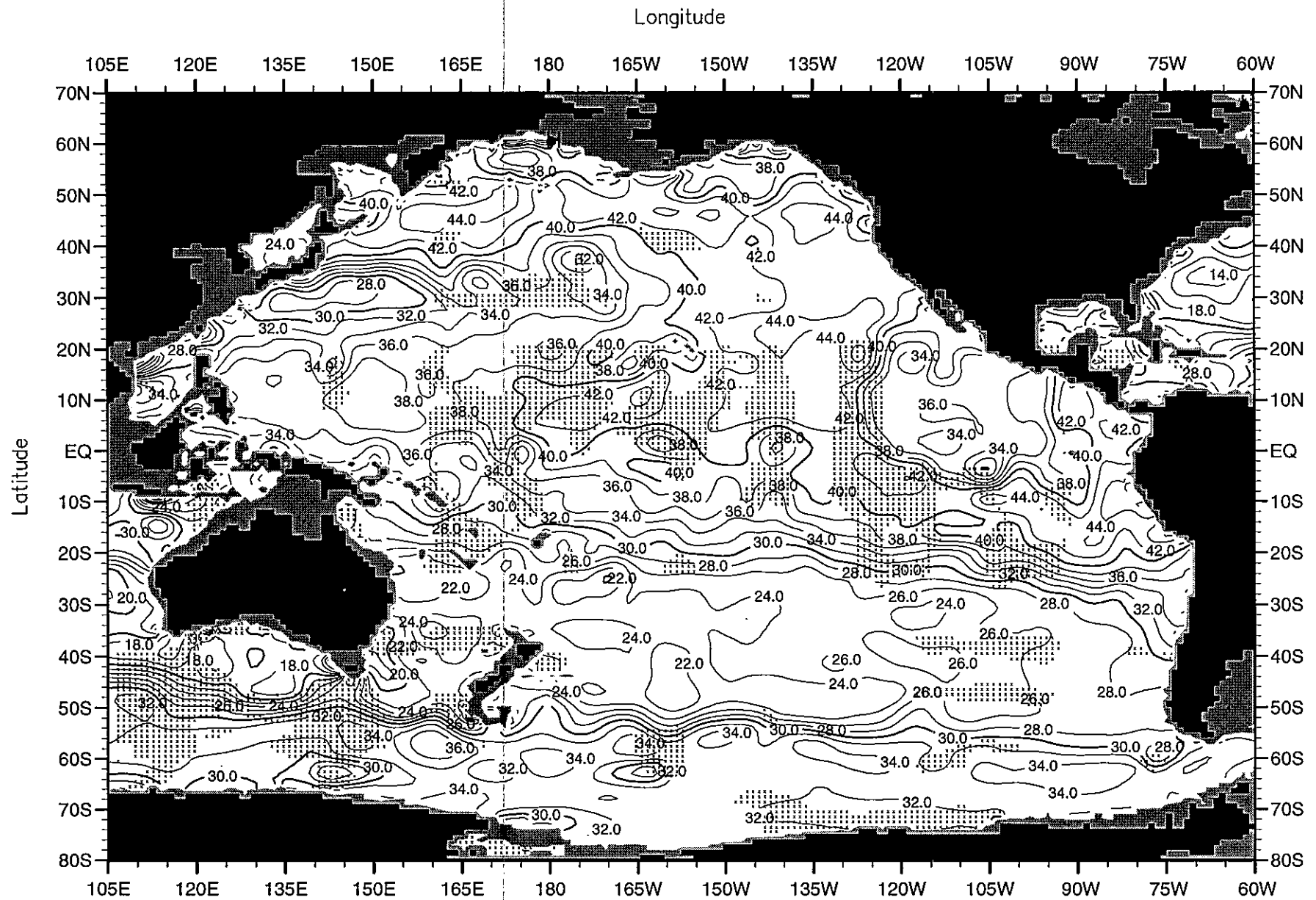
Fig. C26. Annual mean nitrate ( \mu\text{M} ) at 700 m. depth .
