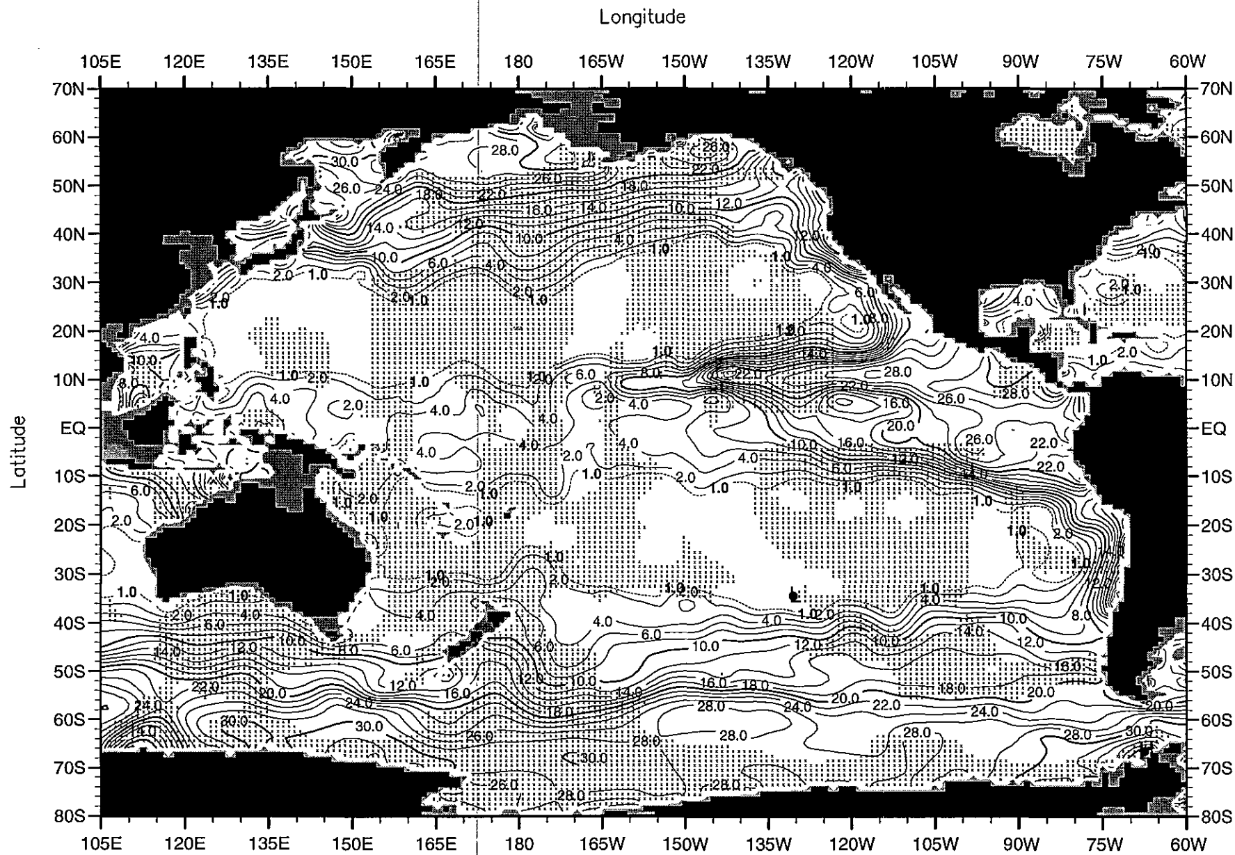
Fig. D46. Fall (Oct.-Dec.) mean nitrate ( \mu\text{M} ) at 100 m. depth .
