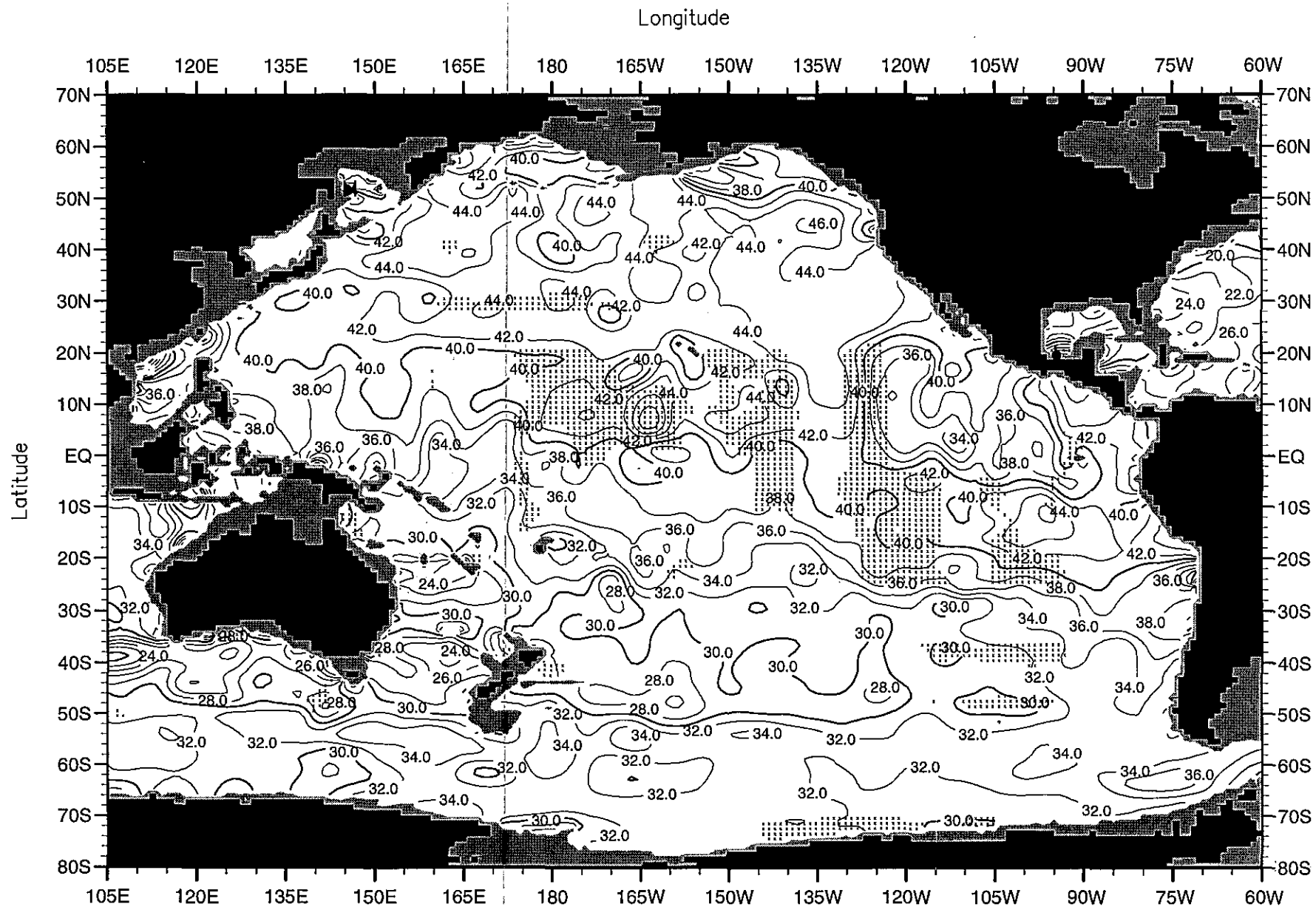
Fig. C27. Annual mean nitrate ( \mu\text{M} ) at 1000 m. depth.
