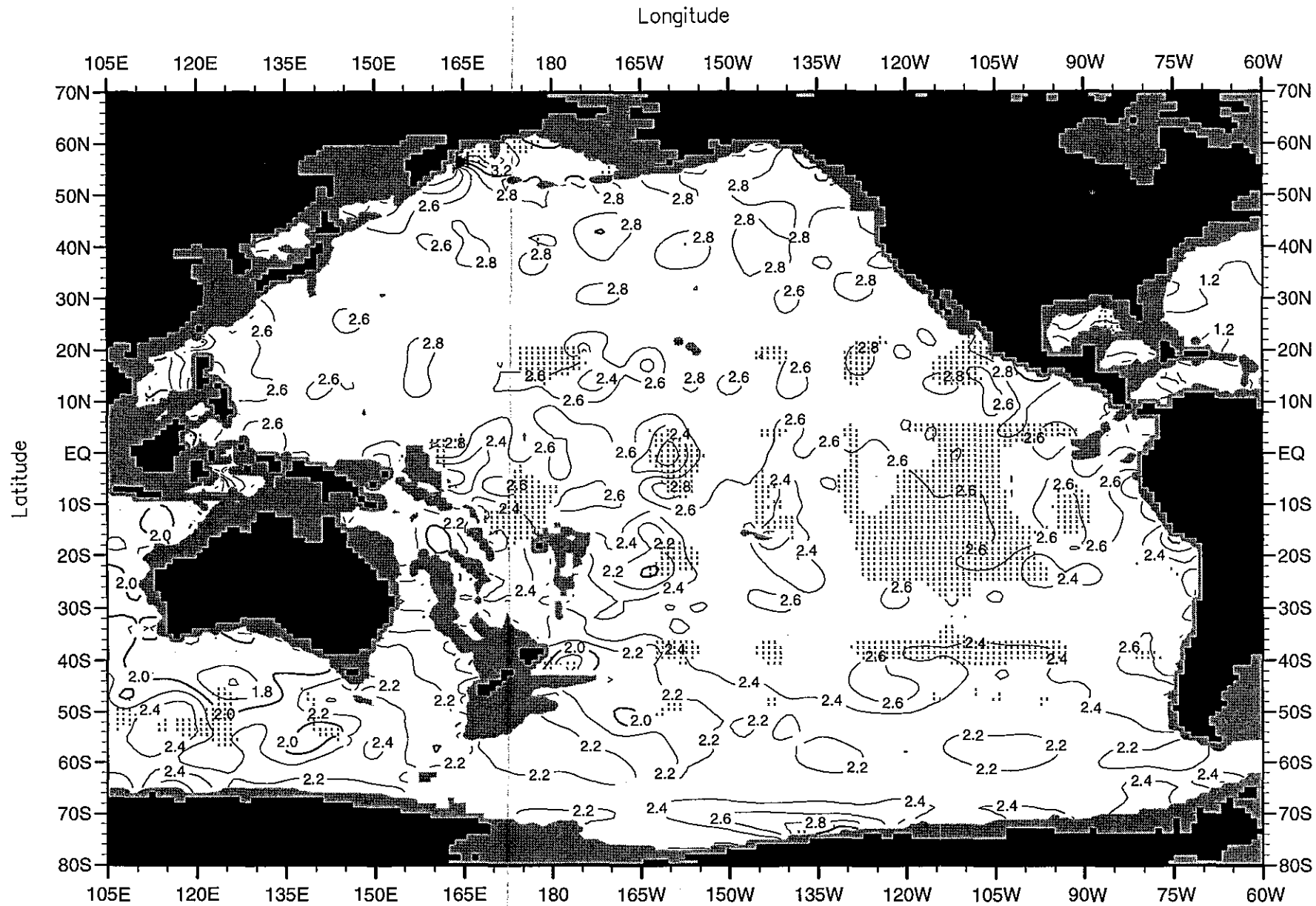
Fig. A31. Annual mean phosphate ( \mu\text{M} ) at 3000 m. depth.
