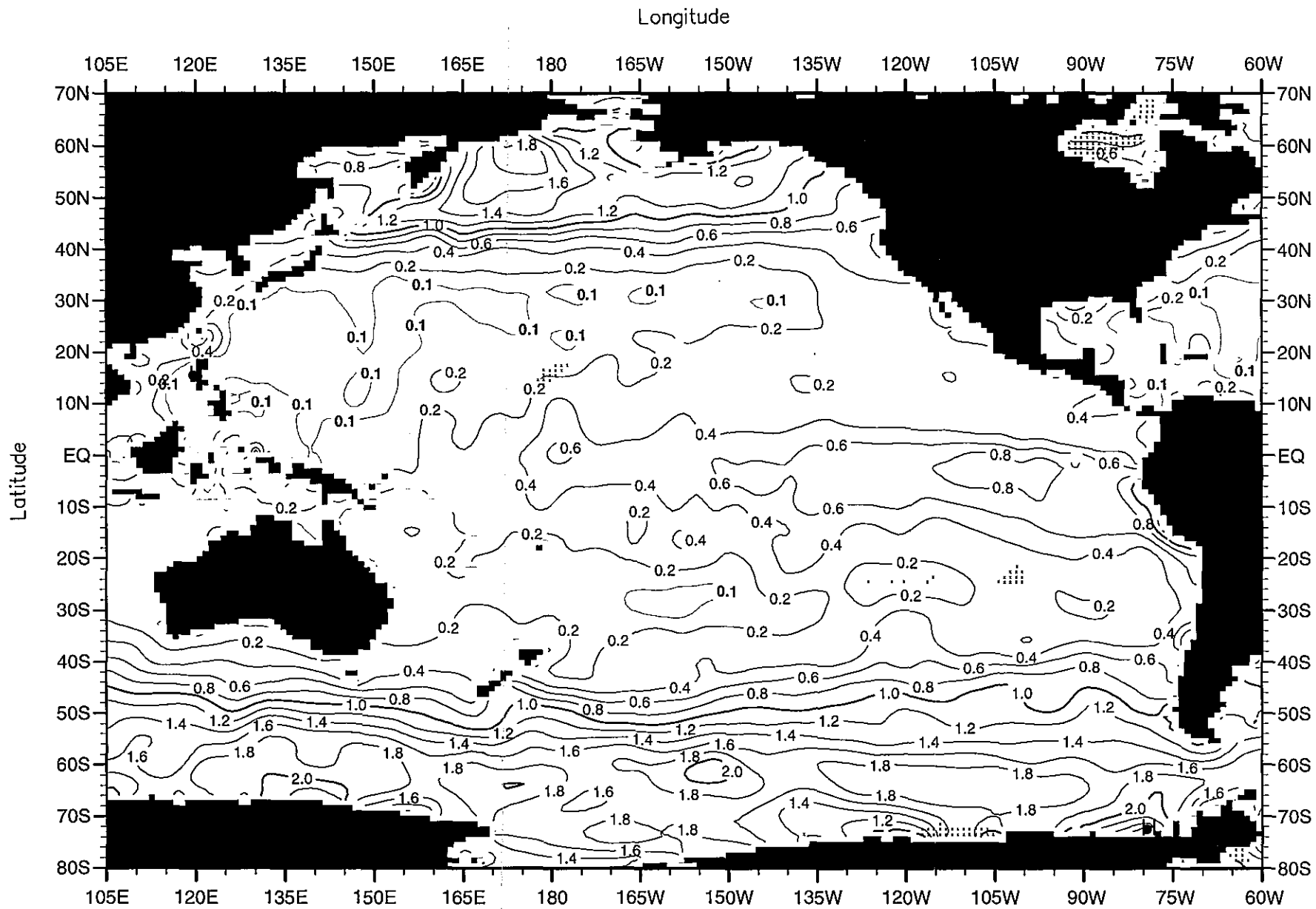
Fig. A17. Annual mean phosphate ( \mu\text{M} ) at the surface.
