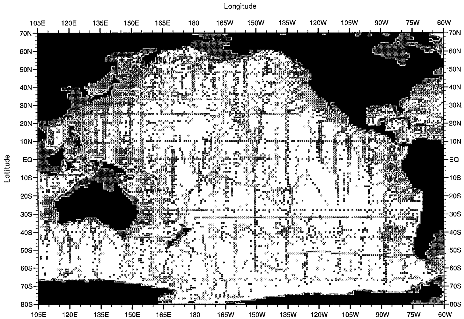
Fig. 1b. Annual phosphate standard error of the mean ( \mu\text{M} ) at 500 meters depth by one-degree squares
