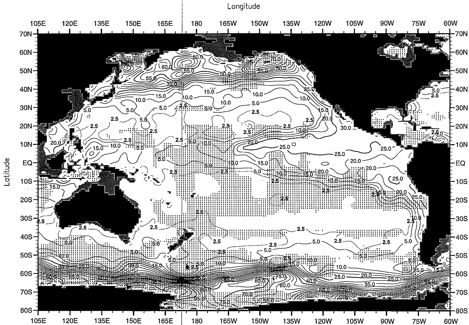
Fig. F35. Spring (Apr.-Jun.) mean silicate ( \mu\text{M} ) at 150 m. depth .
