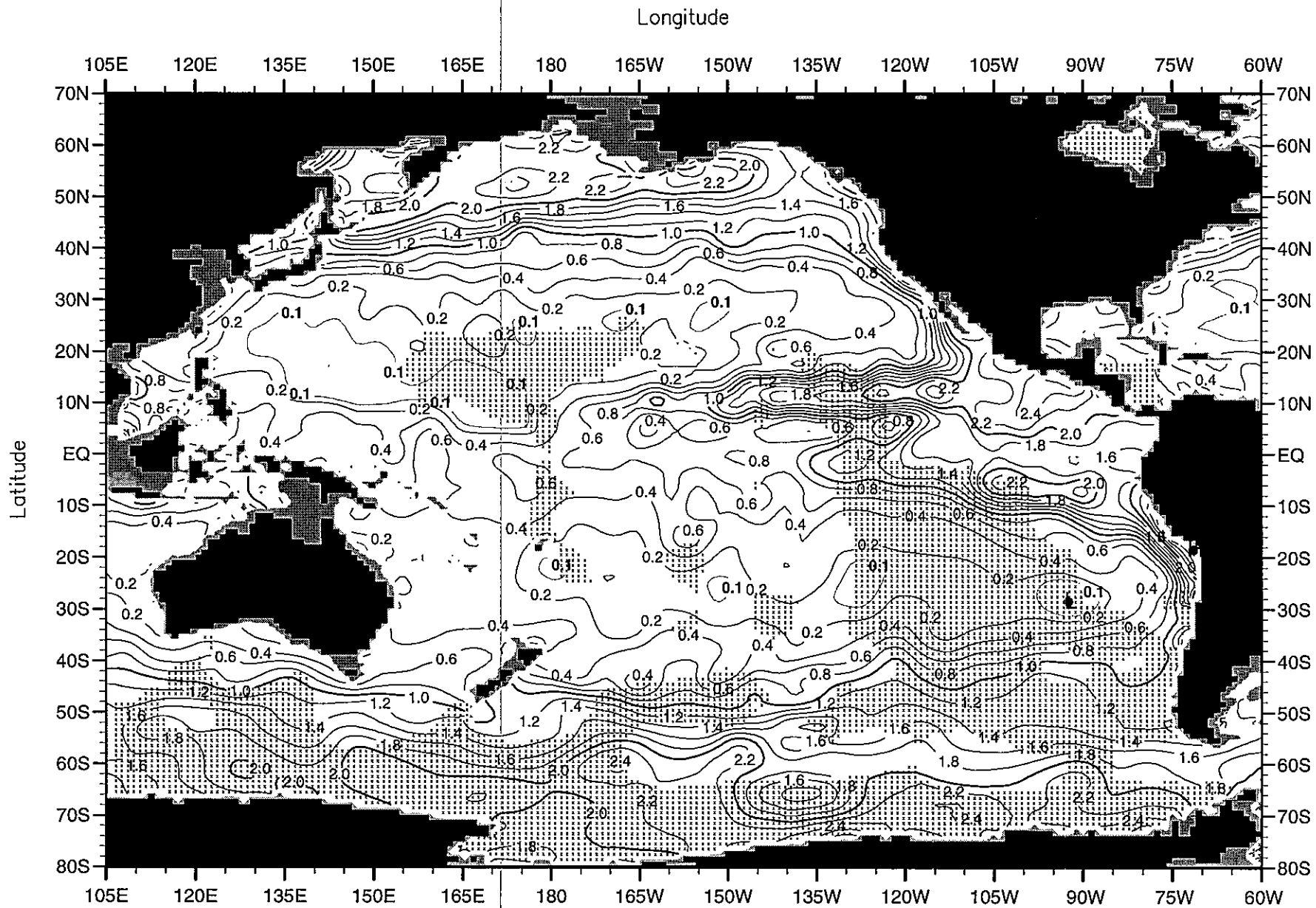
Fig. B40. Summer (Jul.-Sep.) mean phosphate ( \mu\text{M} ) at 100 m. depth .
