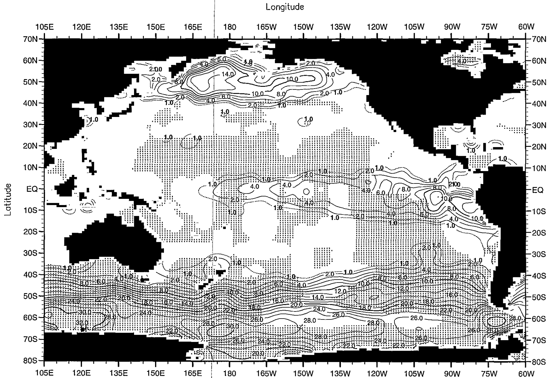
Fig. D37. Summer (Jul.-Sep.) mean nitrate ( \mu\text{M} ) at the surface .
