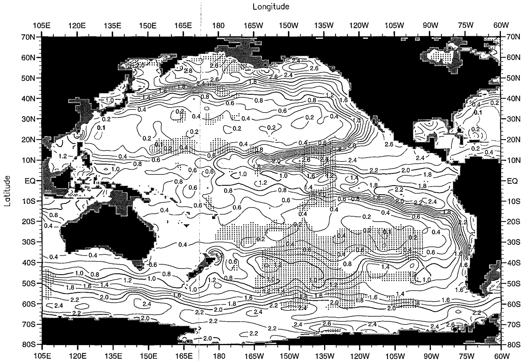
Fig. B29. Winter (Jan.-Mar.) mean phosphate ( \mu\text{M} ) at 150 m. depth .
