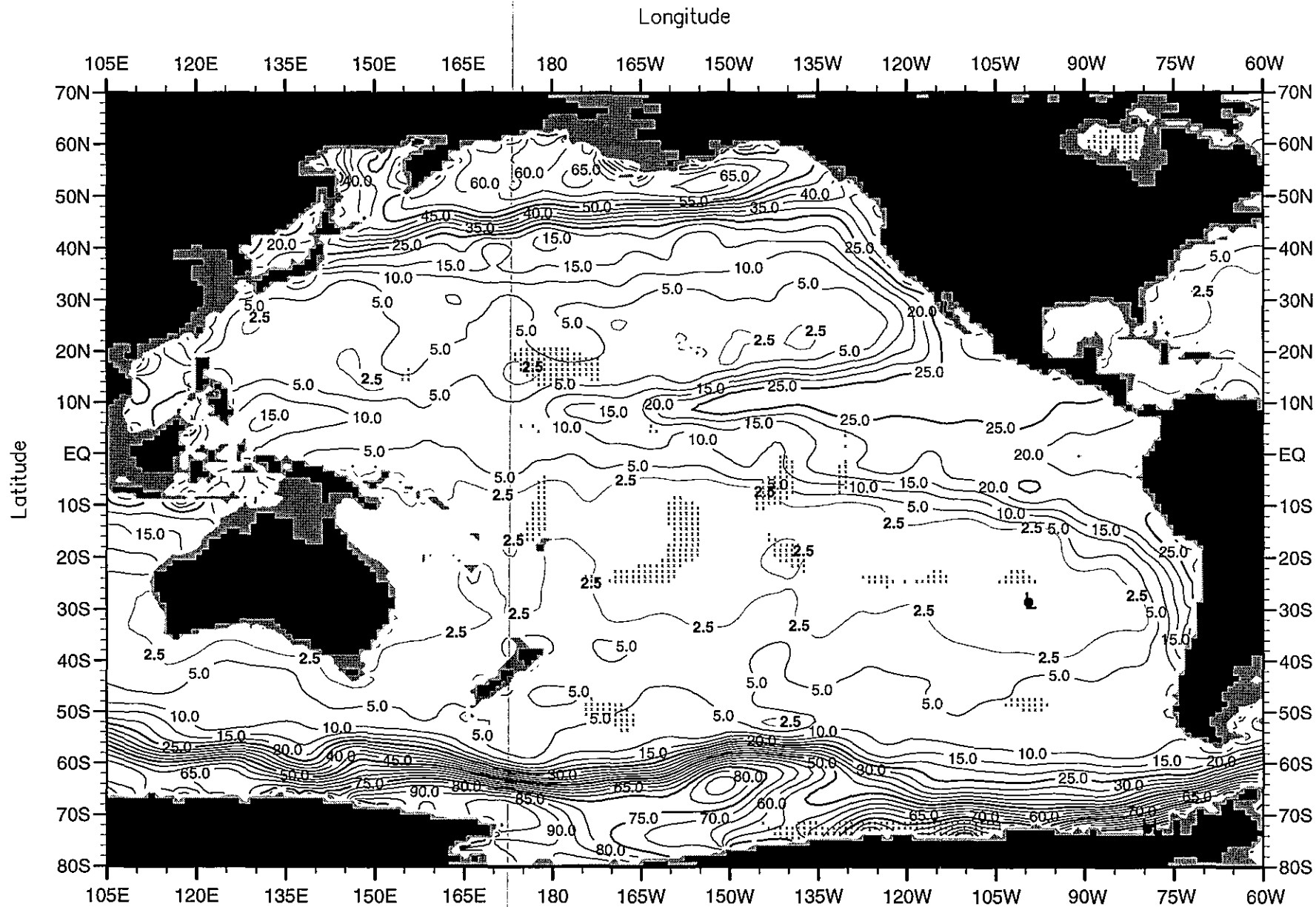
Fig. E21. Annual mean silicate ( \mu\text{M} ) at 150 m. depth .
