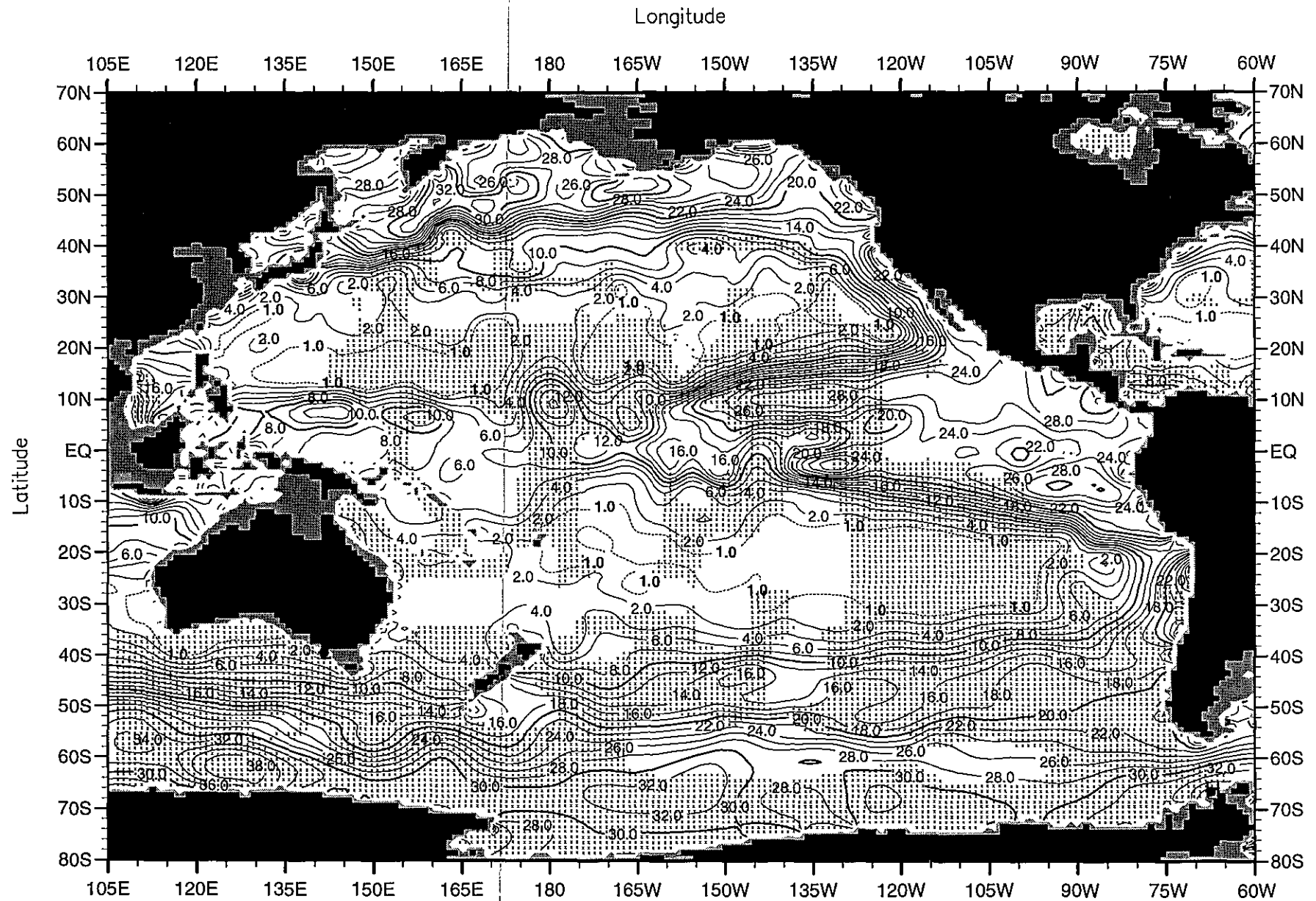
Fig. D41. Summer (Jul.-Sep.) mean nitrate ( \mu\text{M} ) at 150 m. depth.
