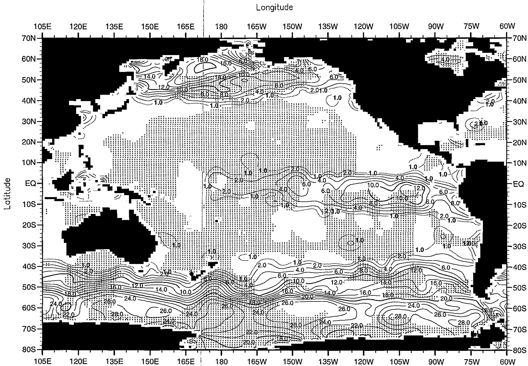
Fig. D43. Fall (Oct.-Dec.) mean nitrate ( \mu\text{M} ) at the surface .
