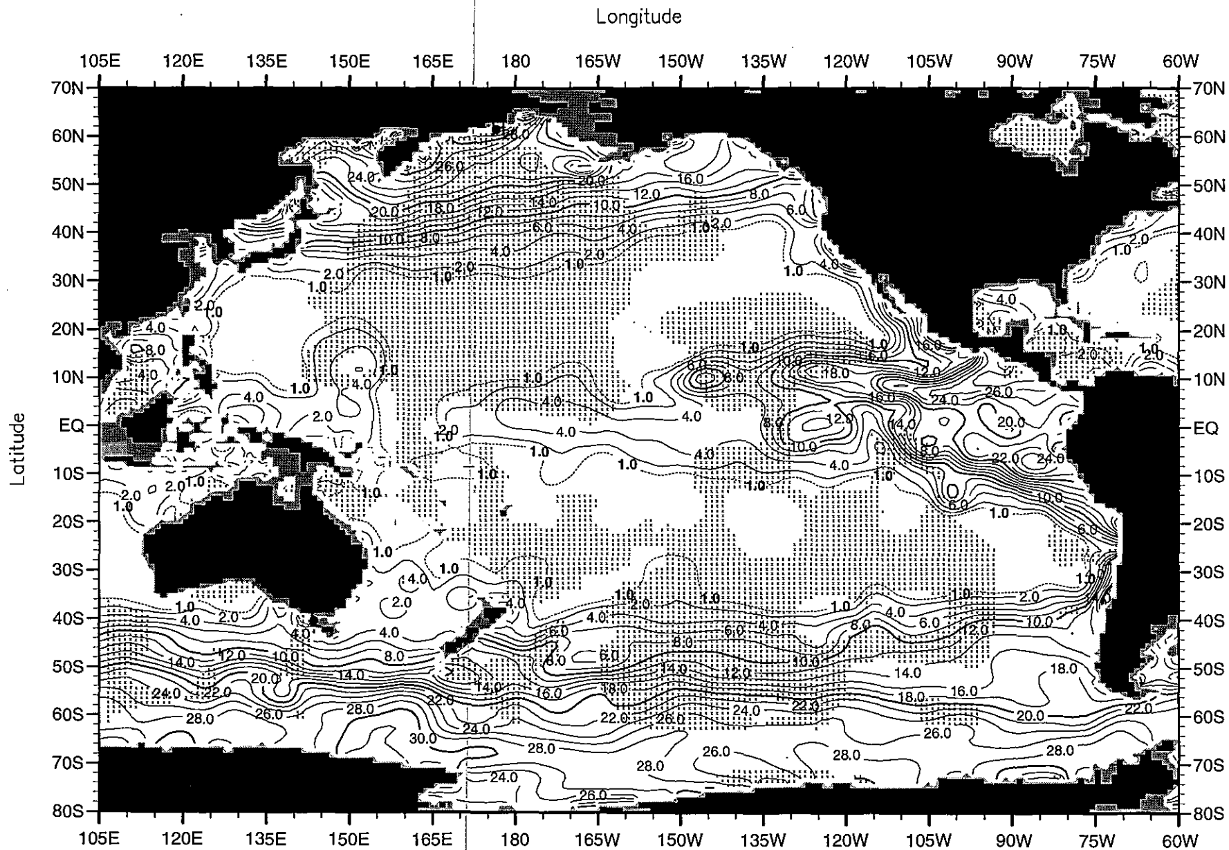
Fig. D27. Winter (Jan.-Mar.) mean nitrate ( \mu\text{M} ) at 75 m. depth.
