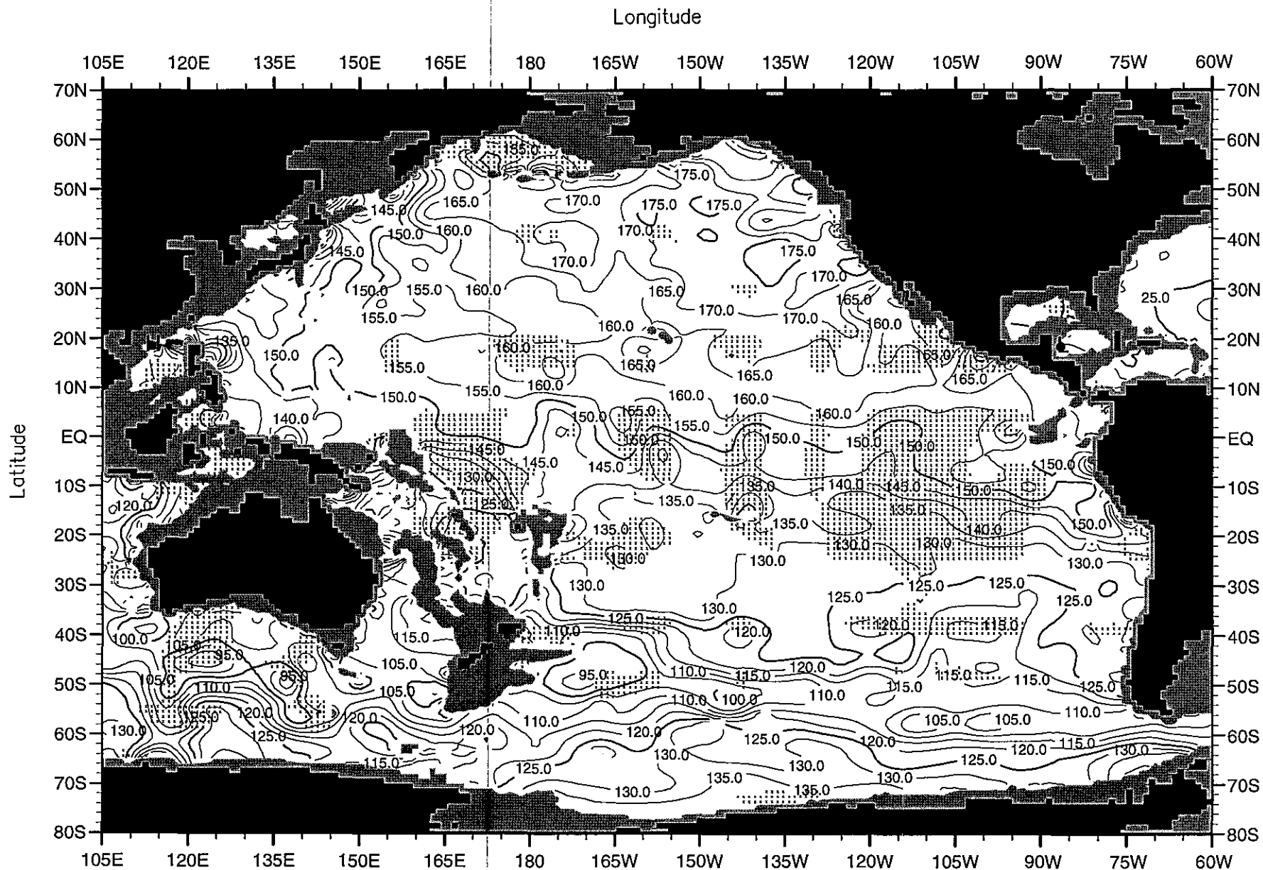
Fig. E31. Annual mean silicate ( \mu\text{M} ) at 3000 m. depth. Minimum Value= 14.68 Maximum Value= 191.02 Contour Interval: 5.00
