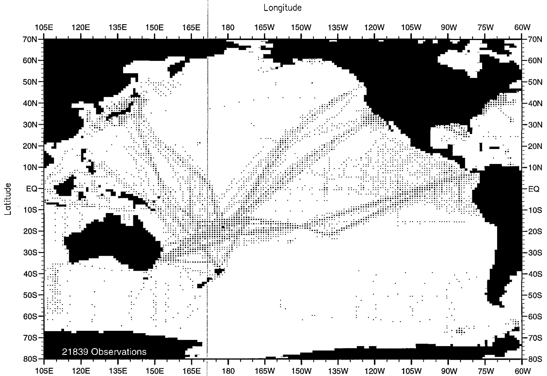
Fig. H4. Fall (Oct.-Dec.) chlorophyll observations at the surface .
