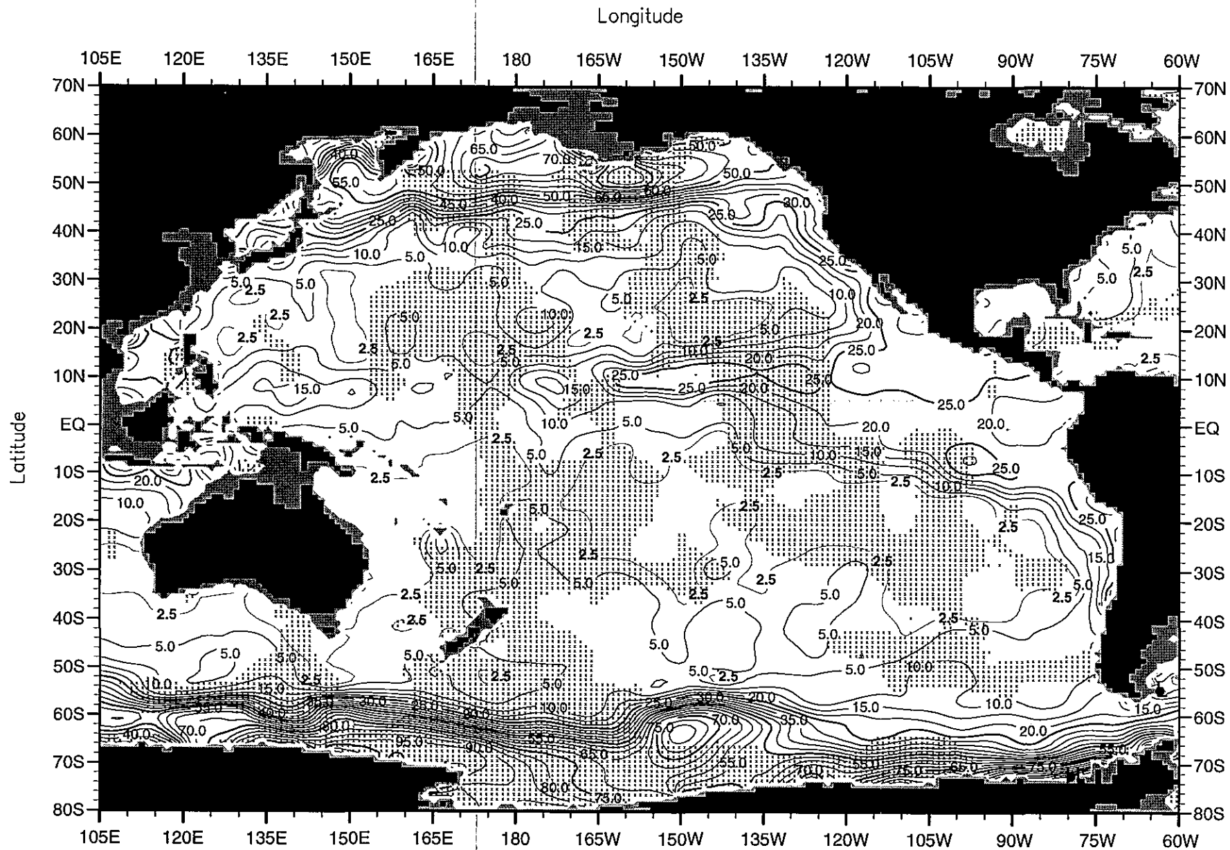
Fig. F47. Fall (Oct.-Dec.) mean silicate ( \mu\text{M} ) at 150 m. depth .
