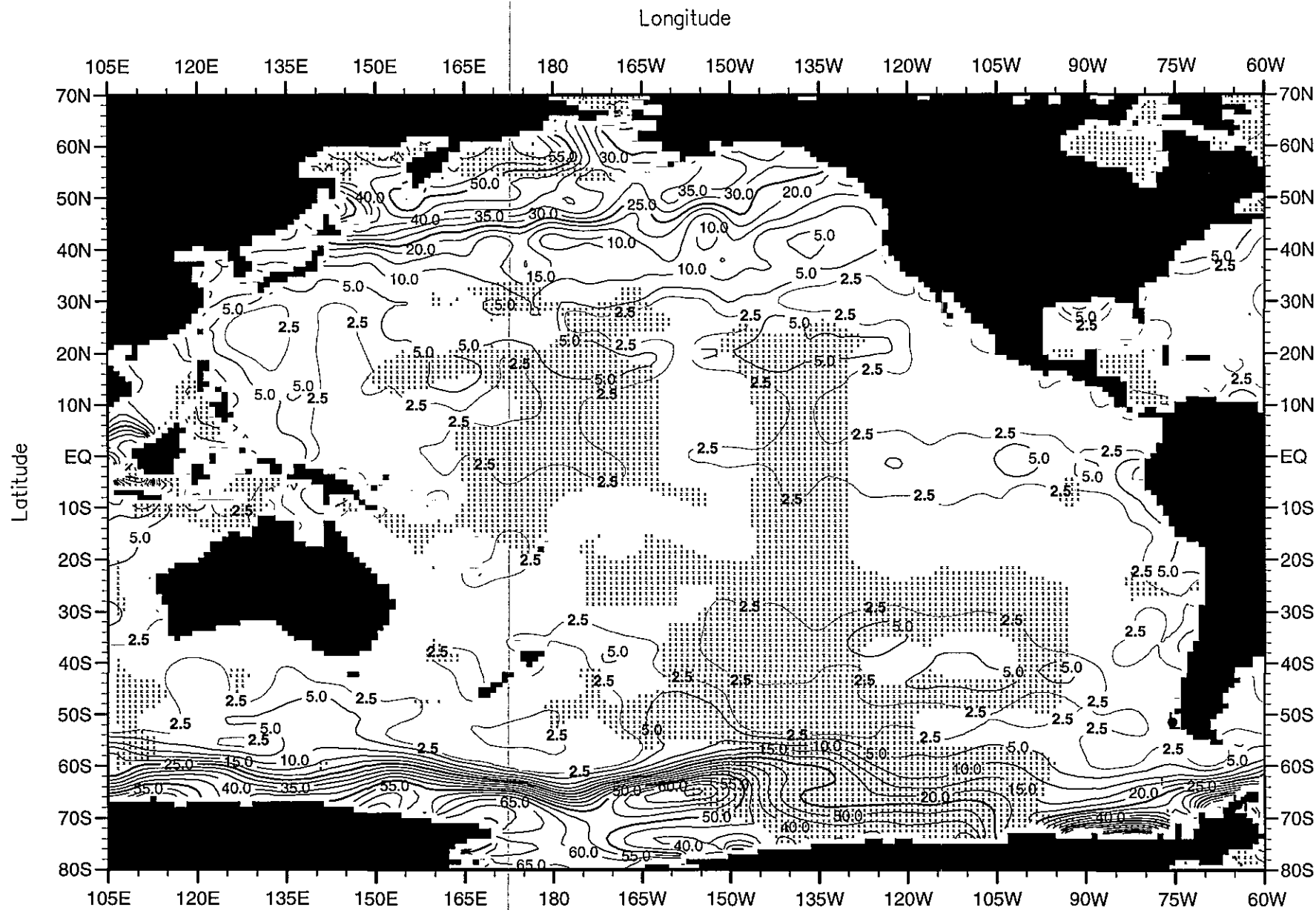
Fig. F25. Winter (Jan.-Mar.) mean silicate ( \mu\text{M} ) at the surface . Minimum Value= 0.00 Maximum Value= 93.19 Contour Interval: 5.00
