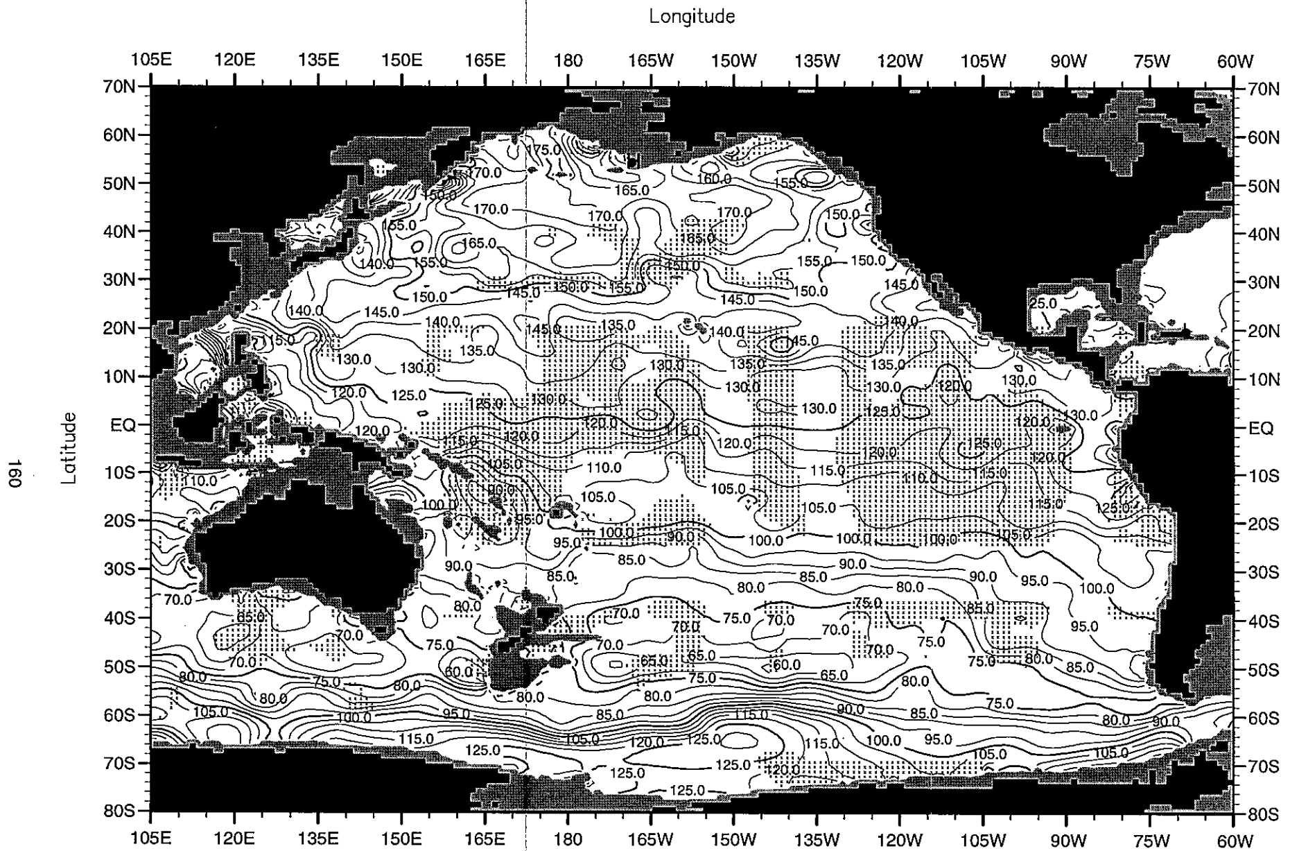
Fig. E28. Annual mean silicate ( \mu\text{M} ) at 1500 m. depth .
