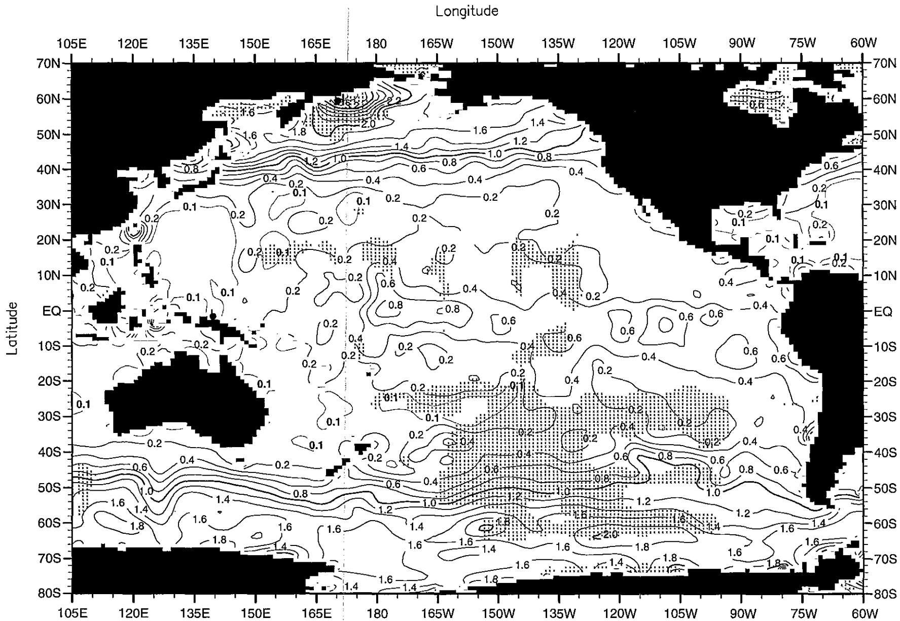
Fig. B25. Winter (Jan.-Mar.) mean phosphate ( \mu\text{M} ) at the surface .
