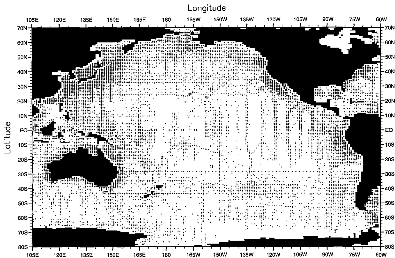
Fig. E1. Annual silicate observations at the surface .
