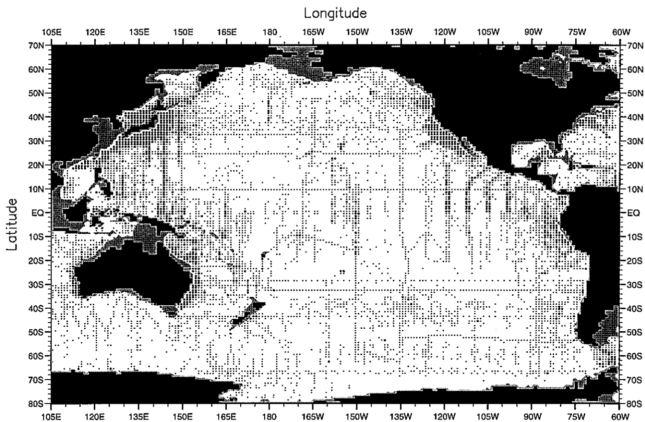
Fig. E7. Annual silicate observations at 250 m. depth .
