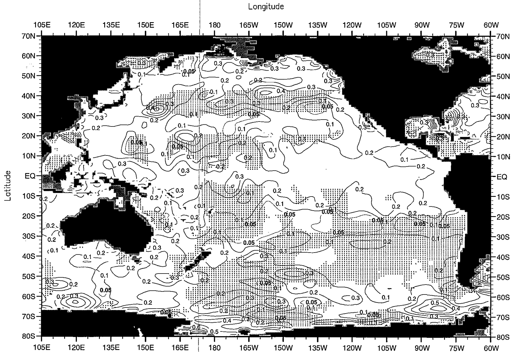
Fig. G11. Annual mean chlorophyll ( \mu\text{g/l} ) at 75 m. depth .
