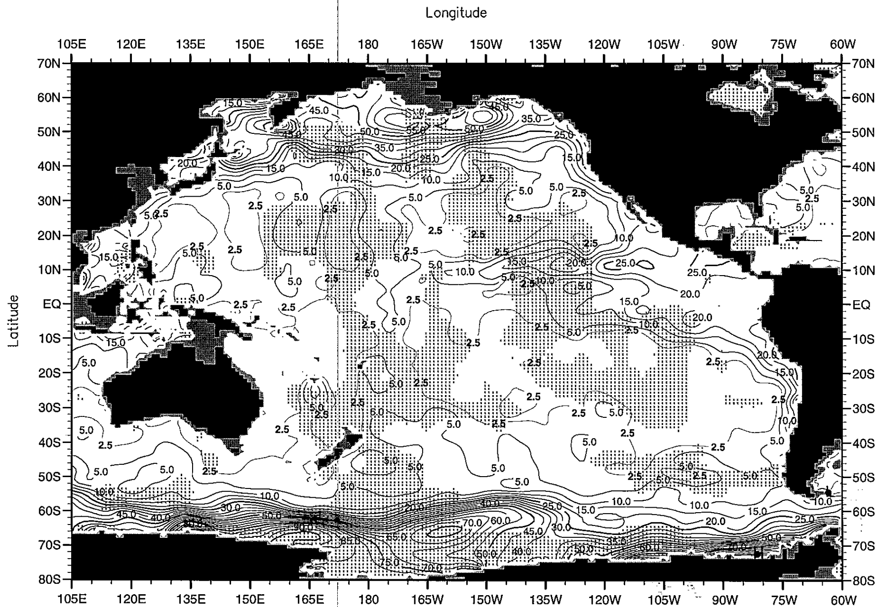
Fig. F46. Fall (Oct.-Dec.) mean silicate ( \mu\text{M} ) at 100 m. depth .
