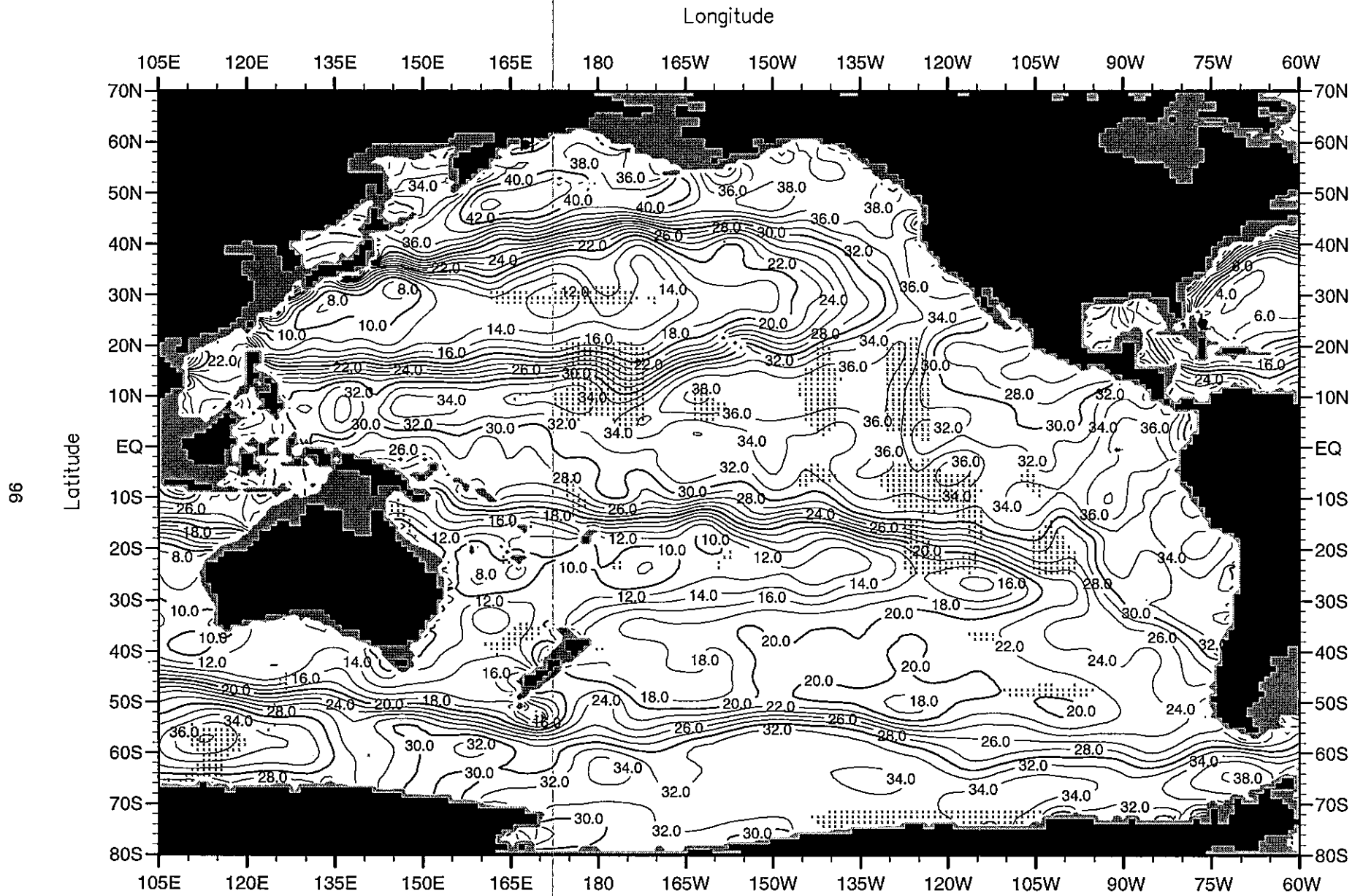
Fig. C24. Annual mean nitrate ( \mu\text{M} ) at 400 m. depth .
