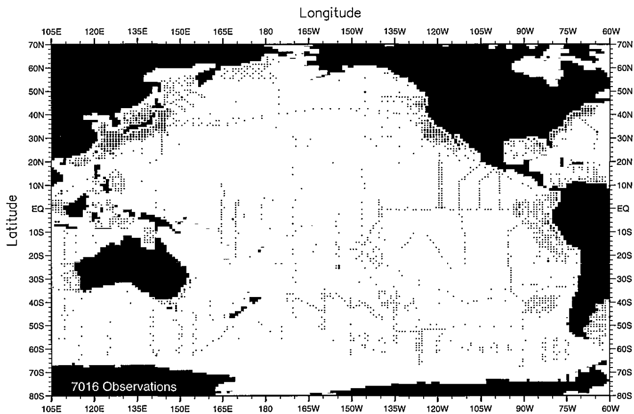
Fig. D19. Fall (Oct.-Dec.) nitrate observations at the surface .
