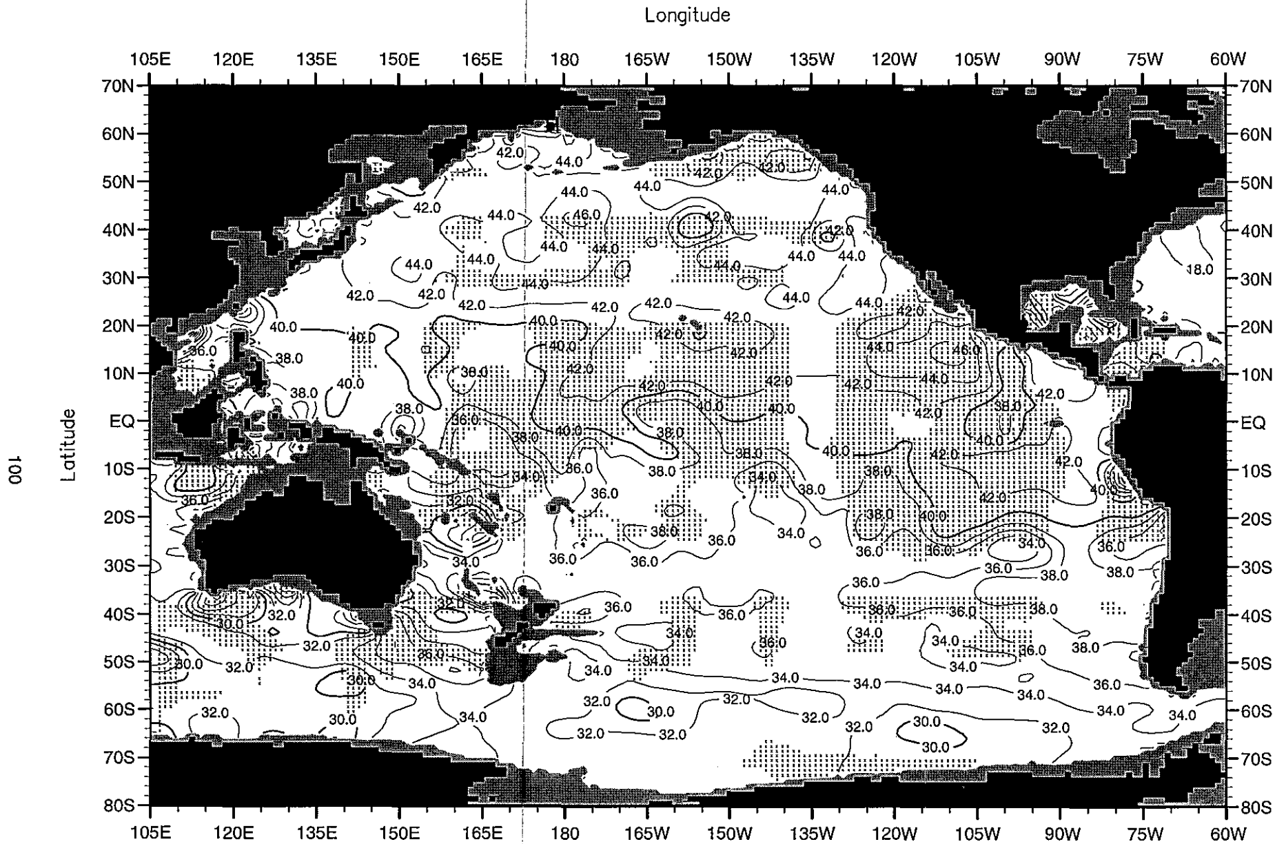
Fig. C28. Annual mean nitrate ( \mu\text{M} ) at 1500 m. depth .
