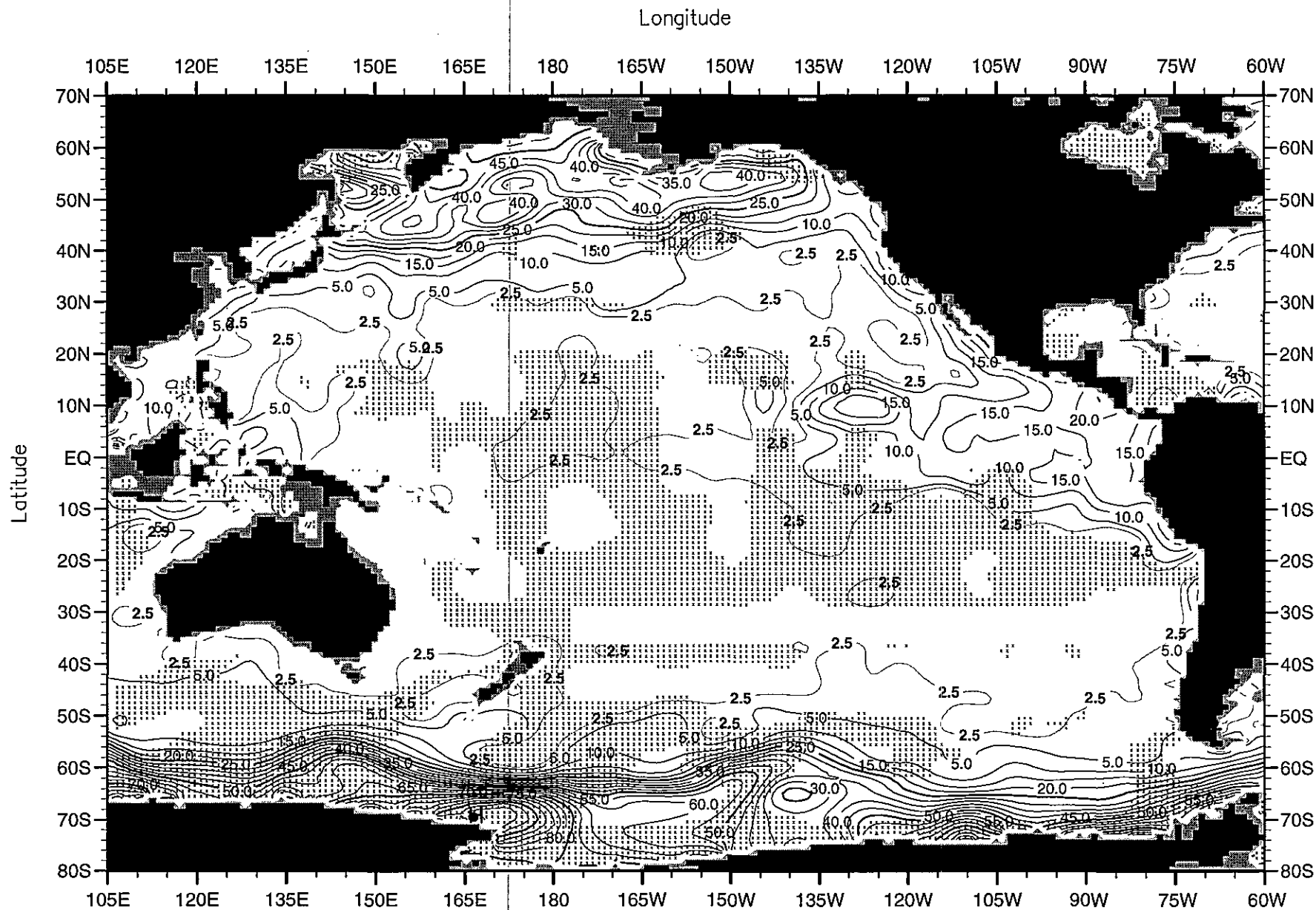
Fig. F33. Spring (Apr.-Jun.) mean silicate ( \mu\text{M} ) at 75 m. depth.
