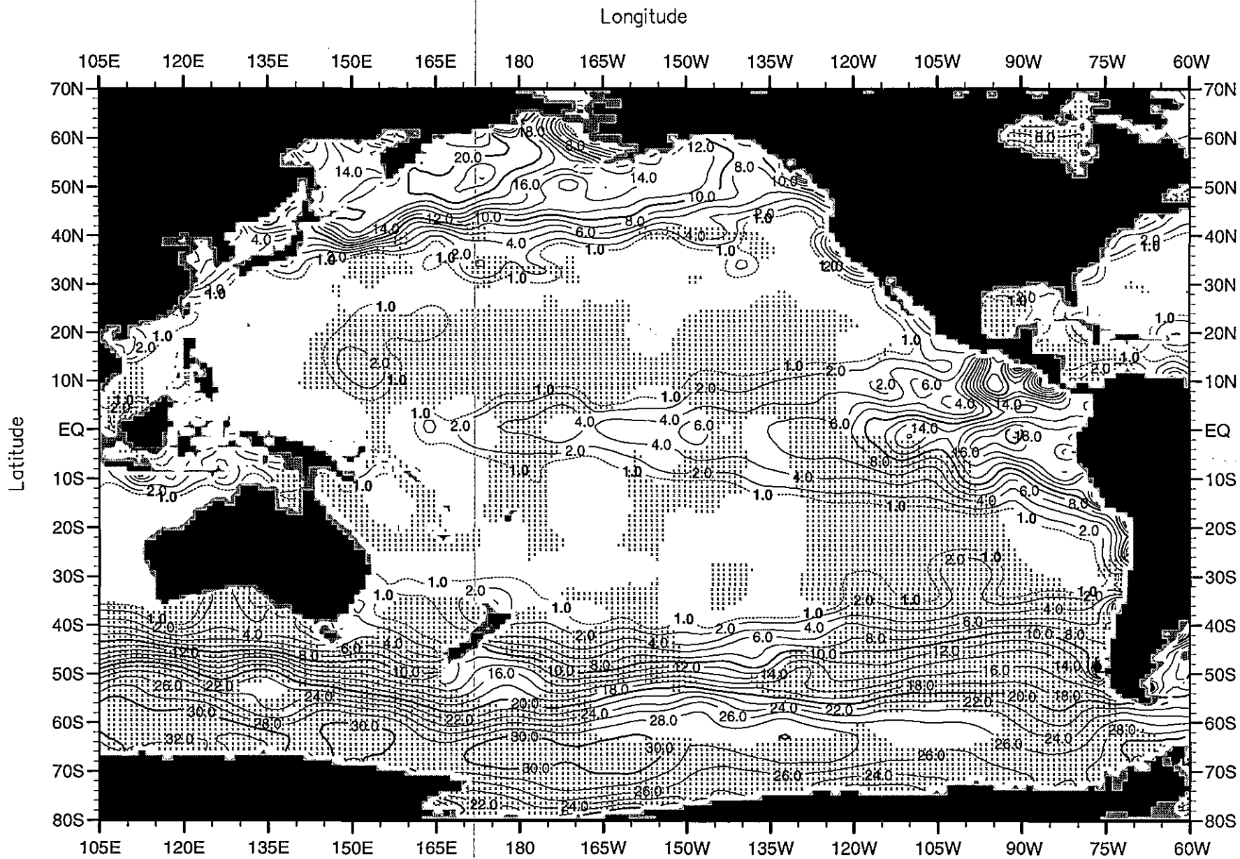
Fig. D38. Summer (Jul.-Sep.) mean nitrate ( \mu\text{M} ) at 50 m. depth .
