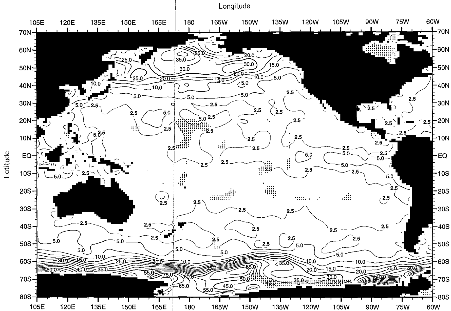
Fig. E17. Annual mean silicate ( \mu\text{M} ) at the surface. Minimum Value= 0.10 Maximum Value= 93.96 Contour Interval: 5.00
