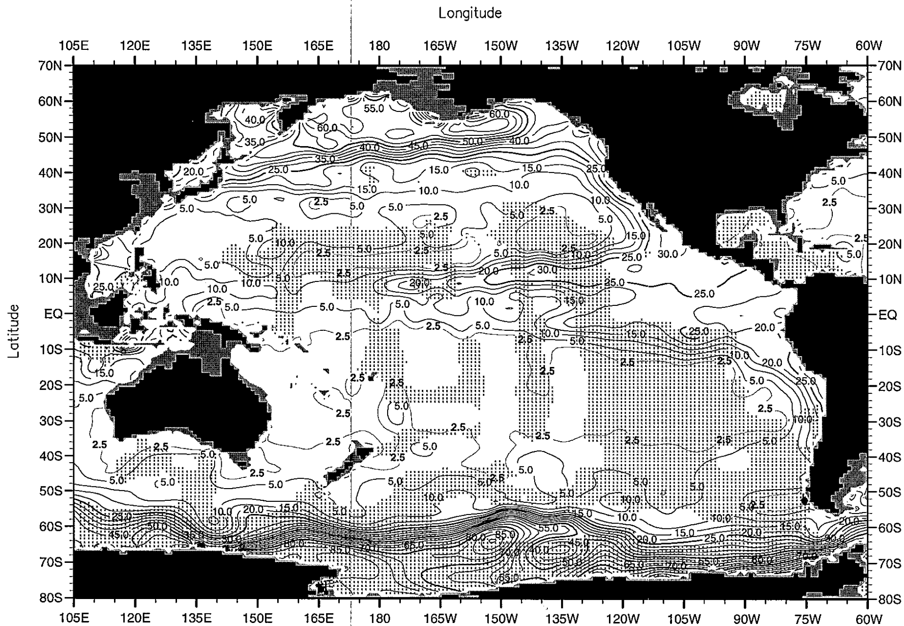
Fig. F41. Summer (Jul.-Sep.) mean silicate ( \mu\text{M} ) at 150 m. depth .
