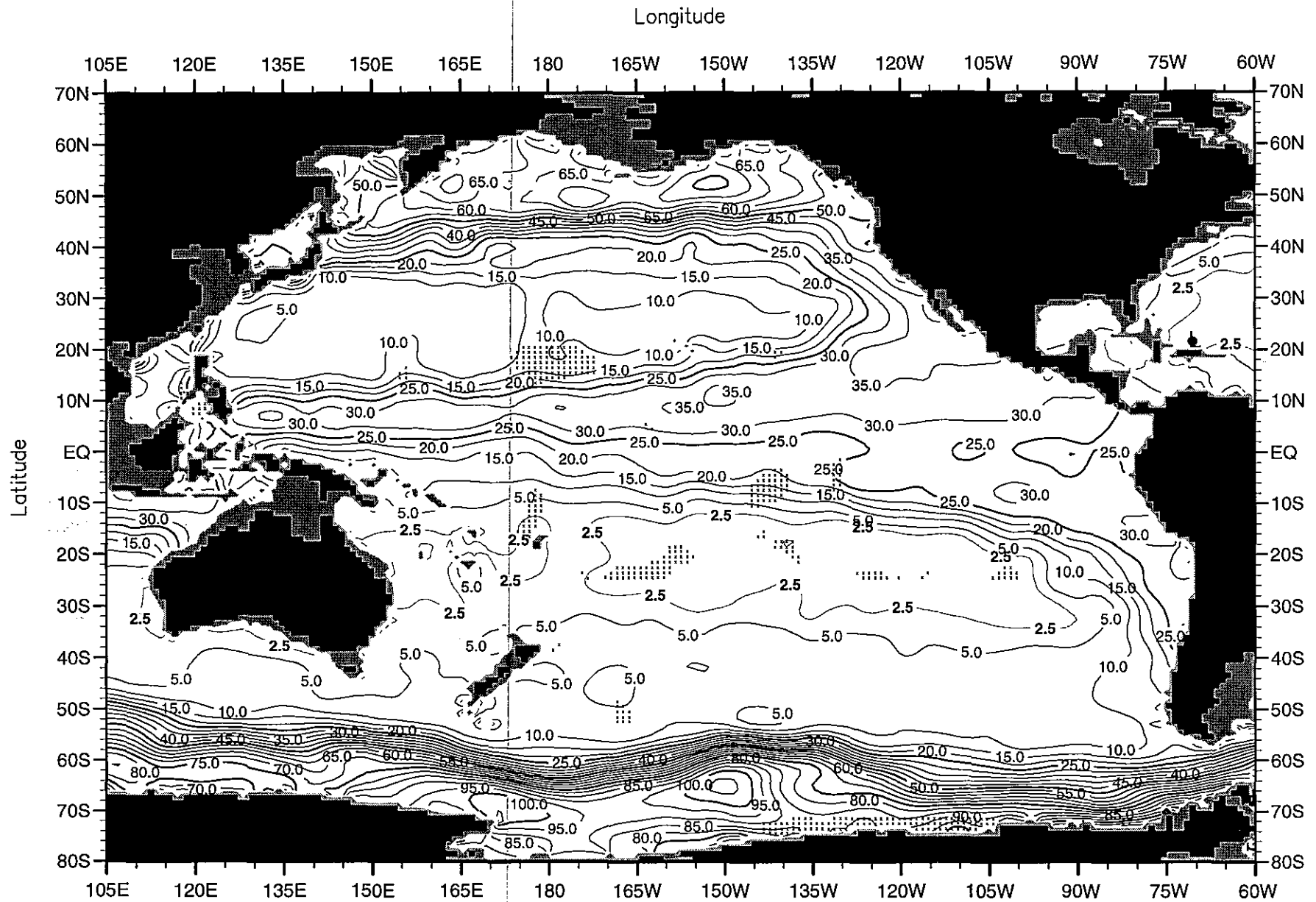
Fig. E23. Annual mean silicate ( \mu\text{M} ) at 250 m. depth .
