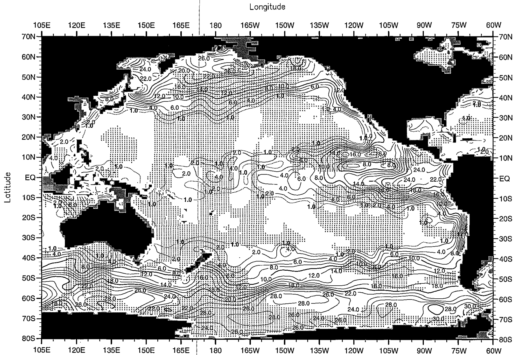
Fig. D45. Fall (Oct.-Dec.) mean nitrate ( \mu\text{M} ) at 75 m. depth.
