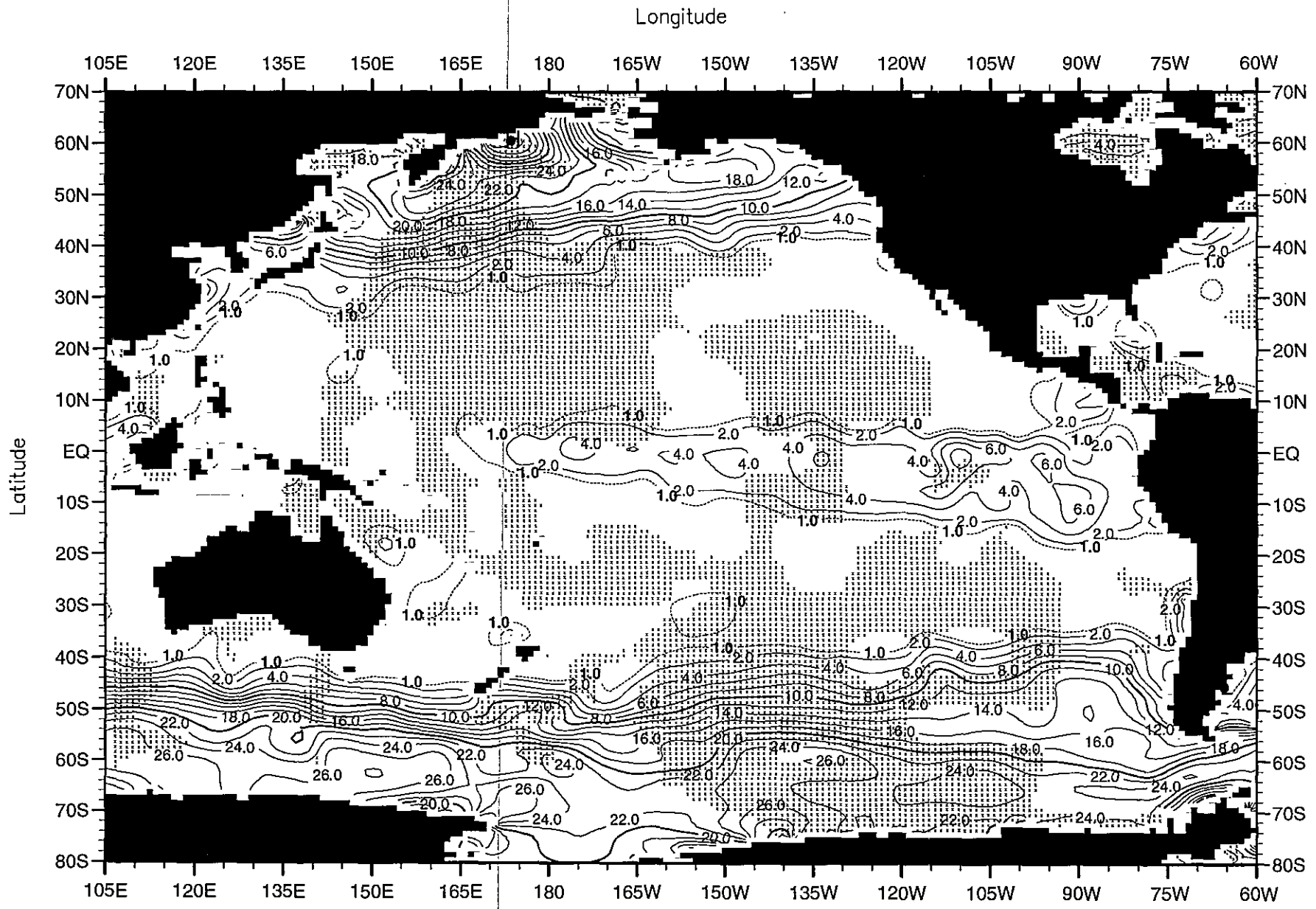
Fig. D25. Winter (Jan.-Mar.) mean nitrate ( \mu\text{M} ) at the surface .
