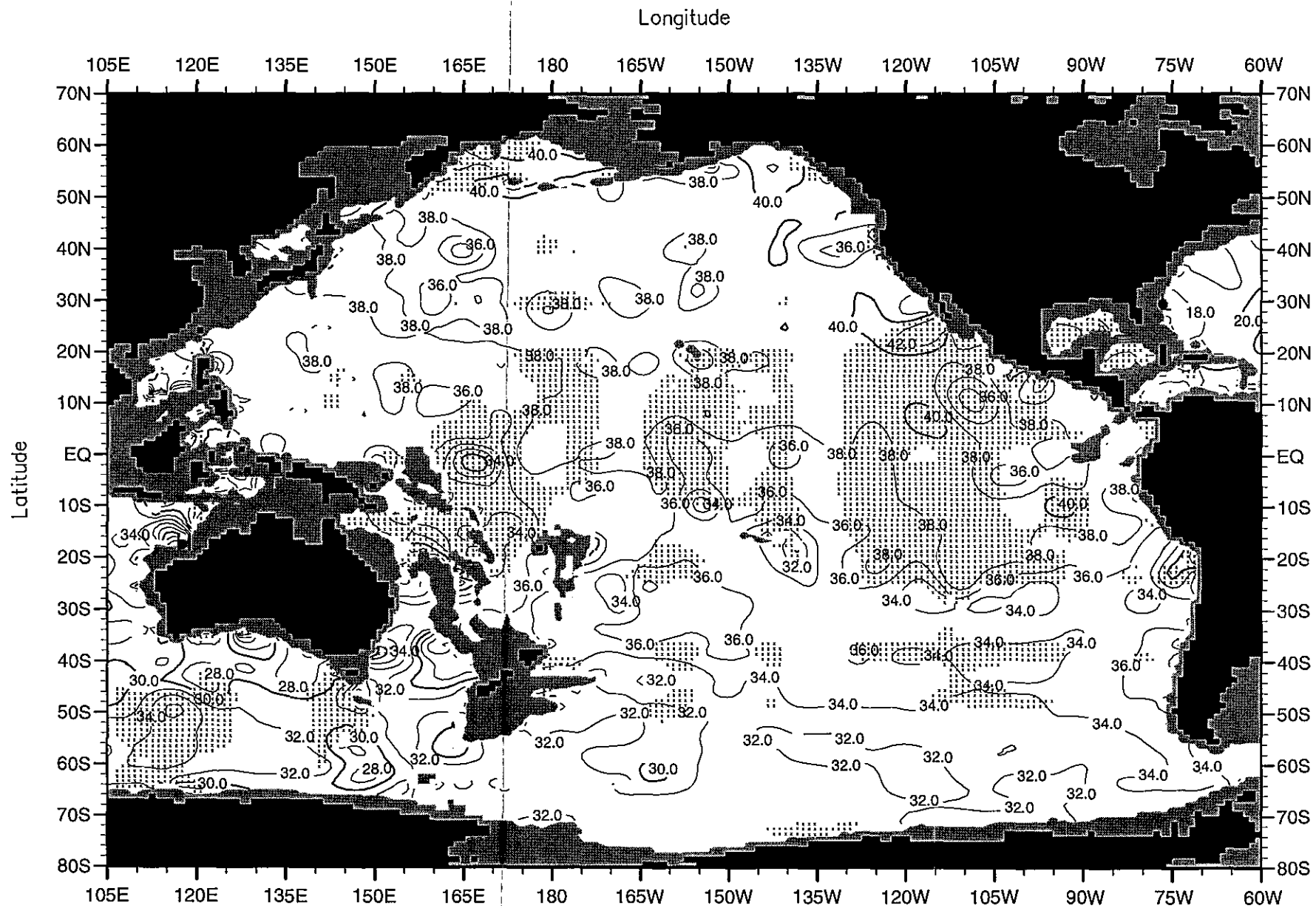
Fig. C31. Annual mean nitrate ( \mu\text{M} ) at 3000 m. depth .
