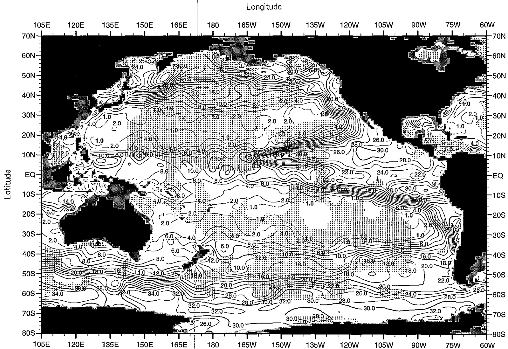
Fig. D29. Winter (Jan.-Mar.) mean nitrate ( \mu\text{M} ) at 150 m. depth .
