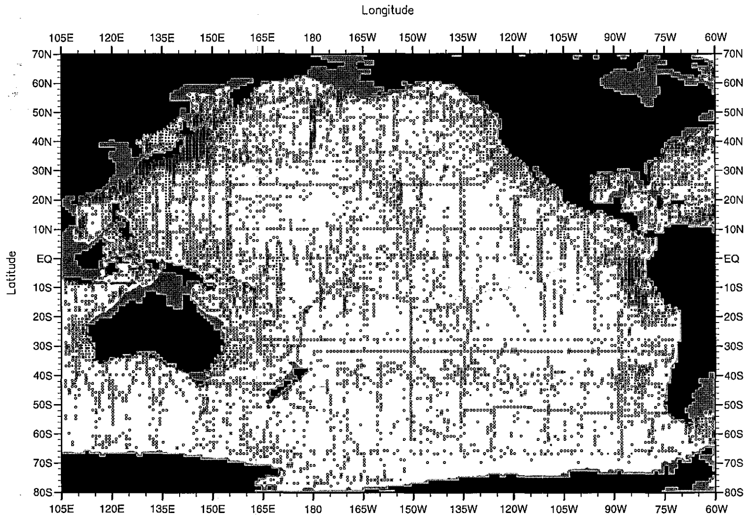
Fig. 1a. Annual phosphate standard deviation ( \mu\text{M} ) at 500 meters depth by one-degree squares.
