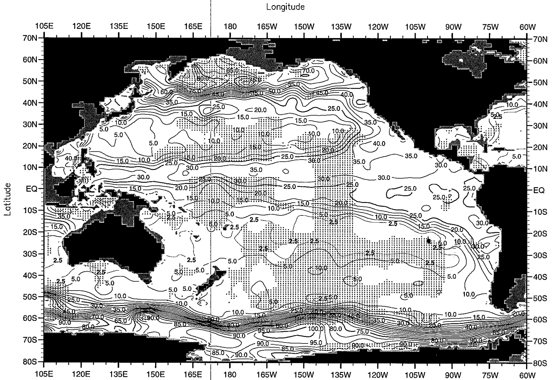
Fig. F30. Winter (Jan.-Mar.) mean silicate ( \mu\text{M} ) at 250 m. depth .
