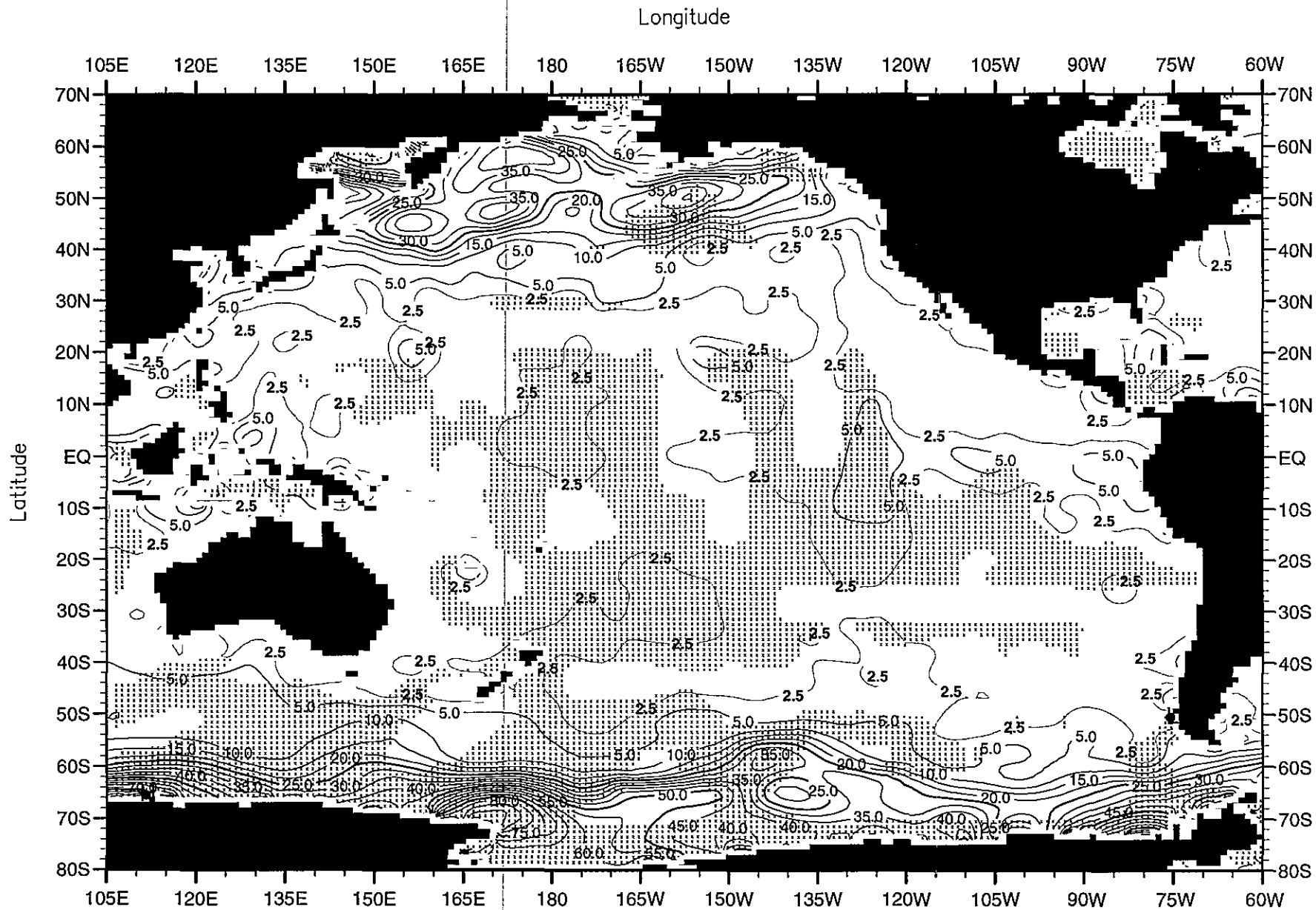
Fig. F31. Spring (Apr.-Jun.) mean silicate ( \mu\text{M} ) at the surface . Minimum Value= 0.00 Maximum Value= 97.46 Contour Interval: 5.00
