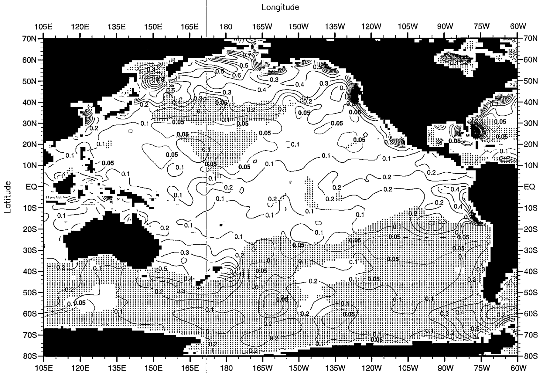
Fig. H7. Summer (Jul.-Sep.) mean chlorophyll ( \mu\text{g/l} ) at the surface .
