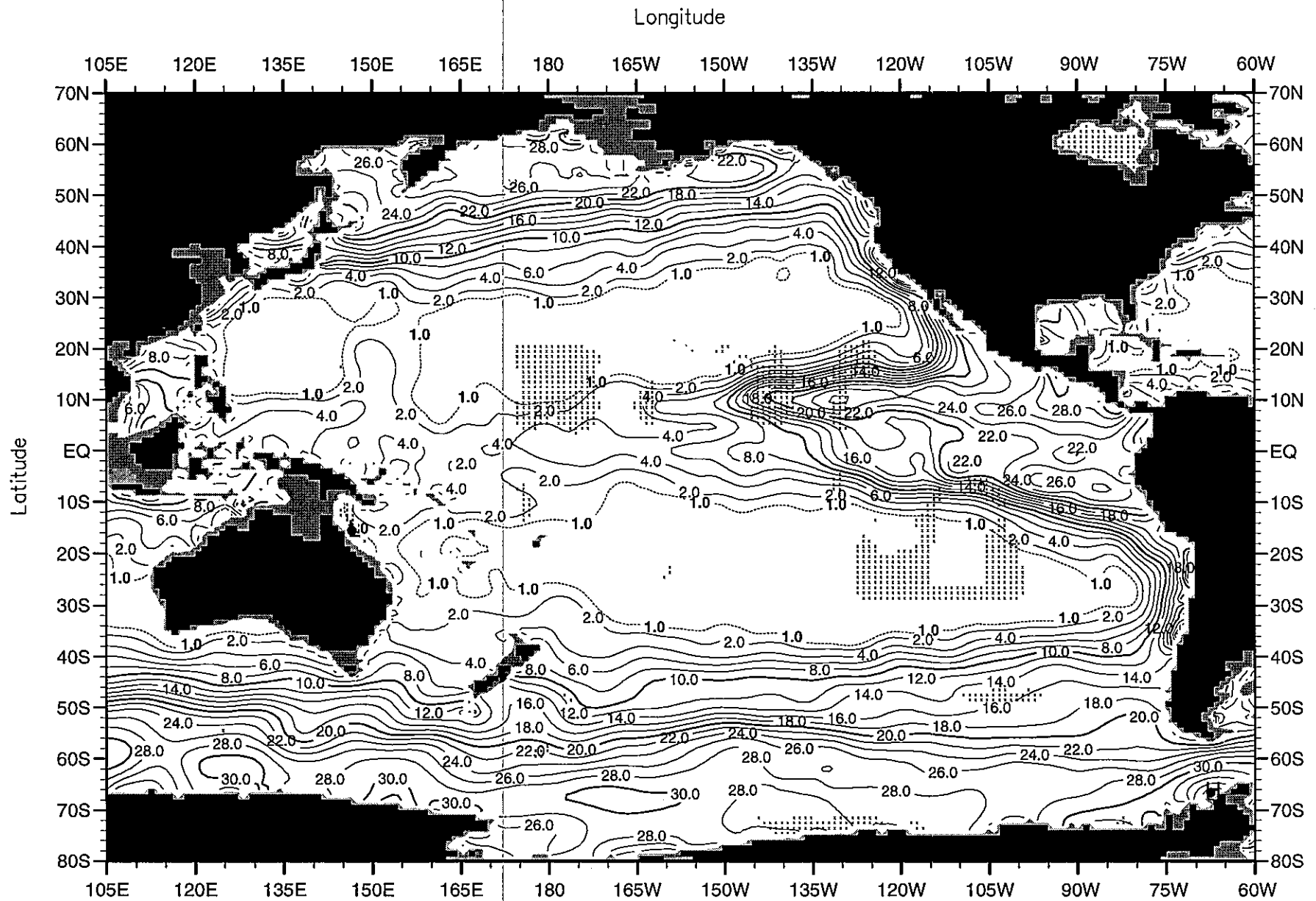
Fig. C20. Annual mean nitrate ( \mu\text{M} ) at 100 m. depth .
