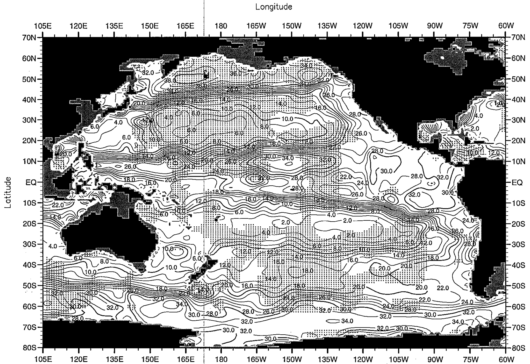
Fig. D30. Winter (Jan.-Mar.) mean nitrate ( \mu\text{M} ) at 250 m. depth .
