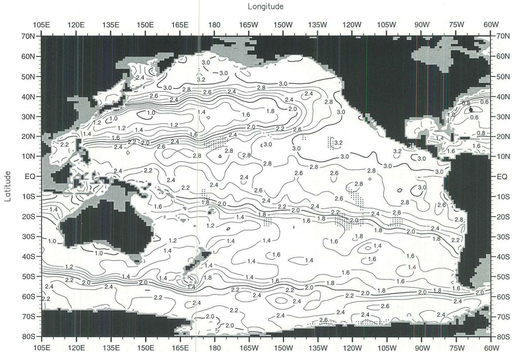
Fig. A25. Annual mean phosphate ( \mu\text{M} ) at 500 m. depth .
