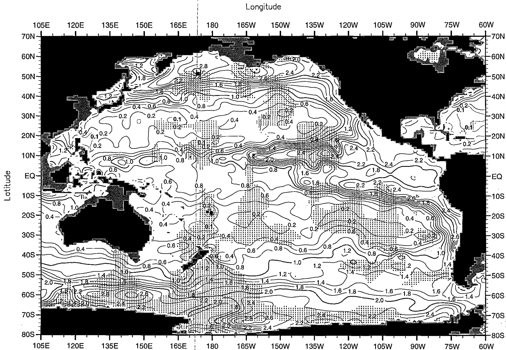
Fig. B47. Fall (Oct.-Dec.) mean phosphate ( \mu\text{M} ) at 150 m. depth .
