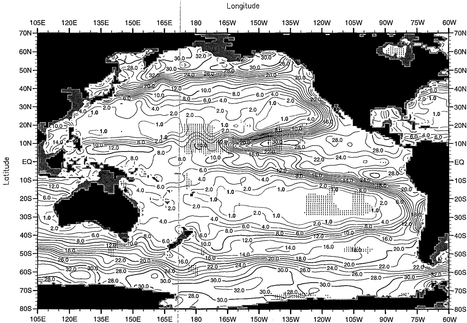
Fig. C21. Annual mean nitrate ( \mu\text{M} ) at 150 m. depth .
