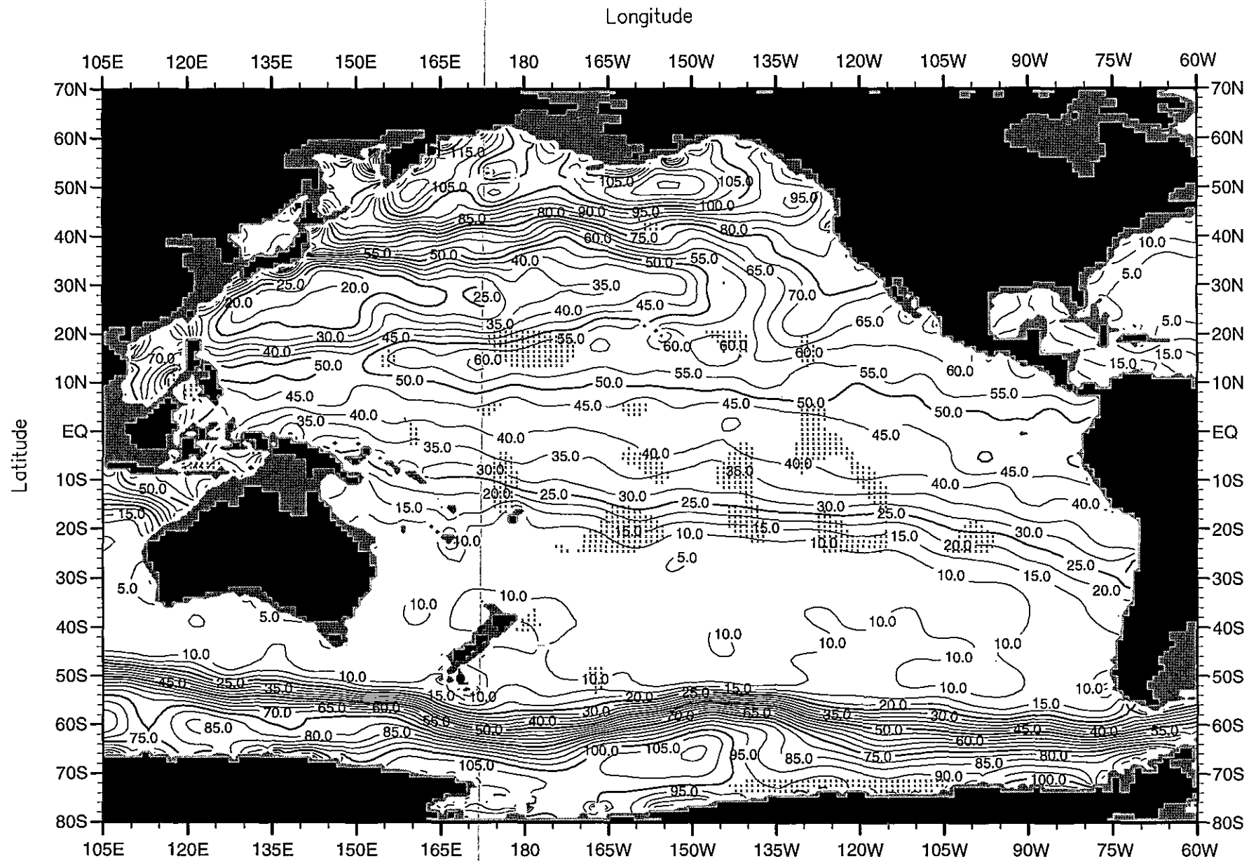
Fig. E25. Annual mean silicate ( \mu\text{M} ) at 500 m. depth .
