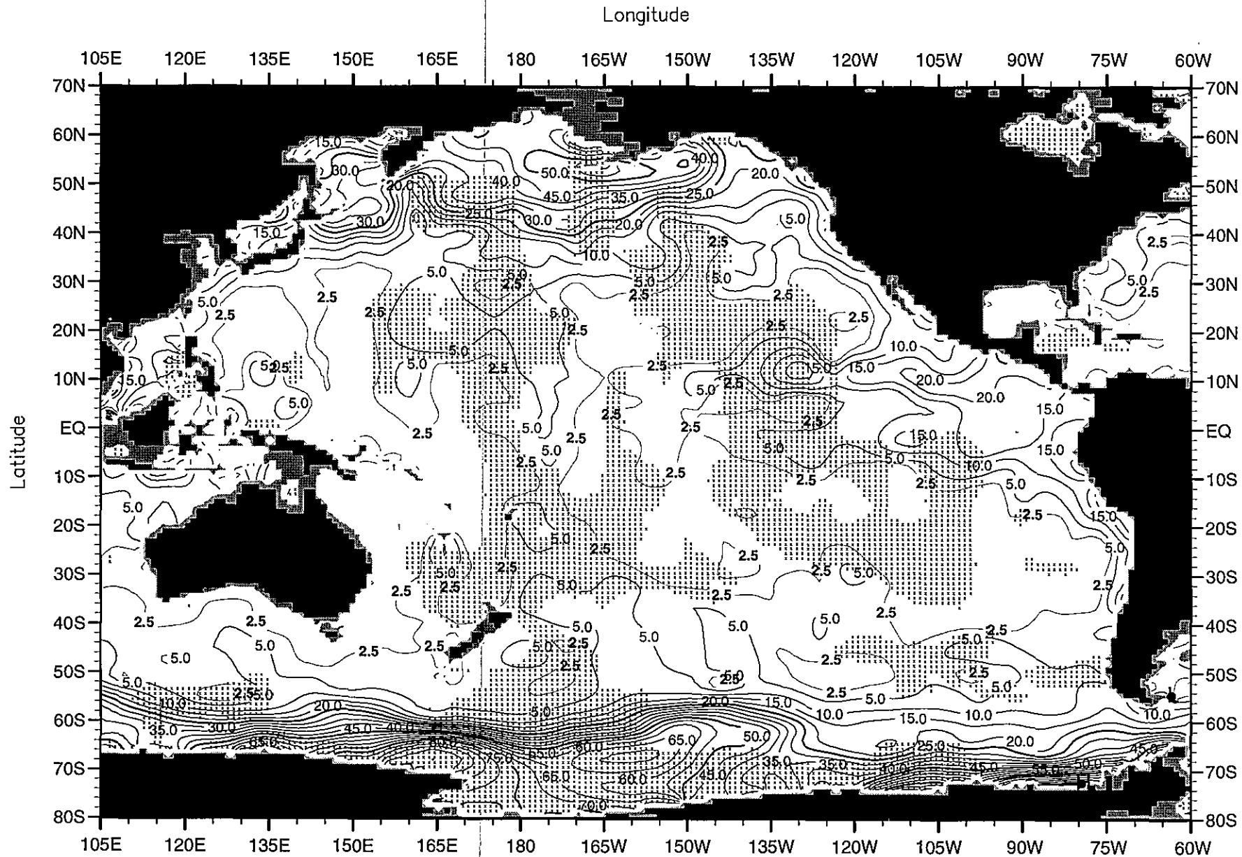
Fig. F45. Fall (Oct.-Dec.) mean silicate ( \mu\text{M} ) at 75 m. depth.
