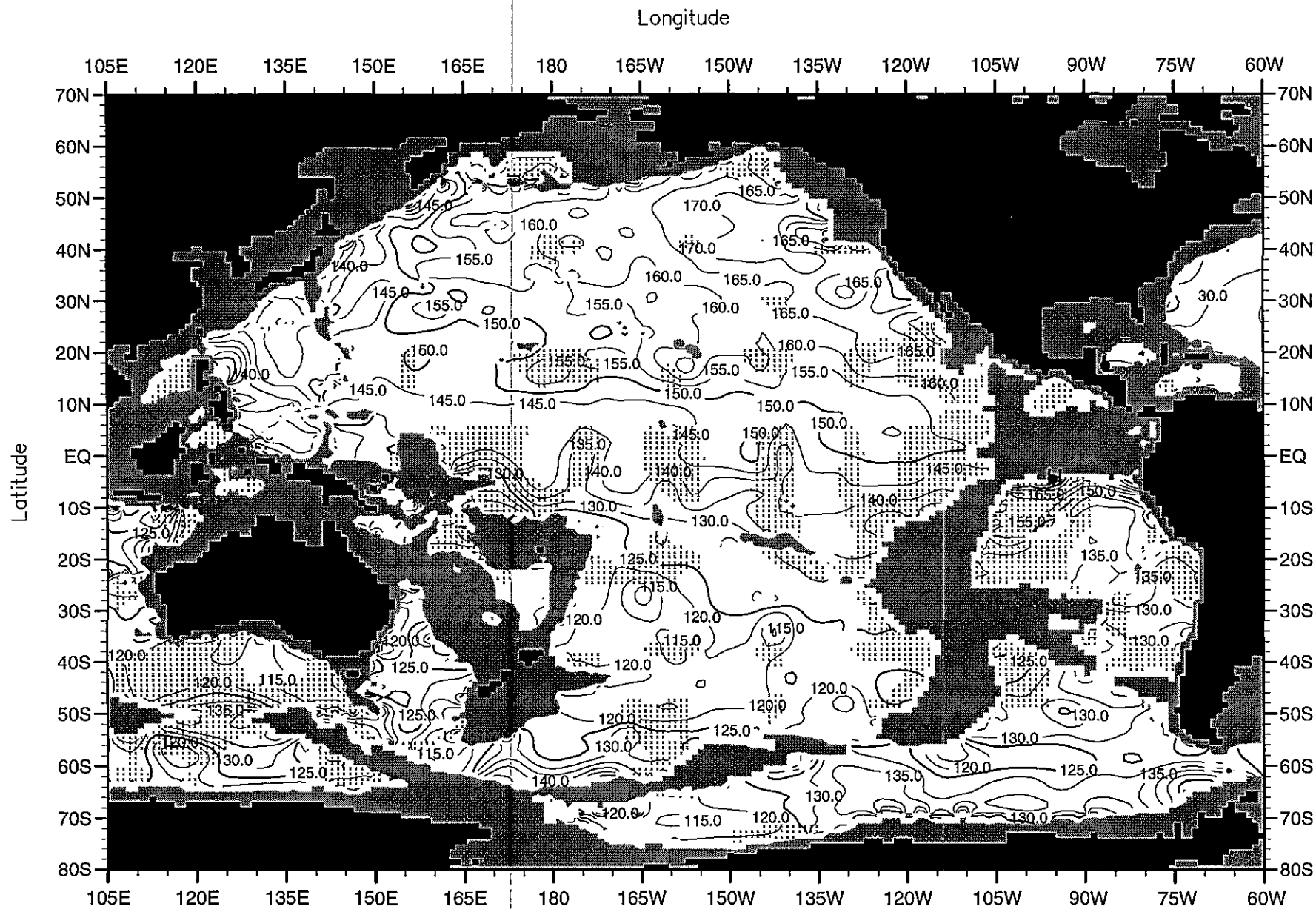
Fig. E32. Annual mean silicate ( \mu\text{M} ) at 4000 m. depth .
