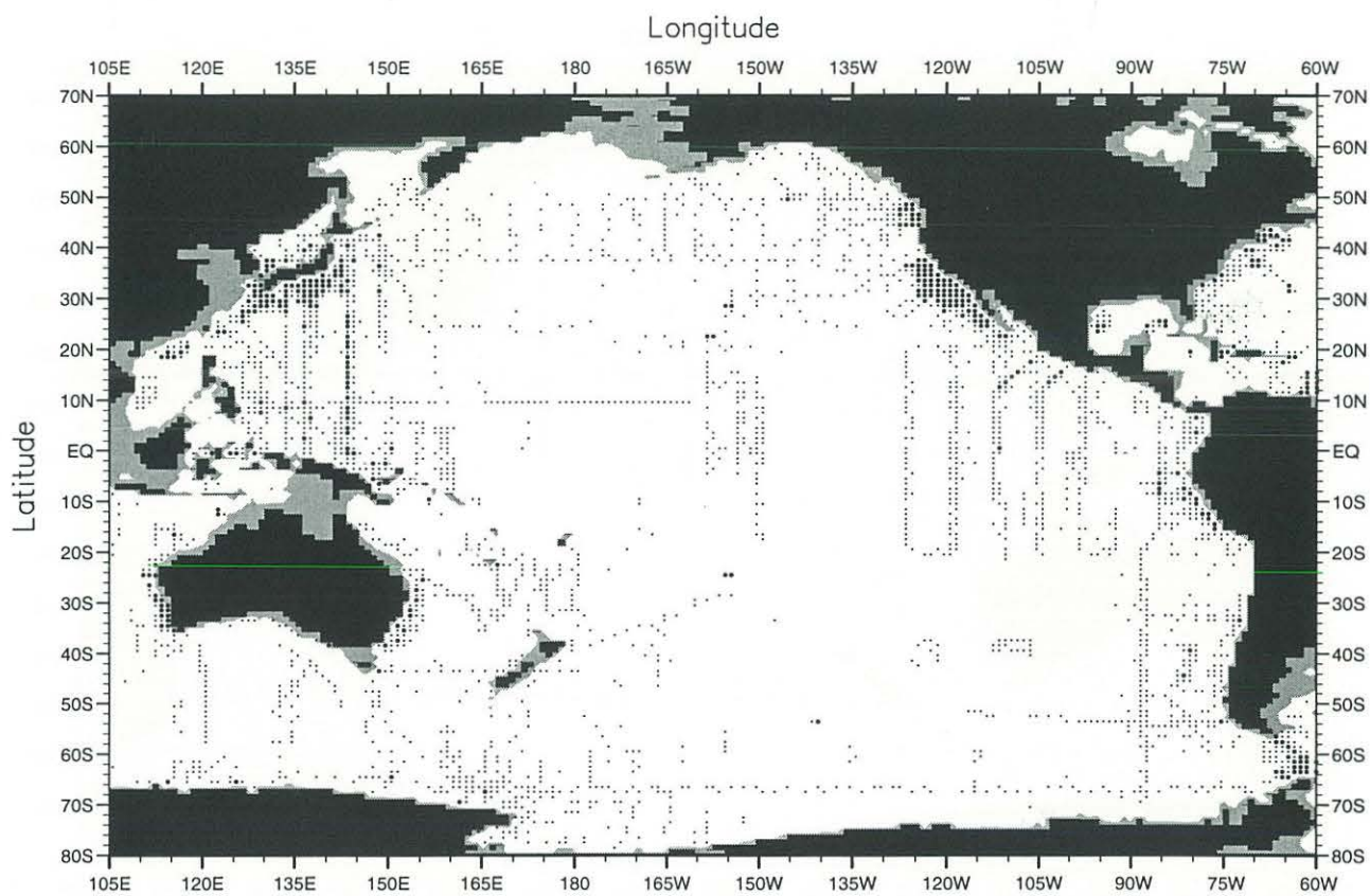
Fig. F5. Winter (Jan.-Mar.) silicate observations at 150 m. depth .
