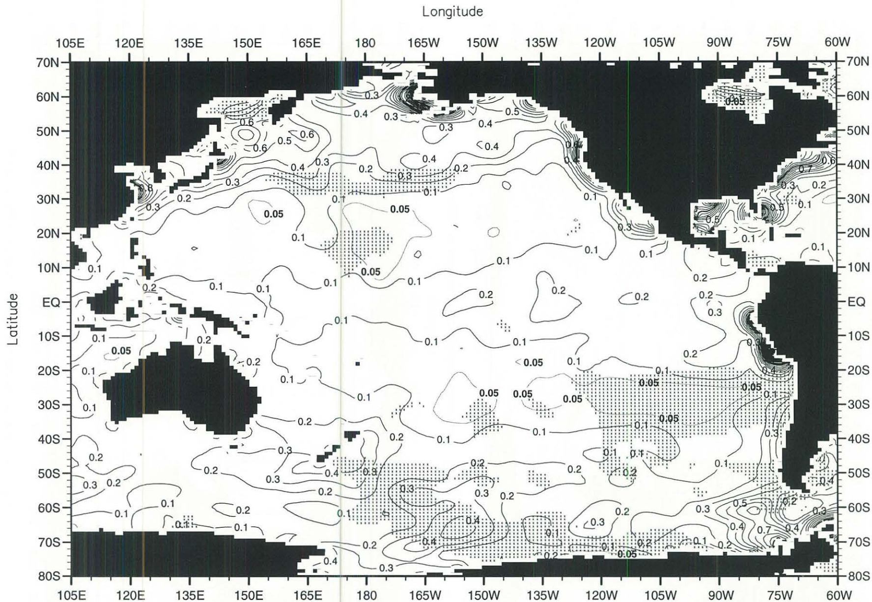
Fig. G7. Annual mean chlorophyll ( \mu\text{g/l} ) at the surface .
