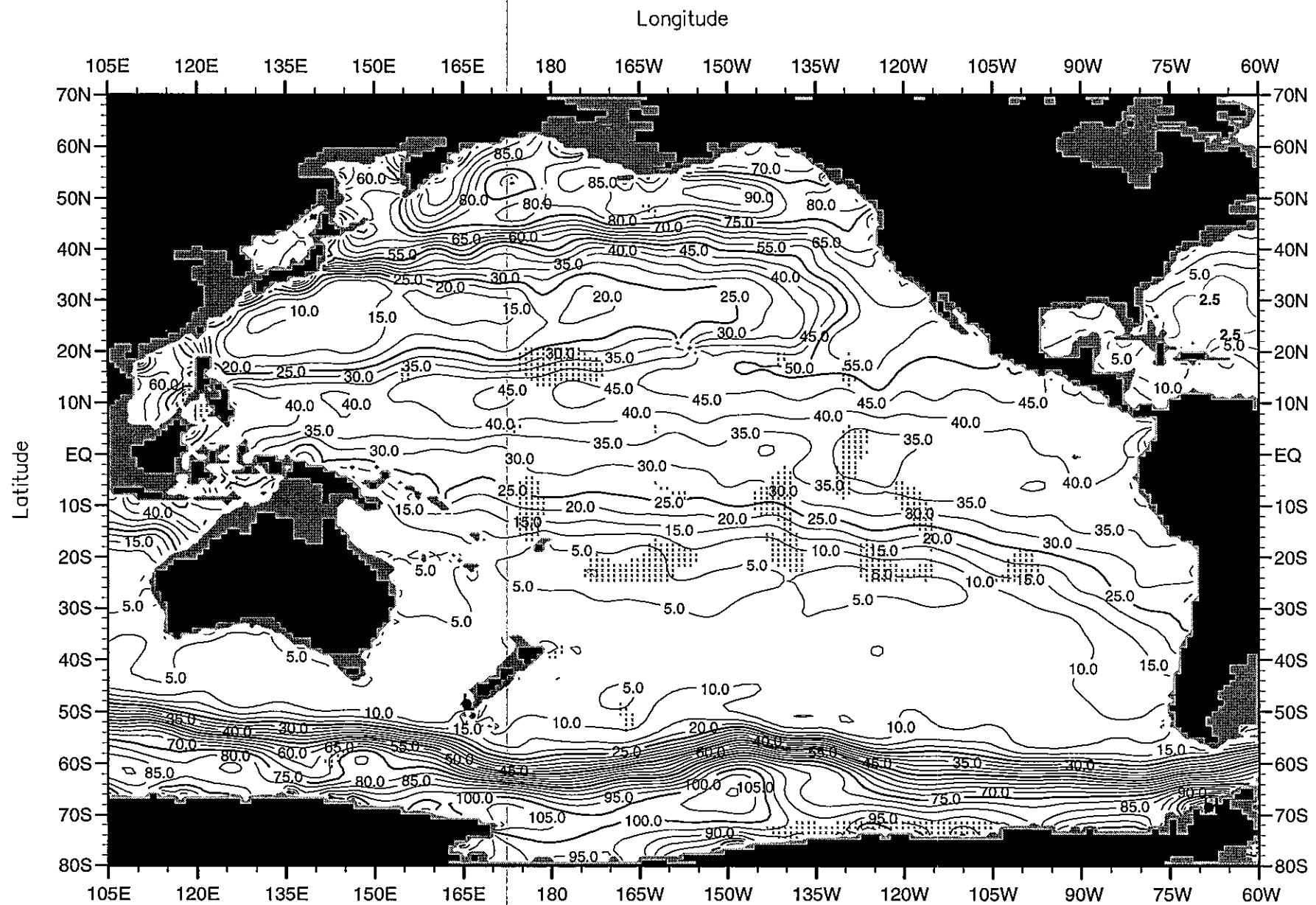
Fig. E24. Annual mean silicate ( \mu\text{M} ) at 400 m. depth .
