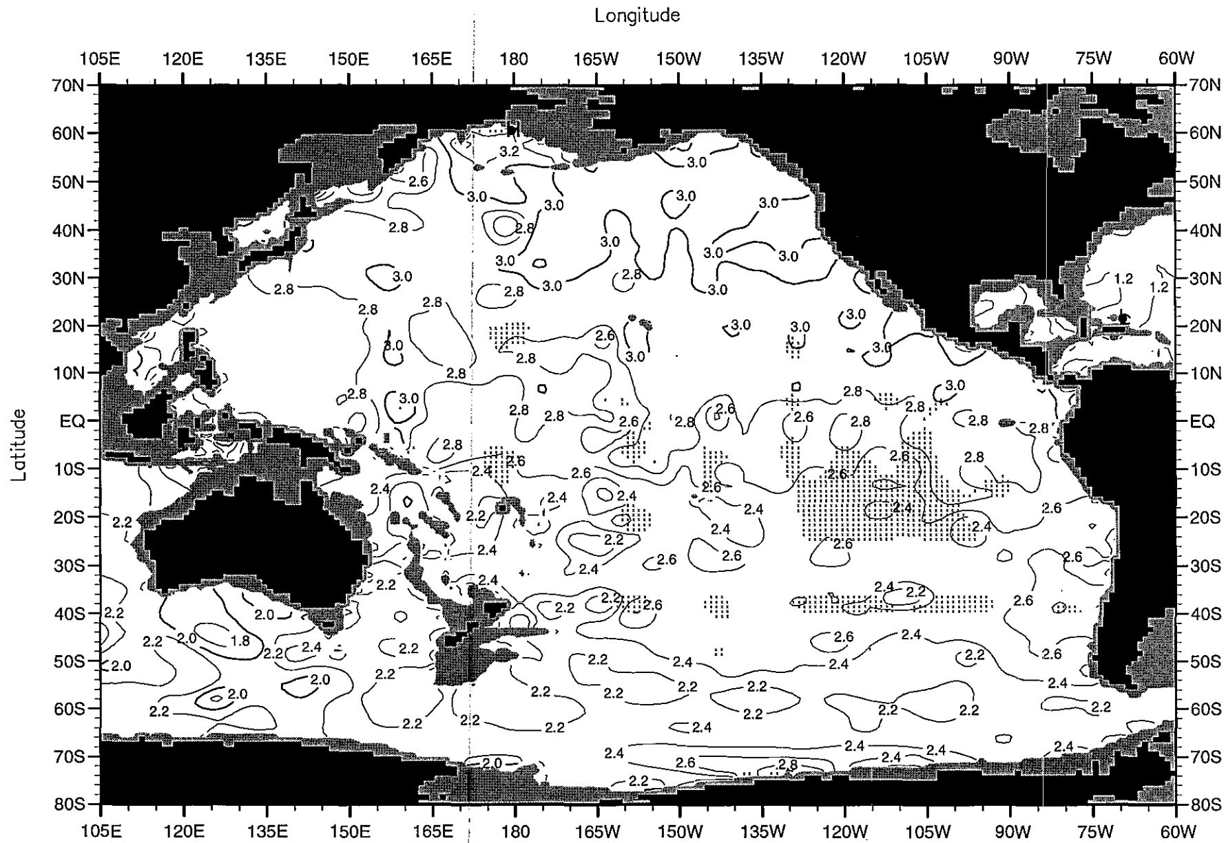
Fig. A29. Annual mean phosphate ( \mu\text{M} ) at 2000 m. depth .
