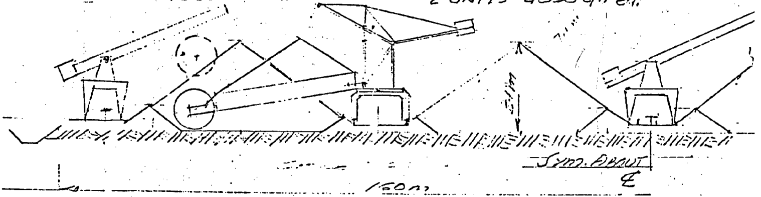
HALF SECTION THRU COAL YARD.
