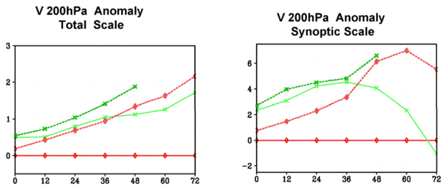
Fig.16. AC with Nature Run for 200mb V. The difference in AC from the CTL (red solid line with \diamond for both T62 and T170) shows the forecast impact of DWL with scanning (x) and non-scanning ( \bullet ). CTL experiments ( \diamond ) include only conventional data. The left panel includes all waves; the right panel includes wave numbers 10-20 only (synoptic scale). Period used is February 13-20. Solid lines are for T62 experiments; dashed lines are for T170 experiments.
