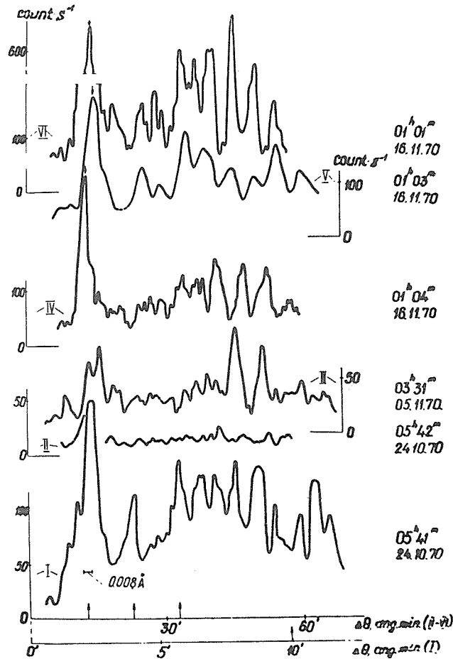
Fig. D2: Spectra in the Region 1.85-1.87 \text{\AA} of 6 solar flares
