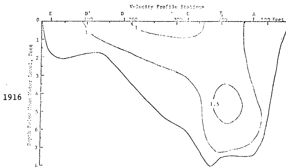
FIGURE 63.--CROSS-CHANNEL FLOOD VELOCITY DISTRIBUTION, 1735 AND 1916 4 MARCH, 1971
