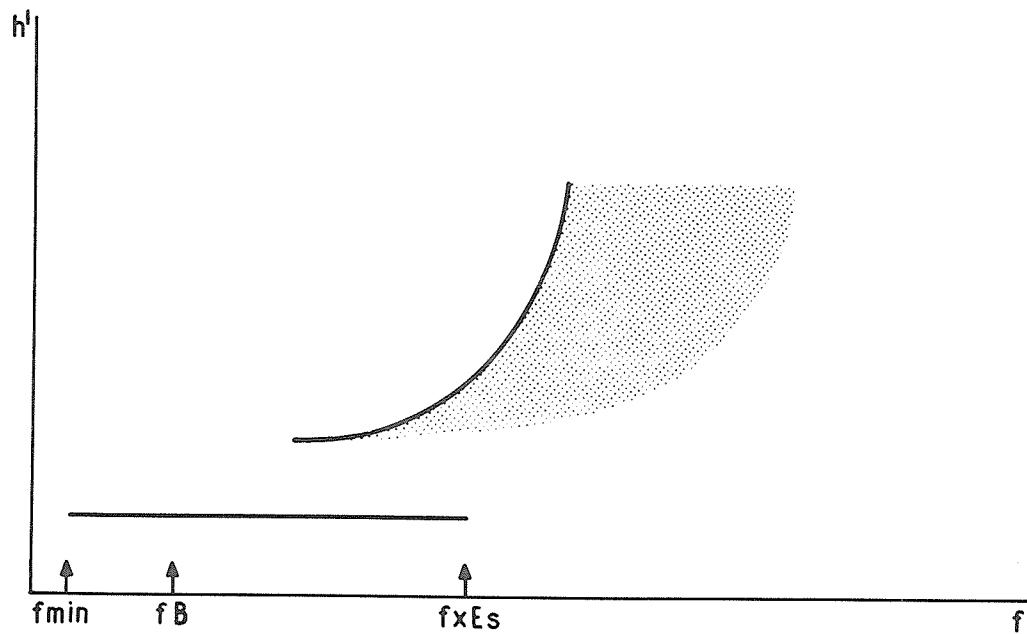
Fig. 4.15 Scatter present
