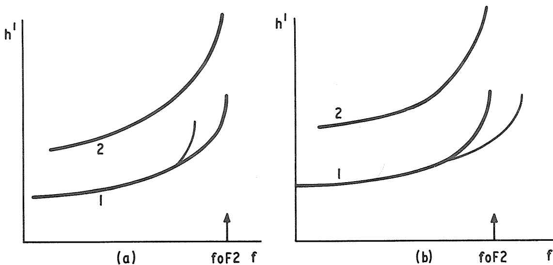
Fig. 2.10 Reflection from a cloud, o mode only
