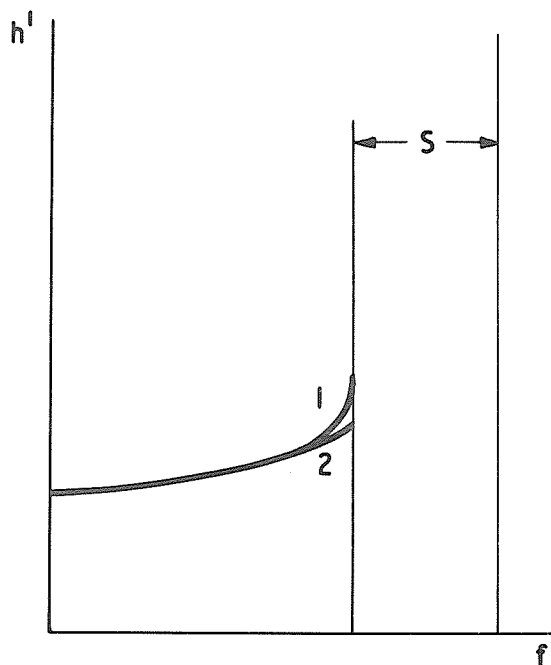
Fig. 3.41 Use of C and S with f_x I
