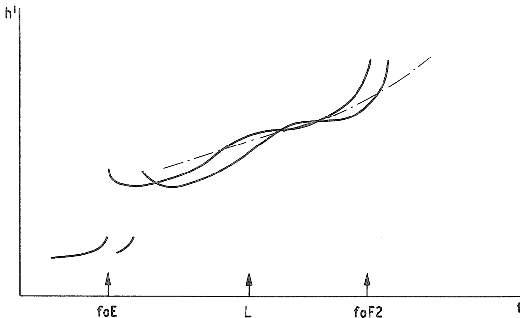
Fig. 3.24 Use of L
