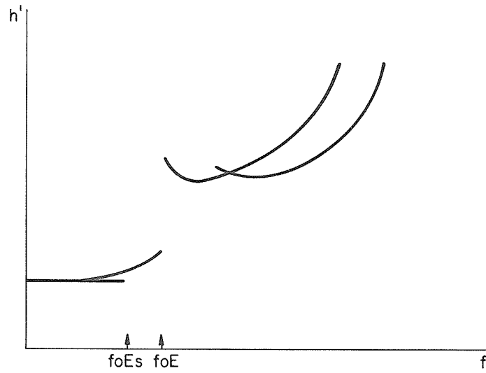
Fig. 3.20 Use of G to show fbEs less than foE foEs is written (foEs)-G
