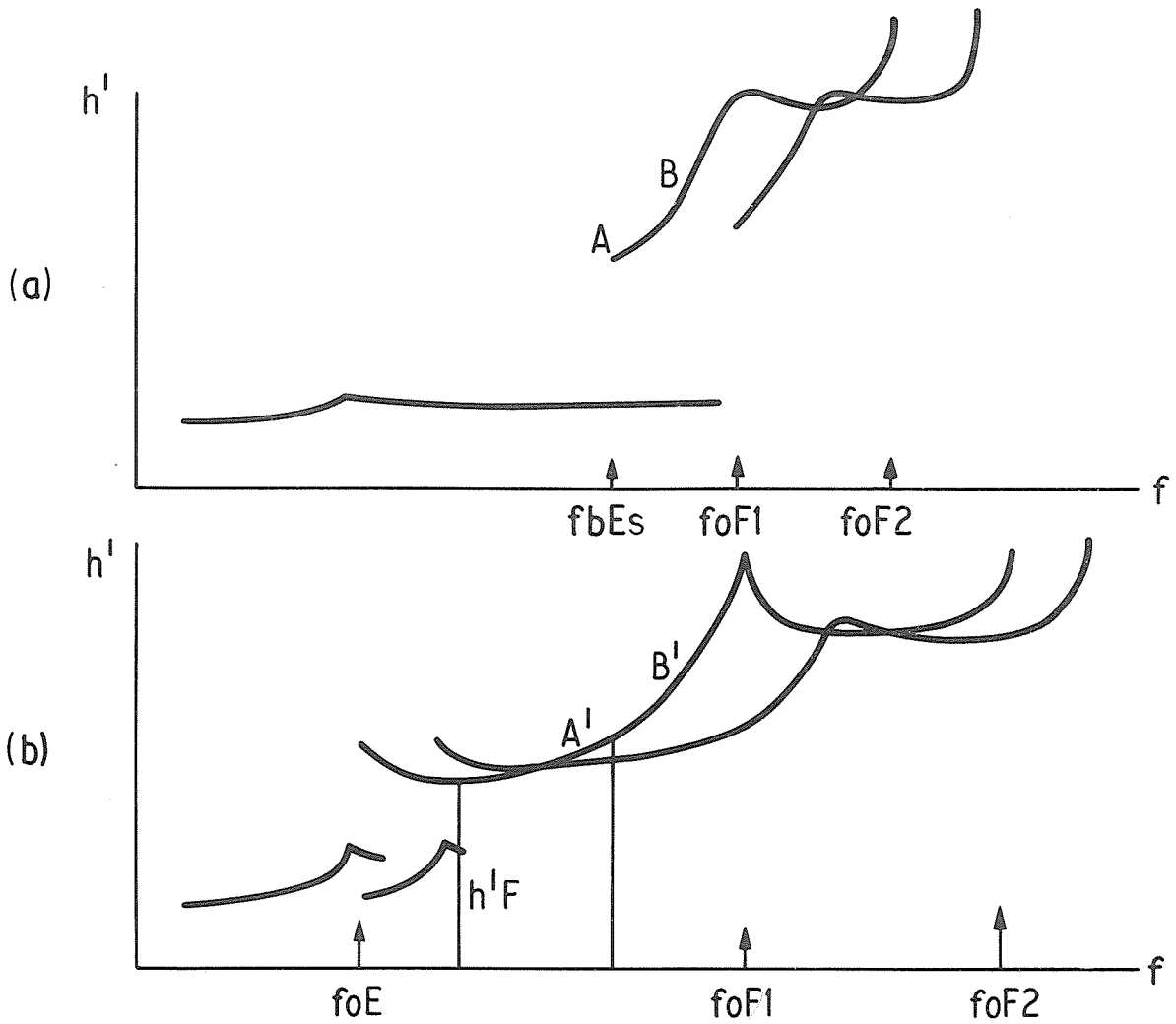
Fig. 2.3 Extrapolation in height
