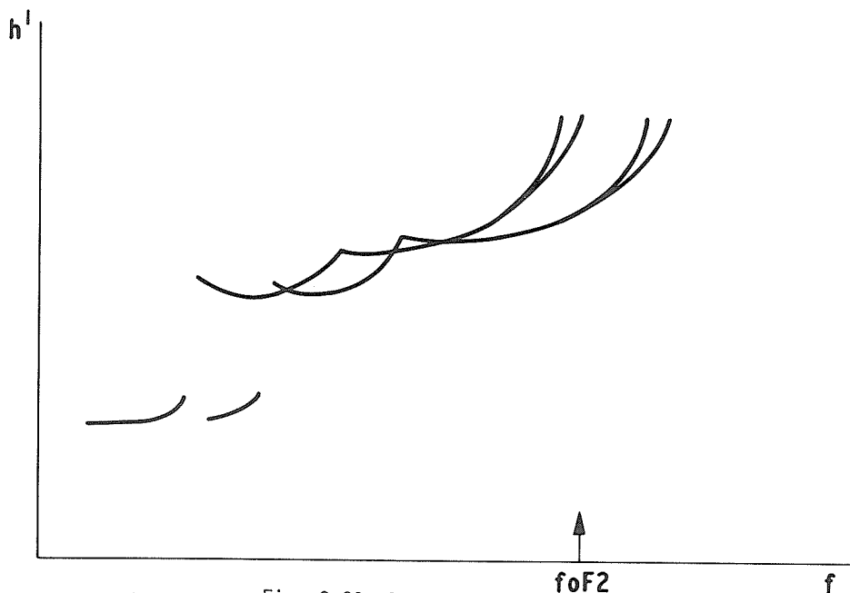
Fig. 3.29 Forked Trace
