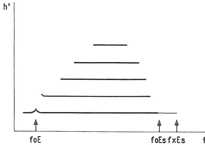
Fig. 3.1 Complete blanketing
