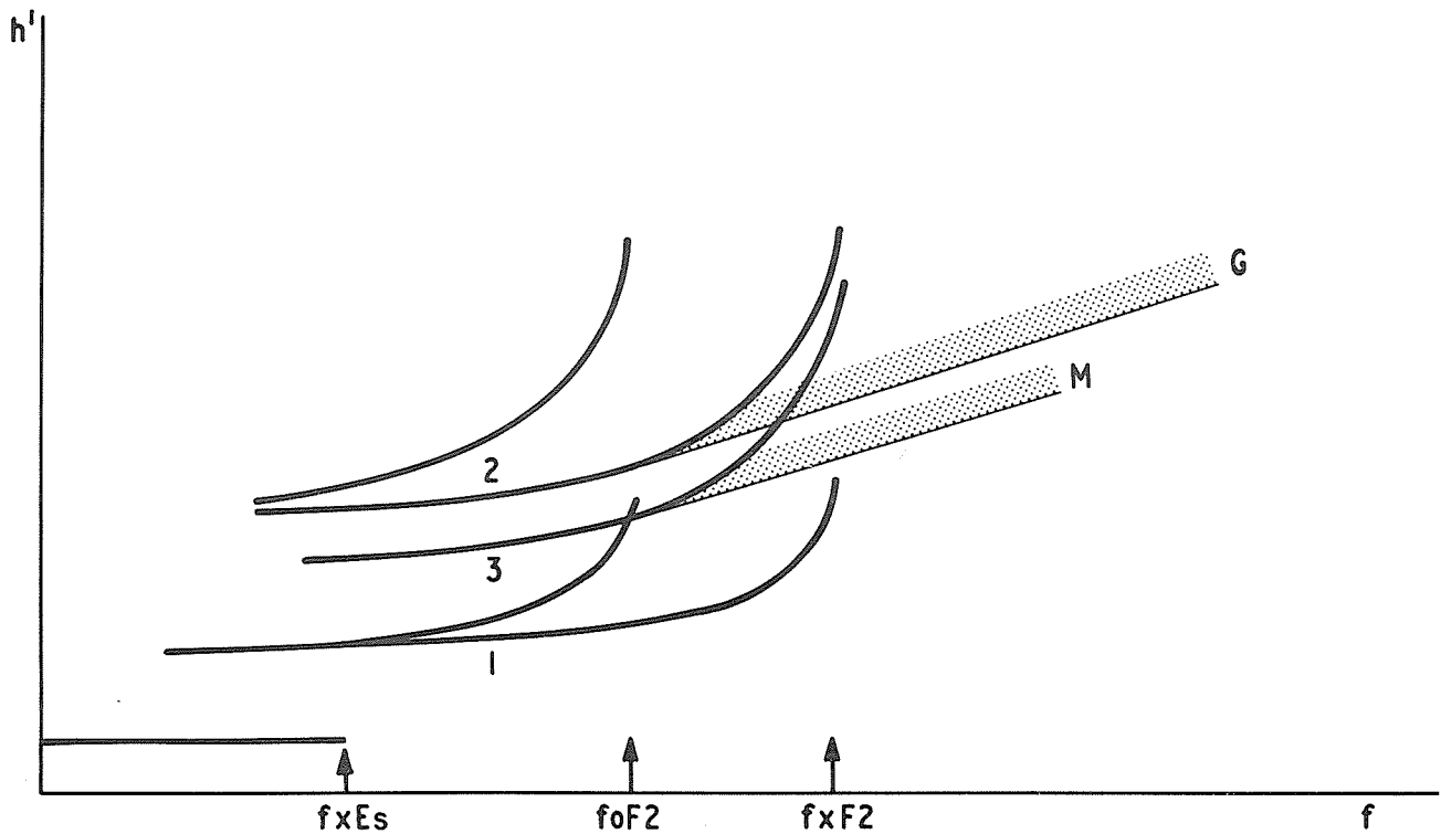
Fig. 3.38 Ground backscatter
