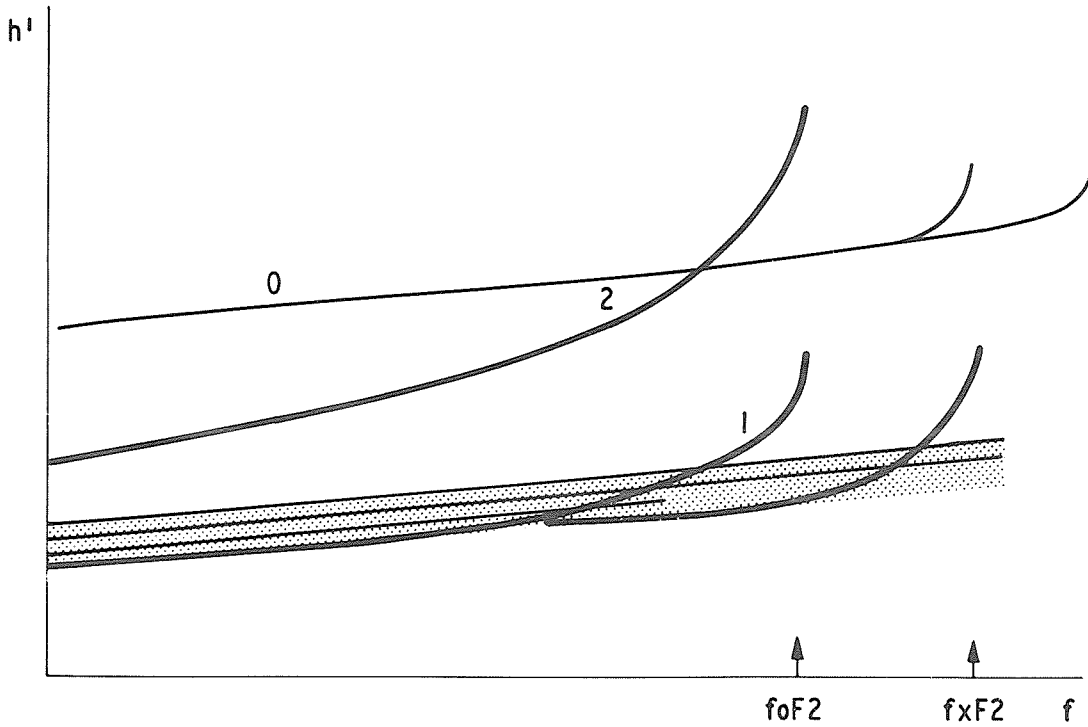
Fig. 2.15 Range spreading
