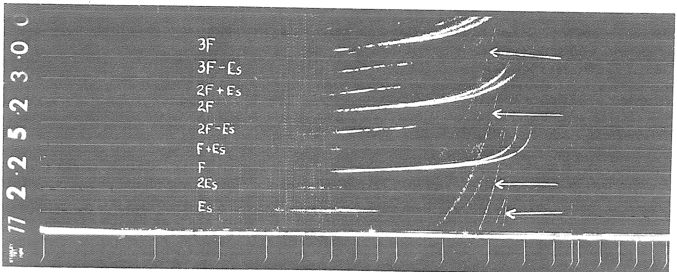
Fig. 1.9(b) Ionogram showing very high order F region reflections, also multiple reflections. Arrows indicate 'round-the-time-base' traces.
