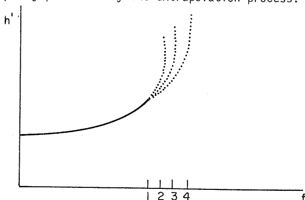
Fig. 2.2b Range of uncertainty when extrapolating to a critical frequency
