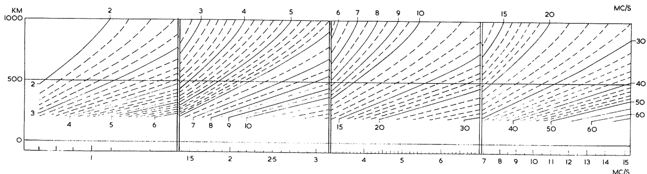
Fig. 1.15 Typical overlay for finding MUF's and MUF factors for ionograms with non-logarithmic frequency scales.
