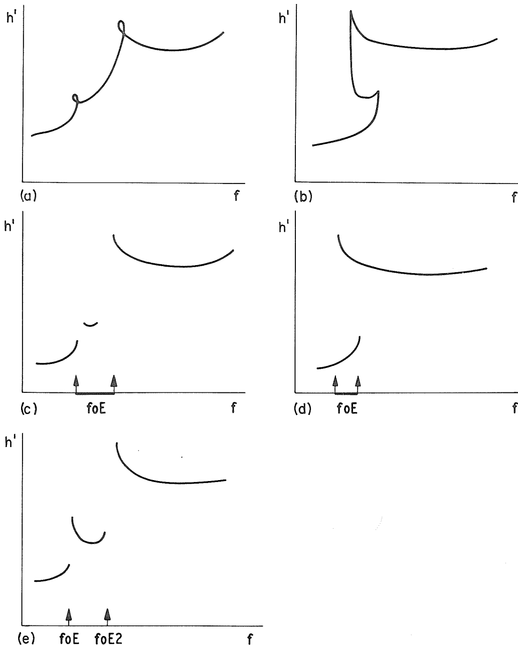
Fig. 2.14 Distinction between effects of layer tilt and intermediate thick E layer (a)(b) The critical forms of o- or x-mode traces when tilts are present near hmE . (c)(d) Traces after allowing for focus phenomena. (e) Thick E2 layer.
