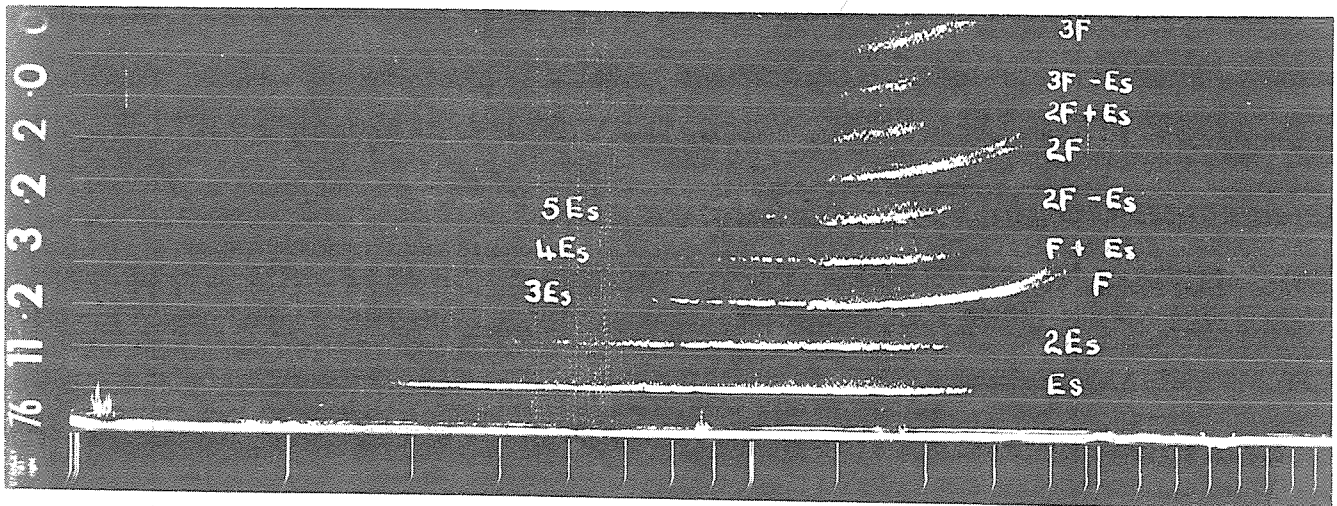
Fig. 1.9(d) Ionogram showing multiple reflections. Note 3E_s is superposed on 1F as is 4E_s on (F + E_s) .
