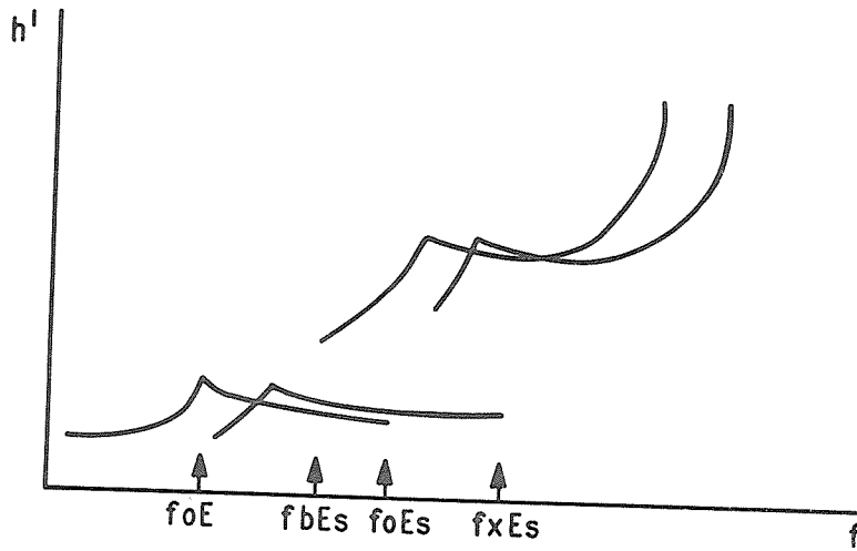
Fig. 3.3 Partial Blanketing
