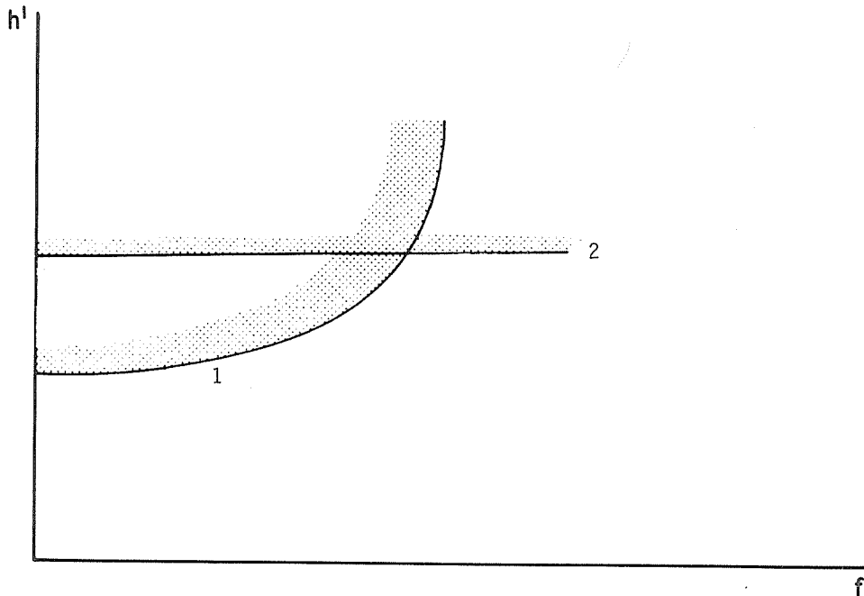
Fig. 2.18 Traces reflected in mode 1 (parallel to field) and mode 2 (perpendicular to field) in Fig. 2.15.
