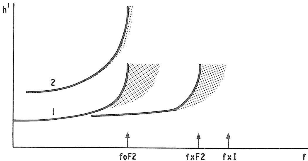
Fig. 2.11 Frequency spread
