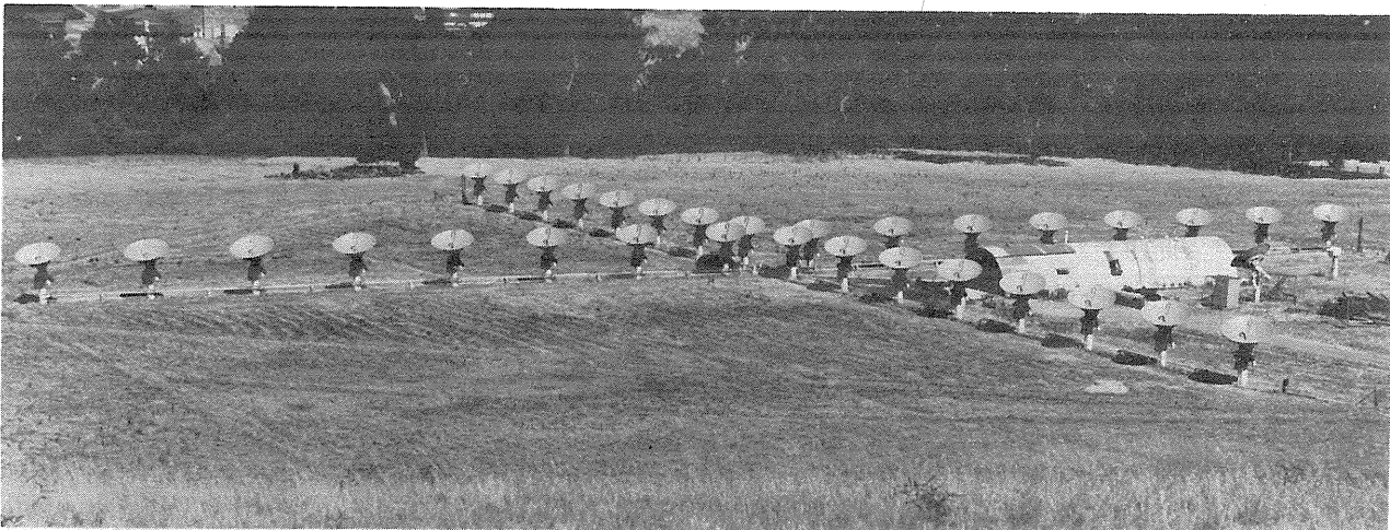
FIG. 1. The Stanford 9.1 cm microwave spectroheliograph in 1958.
