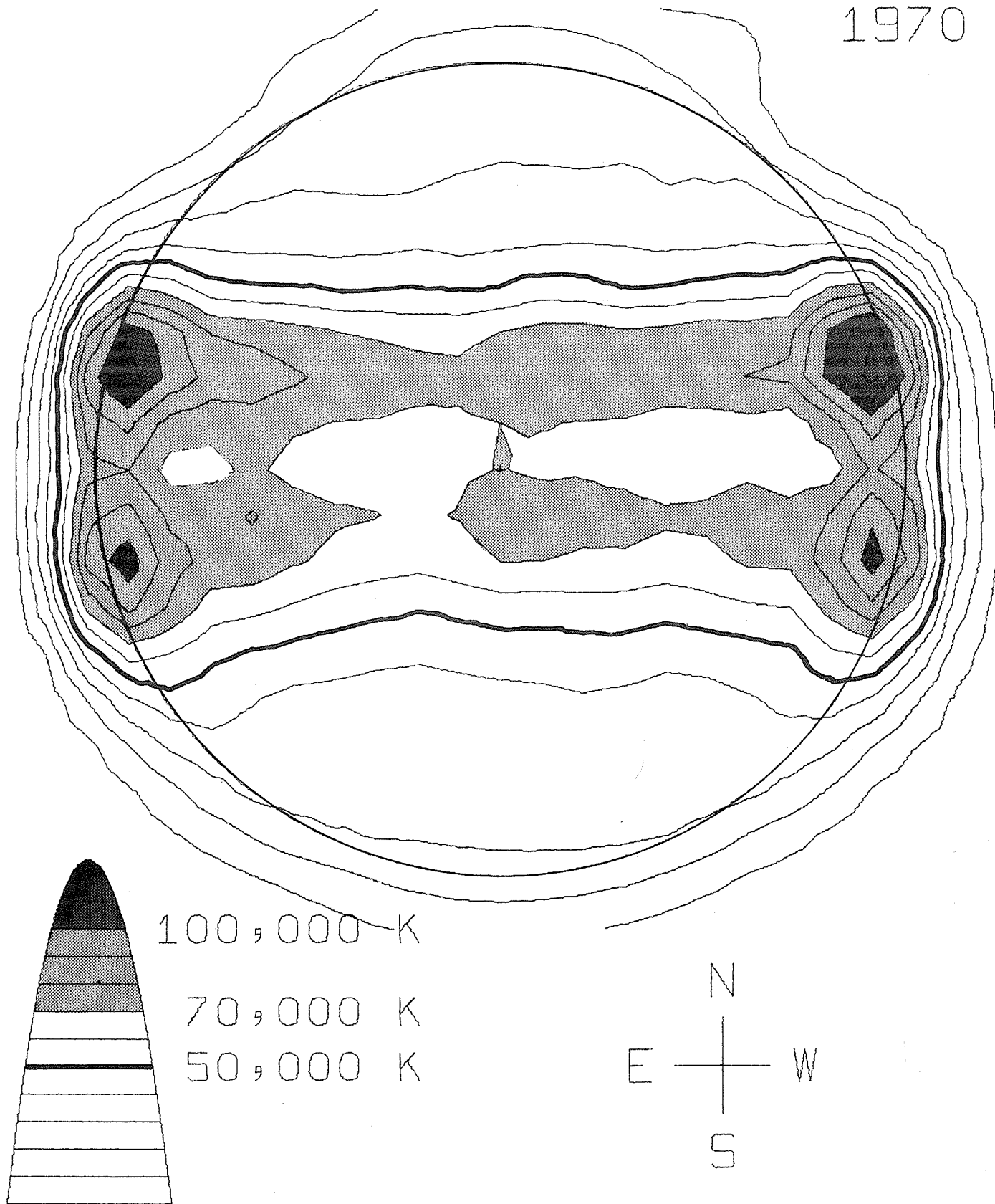
FIG. 5 z . Yearly average map for 1970.
