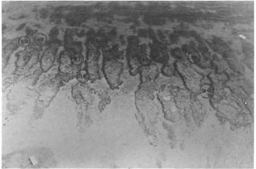
Figure 1.—Aerial view of Looe Key Reef forereef showing approximate areas included in representative, randomly selected, stationary samples.
