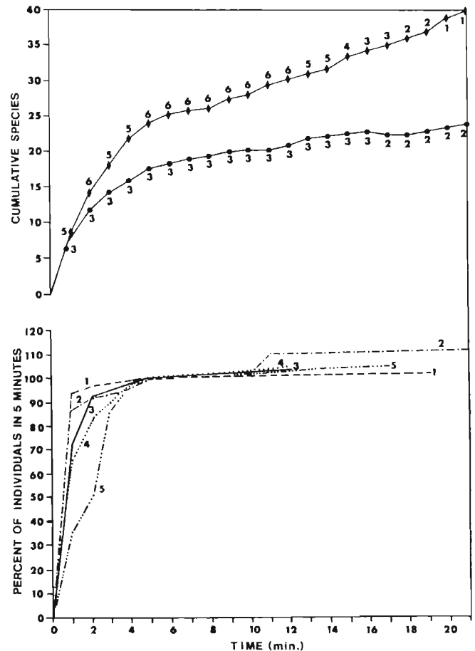
Figure 5.—Effects of sampling time on cumulative observed species and individuals at randomly selected forereef sites. (Top) Cumulative species observed over time from one spot. Numbers show sample size. (Bottom) Percent of individuals represented by species counted per minute during five censuses. Data were standardized by having 100% equal the number of individuals observed in 5 min. 100% represents 640, 381, 172, 235, and 135 individuals for each numbered sample, respectively.
