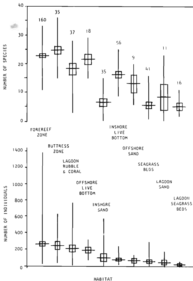
Figure 4.—Mean numbers of species (top) and individuals (bottom) censused per sample in various habitats of Looe Key National Marine Sanctuary. Boxes show 95% confidence limits, vertical lines show ranges, and numbers indicate the number of samples in each habitat. Subjective rankings of habitat complexity from most to least complex were: forereef, buttress, live bottom, lagoon rubble and coral, seagrass beds, and sand flats. Bohnsack et al. (in press) provides more detailed descriptions of sampled habitats.
