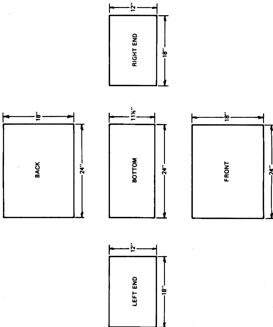
LAYOUT DIAGRAM FOR AQUARIUM CONSTRUCTION Figure 1
